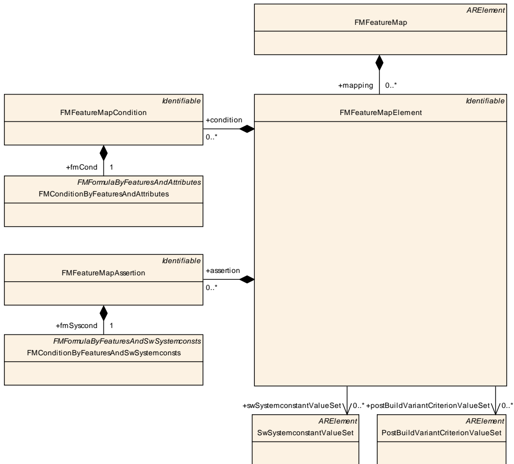
Figure 6.1: Class FMFeatureMap
