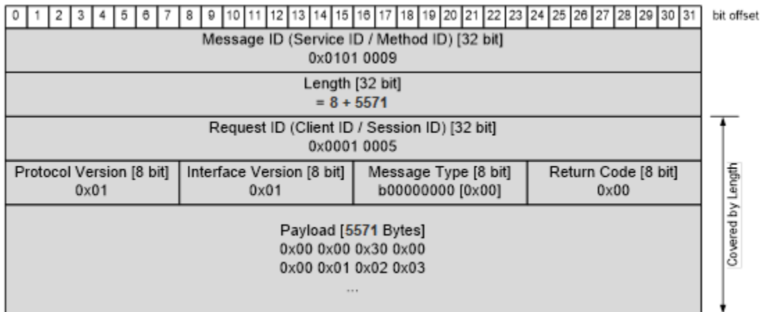
Figure 5 – Example: Header of Original SOME/IP message
