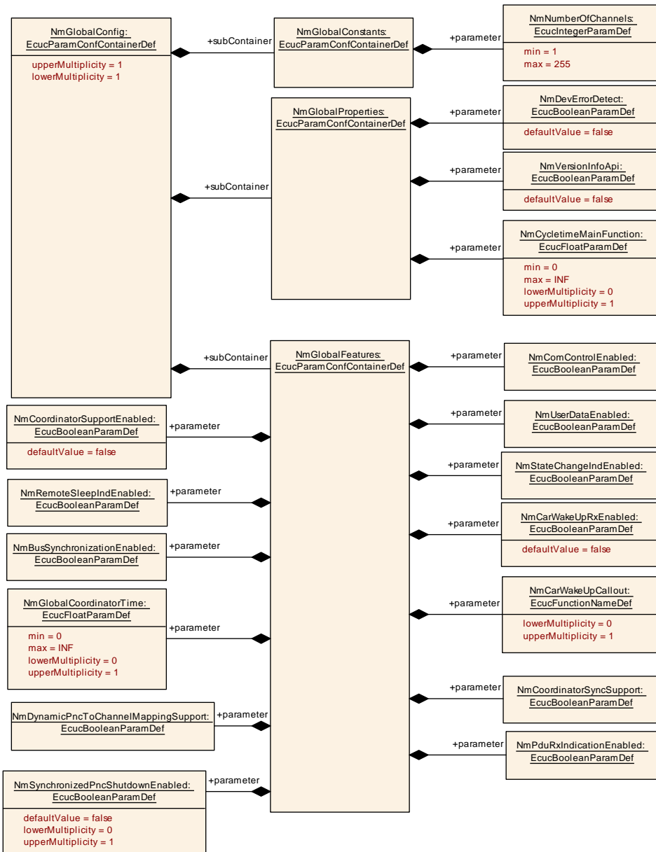
Figure 10.3: NmGlobalConfig overview
