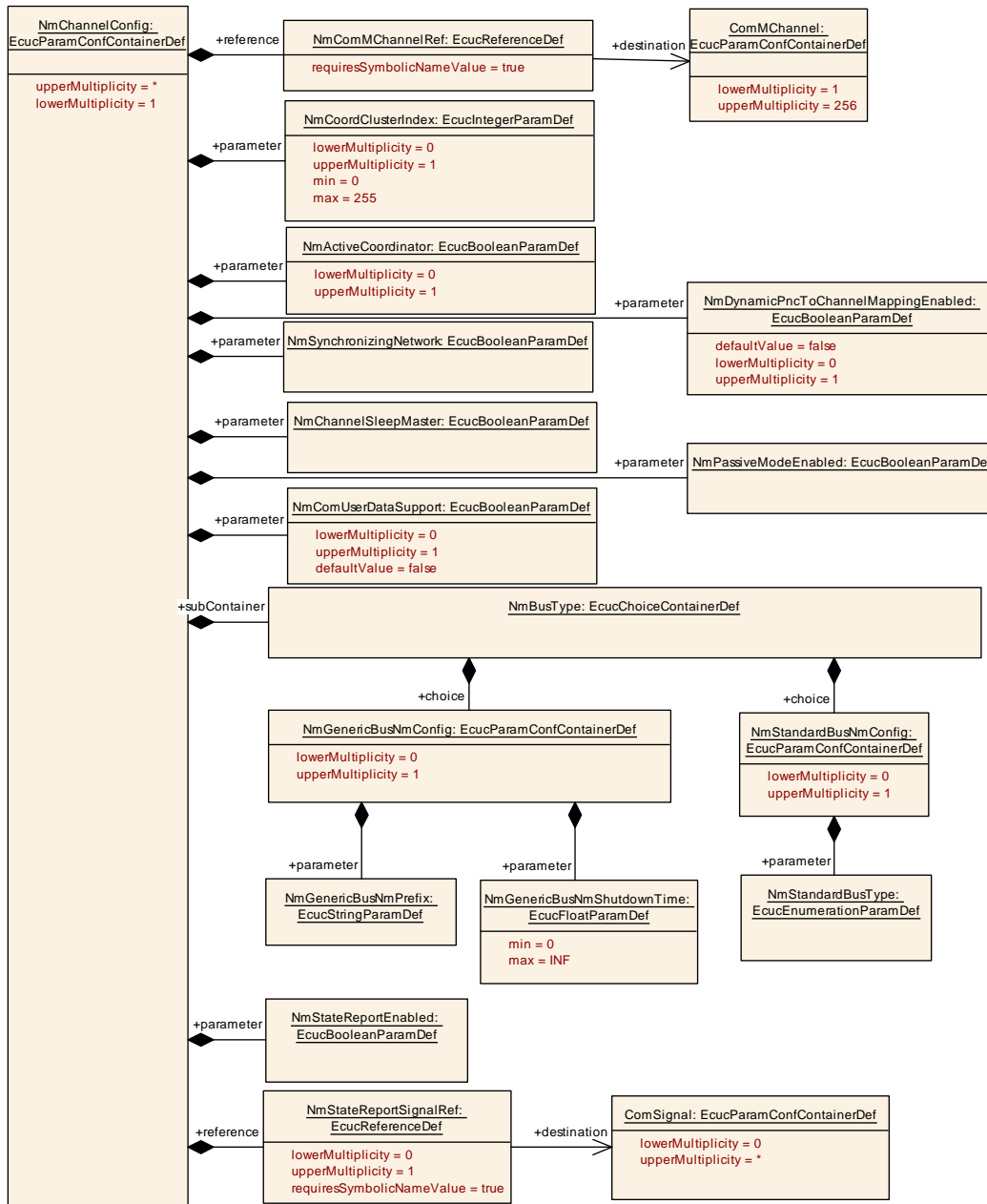
Figure 10.4: NmChannelConfig overview
