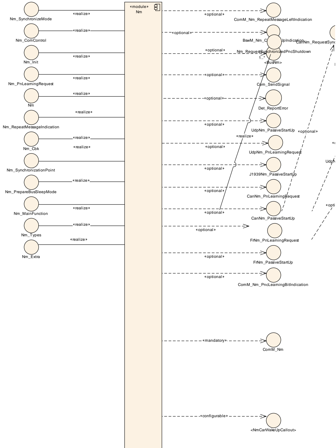
Figure 5.1: Nm's interfaces to other modules
