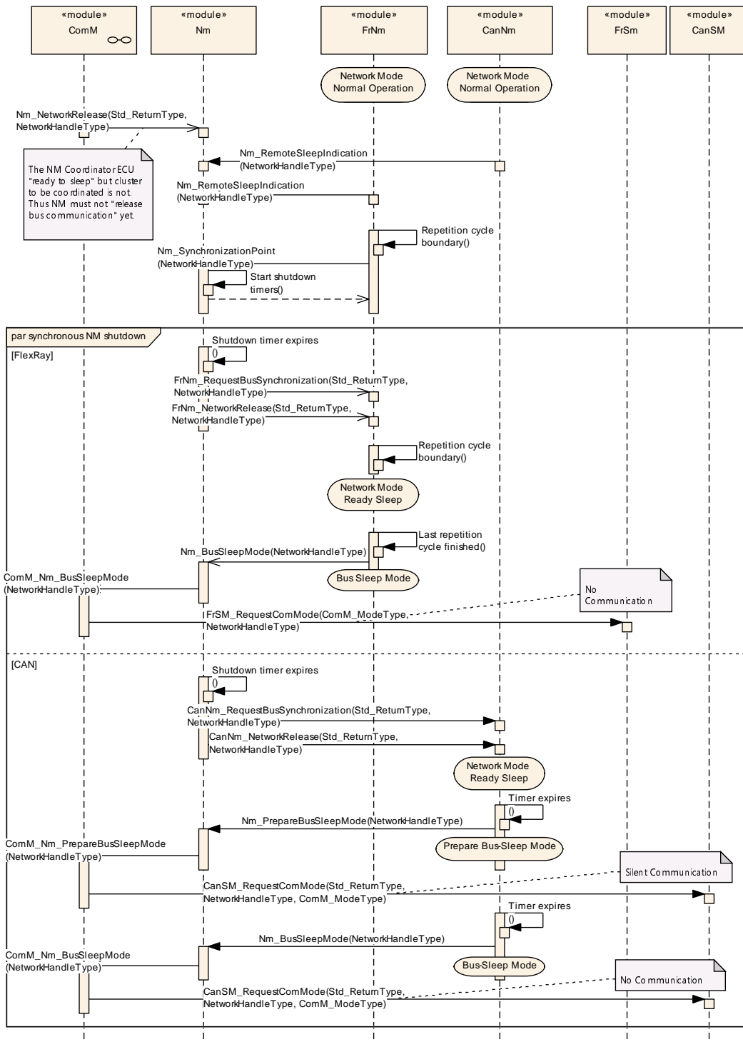
Figure 9.1: Nm Coordination
