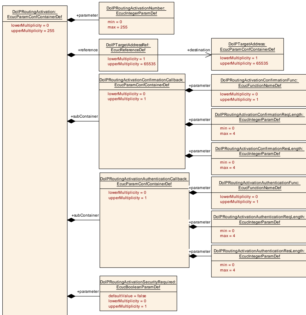
Figure 10.7: DoIPRoutingActivation
