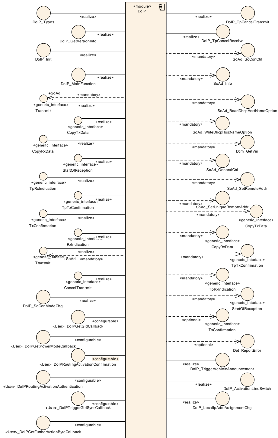
Figure 5.1: DoIPBSWInterfaces
