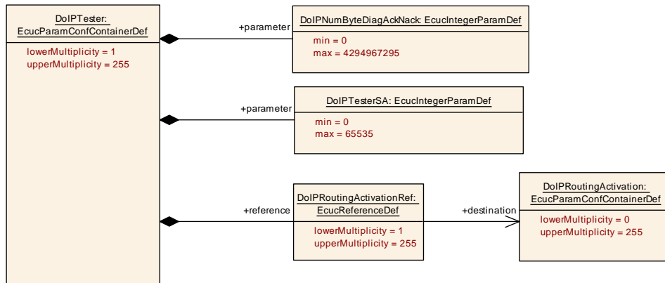
Figure 10.8: DoIPTester
