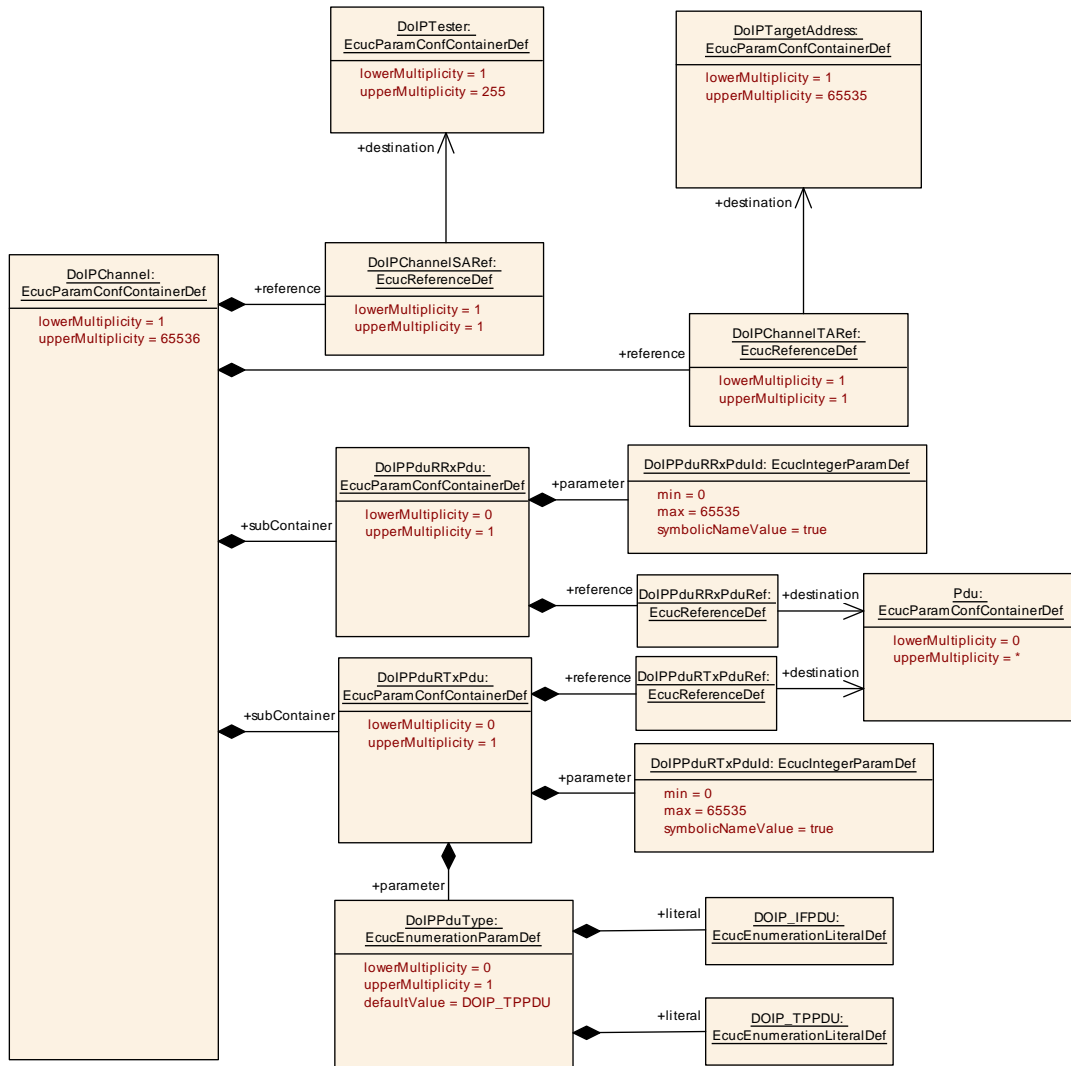
Figure 10.5: DoIPChannel
