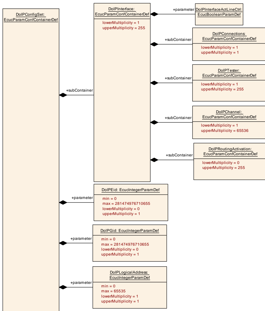
Figure 10.3: DoIPConfigSet
