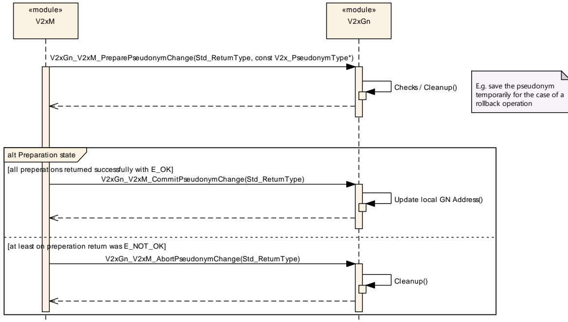
Figure 4 – V2xGn_V2xM_UpdatePseudonym
