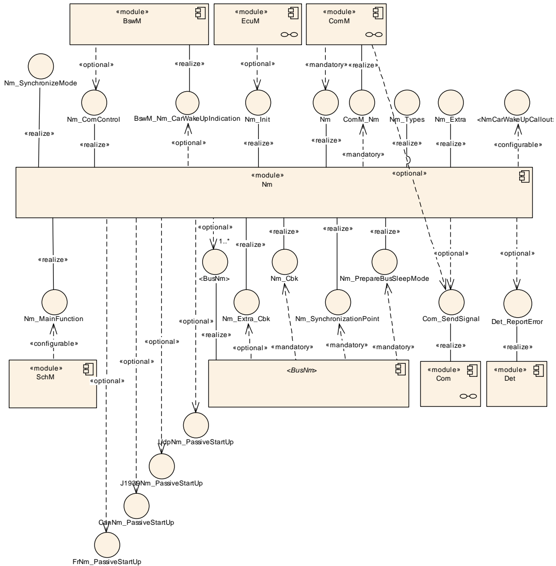
Figure 5.1: Nm's interfaces to other modules
