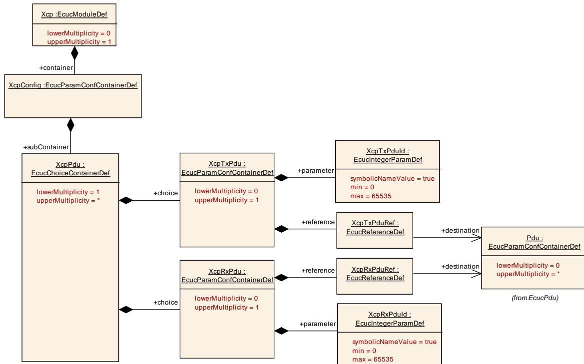
Figure 11: Diagram XcpPdu
