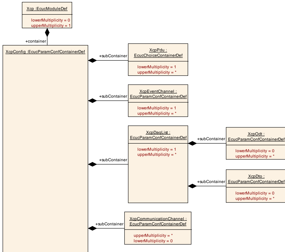
Figure 9: Diagram XcpConfig
