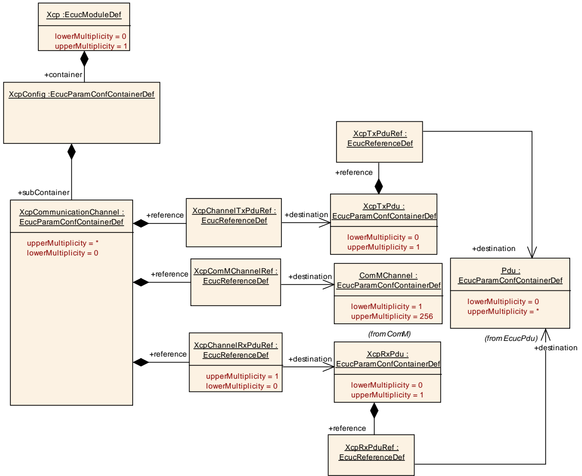
Figure 12: Diagram XcpCommunicationChannel
