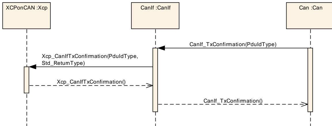
Figure 6: Xcp on CAN Transmit Confirmation
