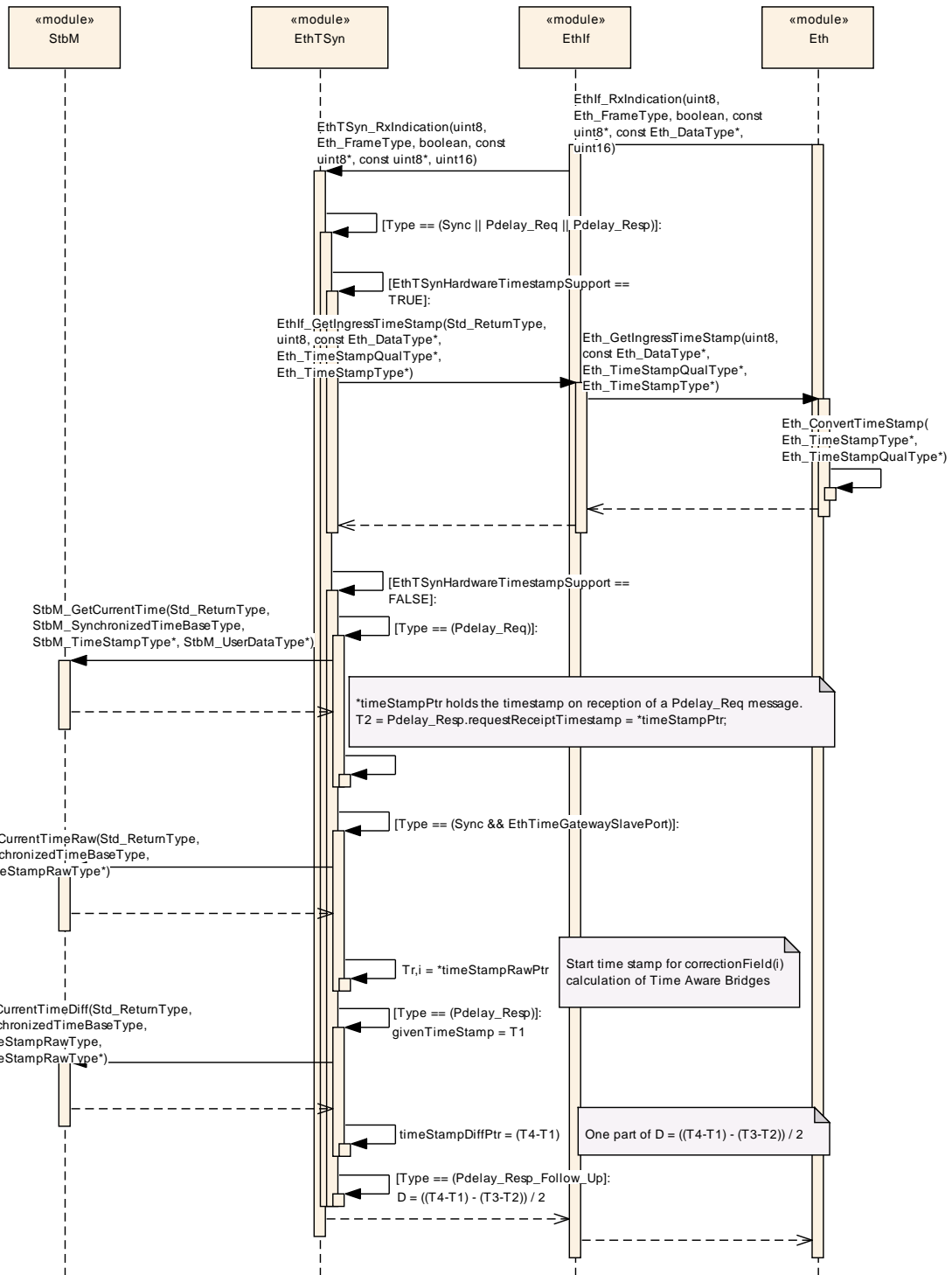
Figure 19: Time Slave Sync/Follow_Up and Pdelay – Rx
