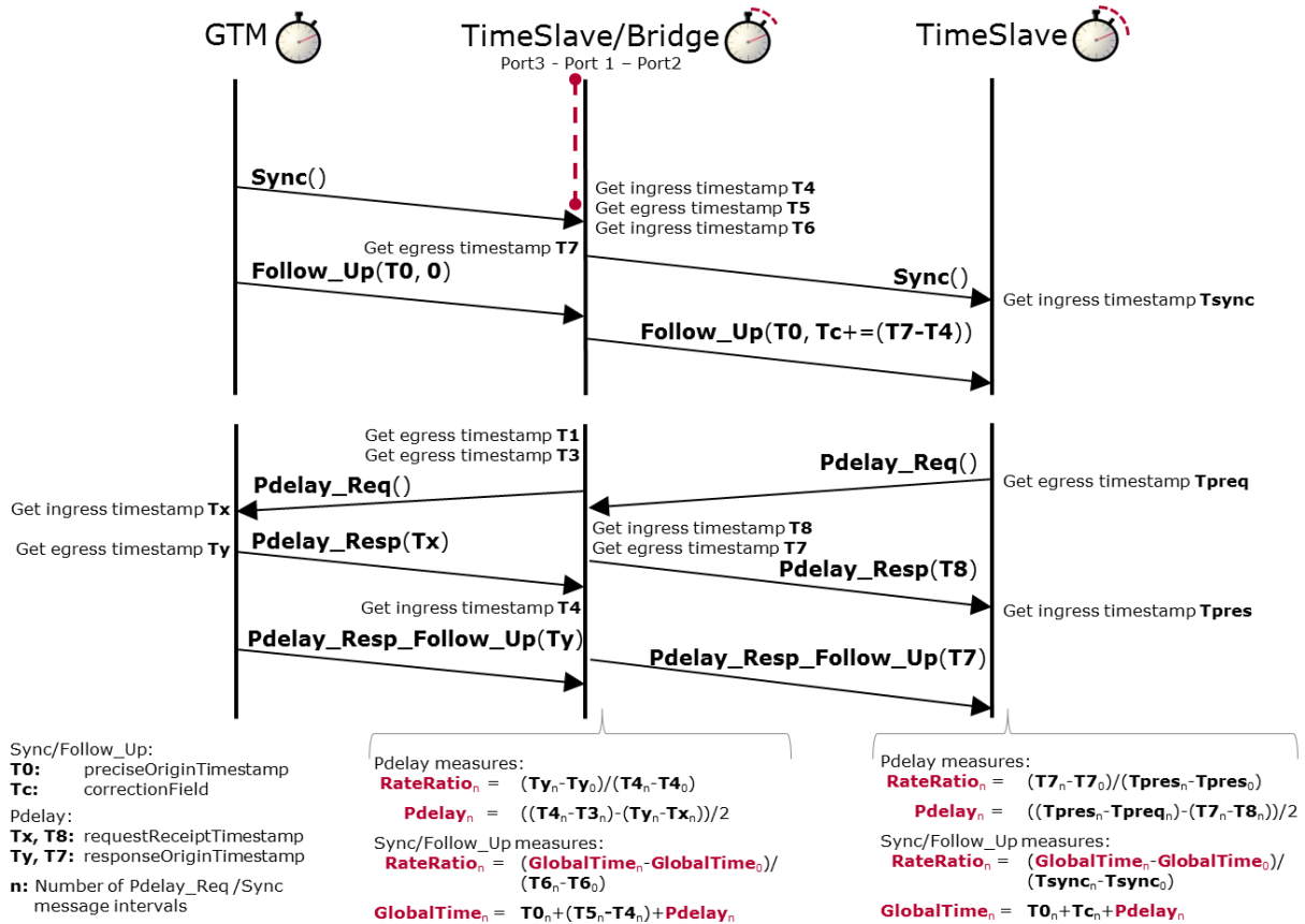
Figure 16: Timestamping sequence for Time Aware Bridge with GTM not as Management CPU |(SRS_StbM_20048, SRS_StbM_20059)
