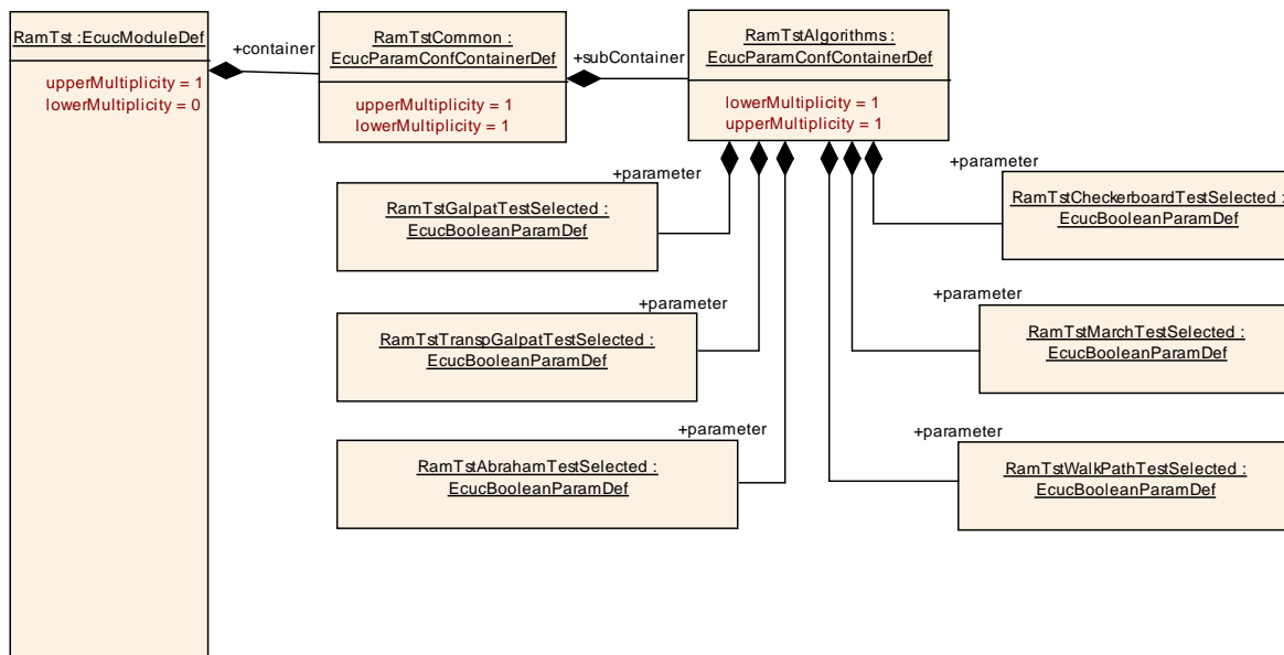
Figure 17: RamTstAlgorithms
