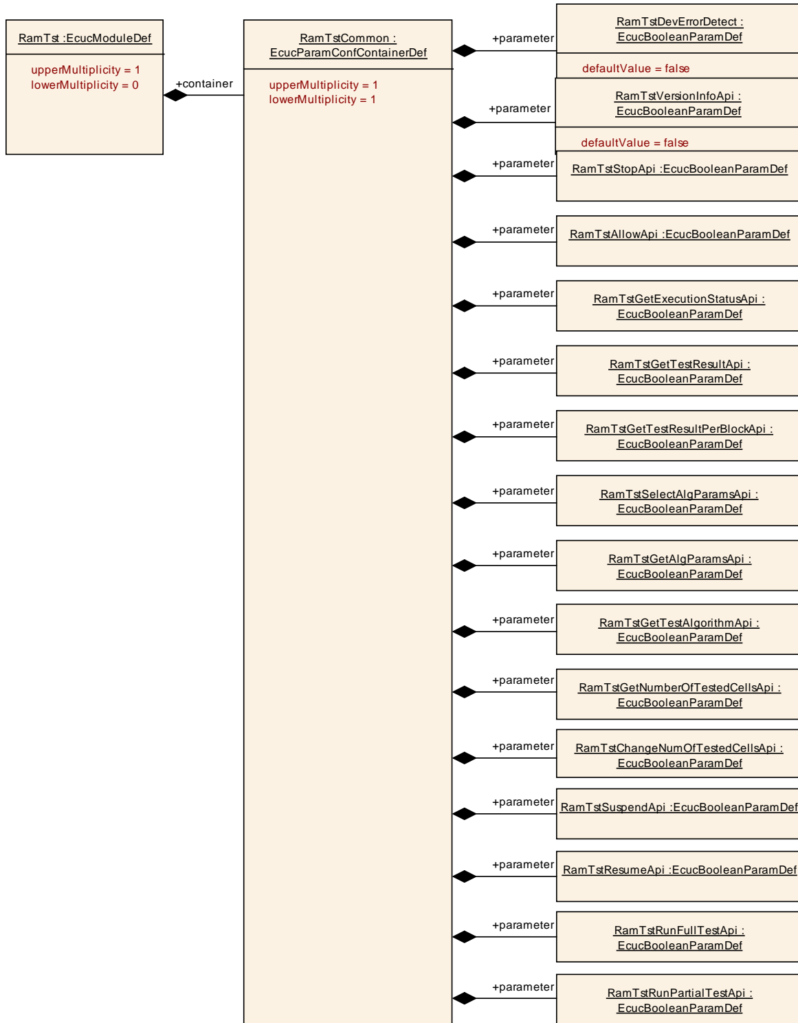
Figure 16: RamTstCommon
