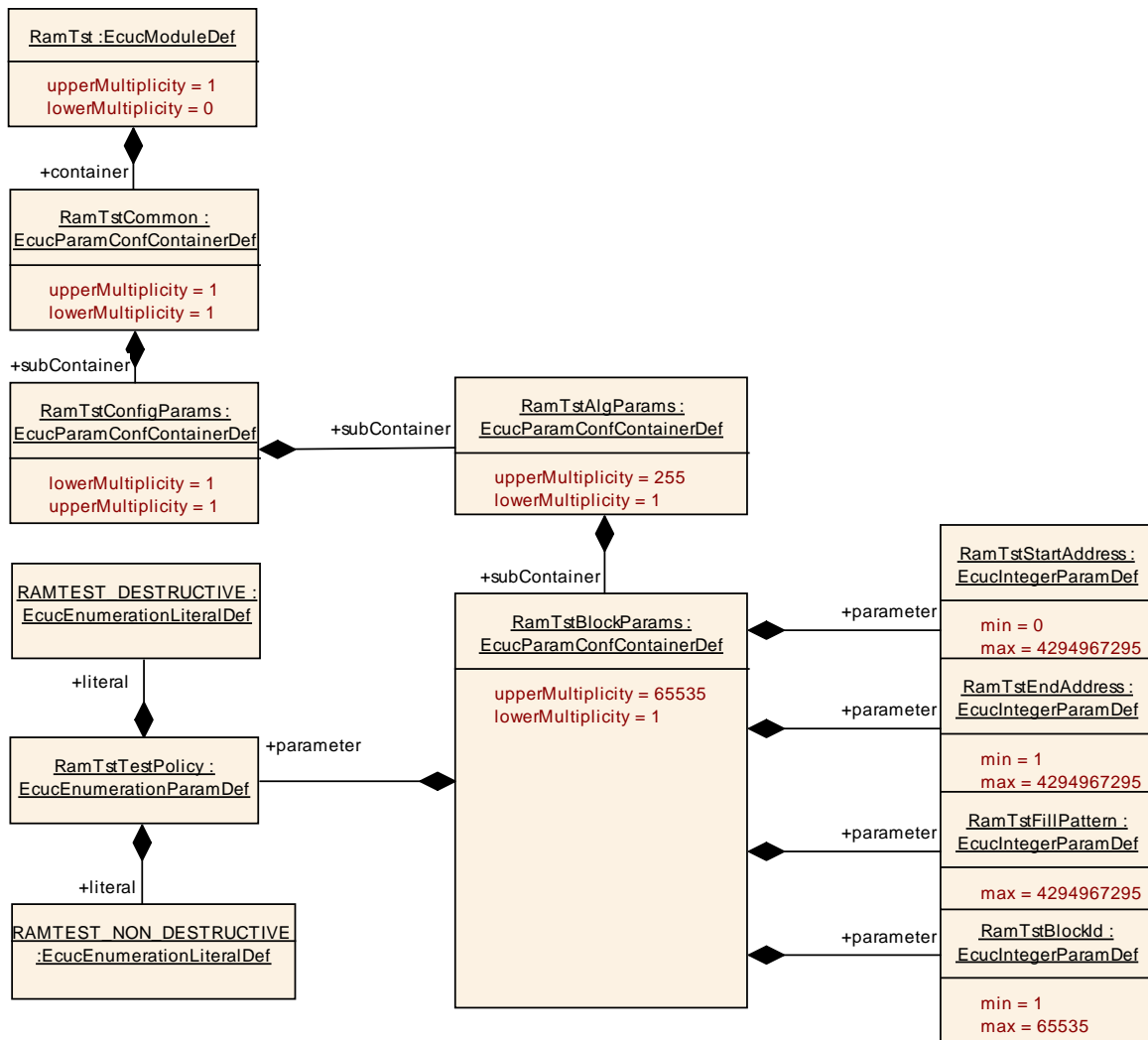
Figure 20: RamTstBlockParams
