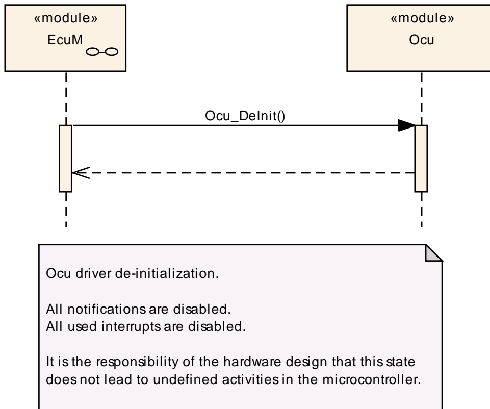
Figure 12: Ocu de-initialization
