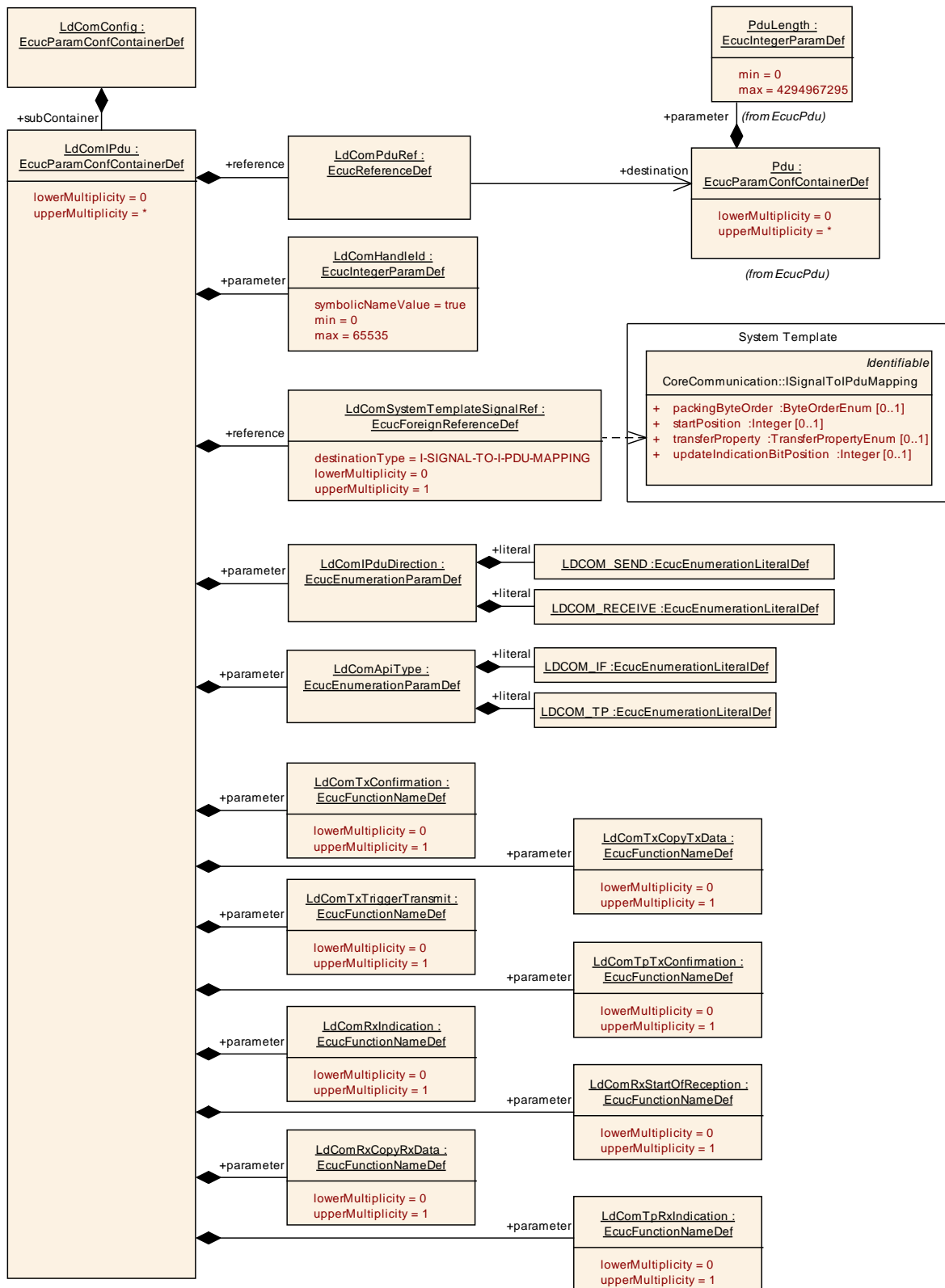
Figure 7 : Configuration LdComIPdu
