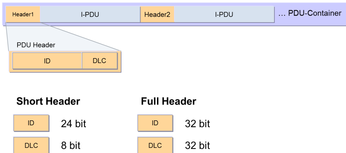
Figure 5 Layout of a dynamic Container
