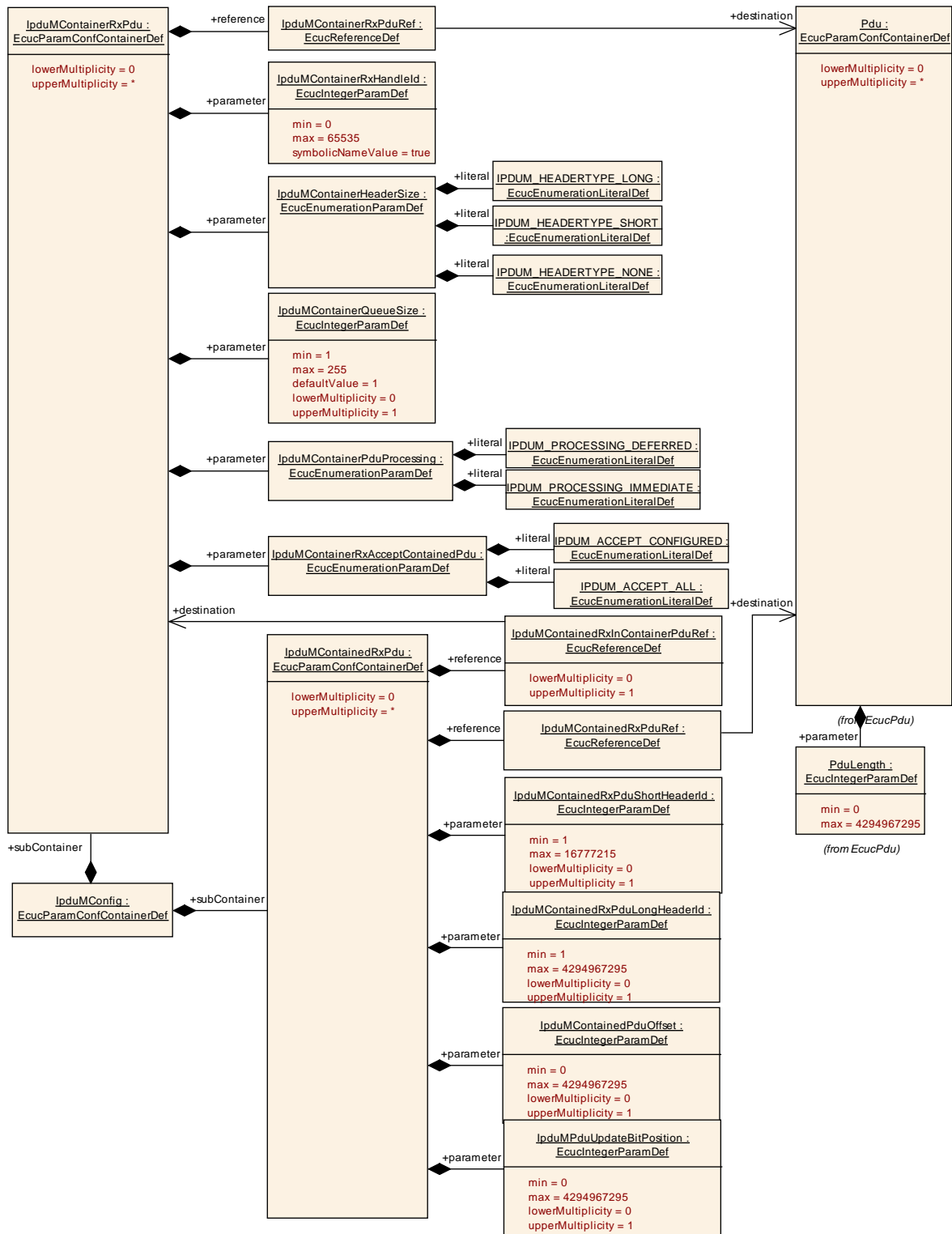
Figure 11 Configuration Overview RxContainer
