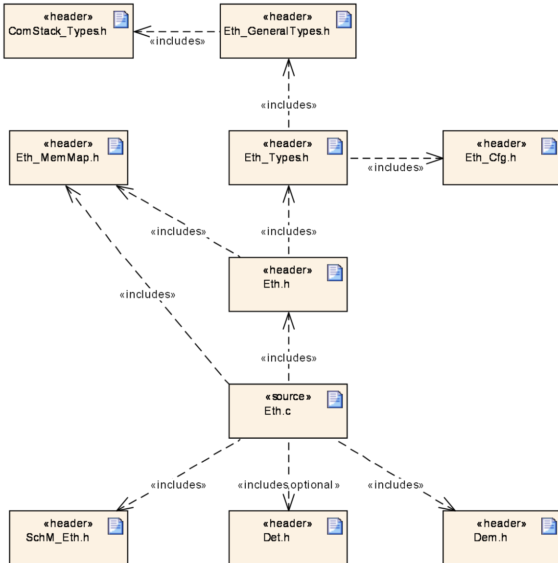
Figure 5.1 Ethernet Driver file structure
