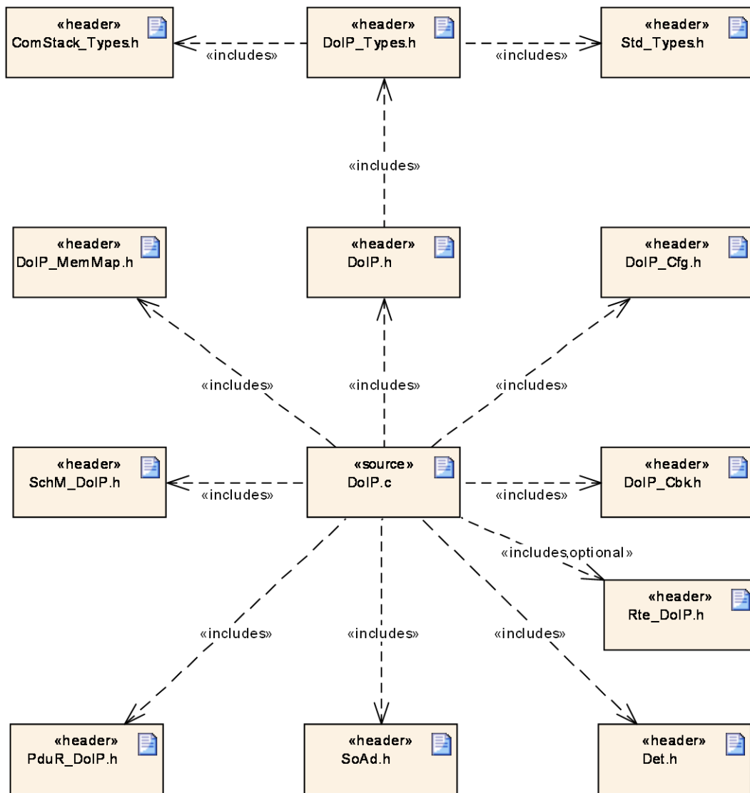
Figure 2: AUTOSAR DoIP header file structure
