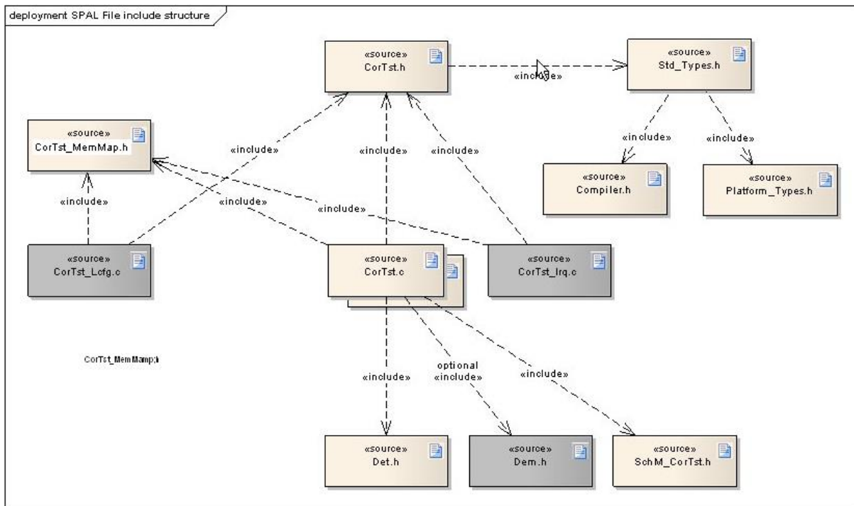
Figure 1 – File structure
