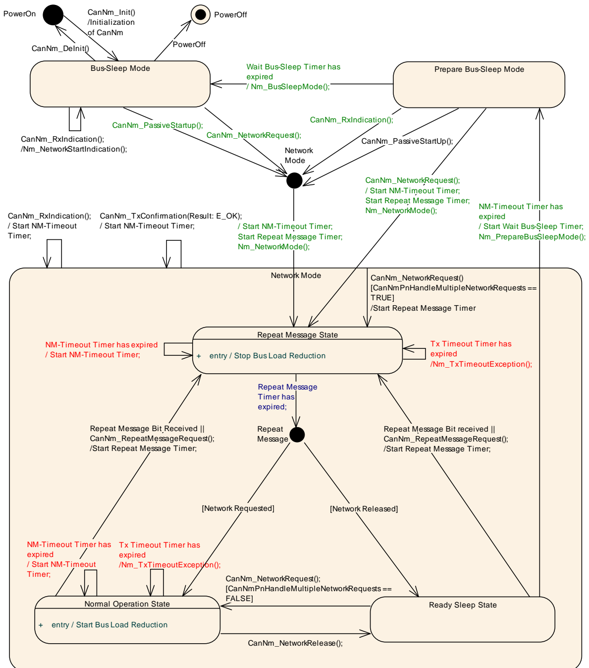
Figure 7-5 CanNm Algorithm
