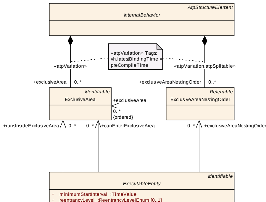
Figure 7.14: Description of nested usage of ExclusiveArea
