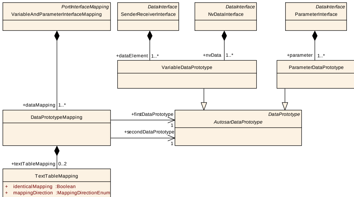
Figure 4.10: Mapping of Sender Receiver Interface, Parameter Interface and Non Volatile Data Interface elements
