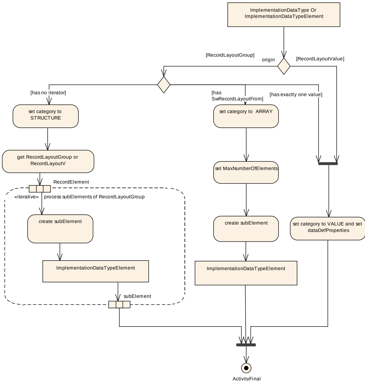
Figure 5.52: refining subElements
