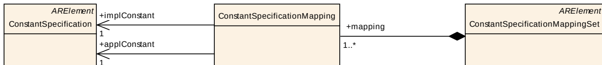
Figure 5.59: Constant Mapping
