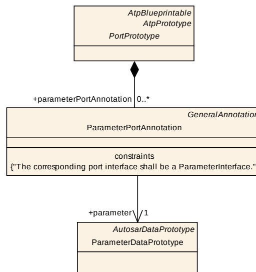
Figure 4.23: ParameterPortAnnotation
