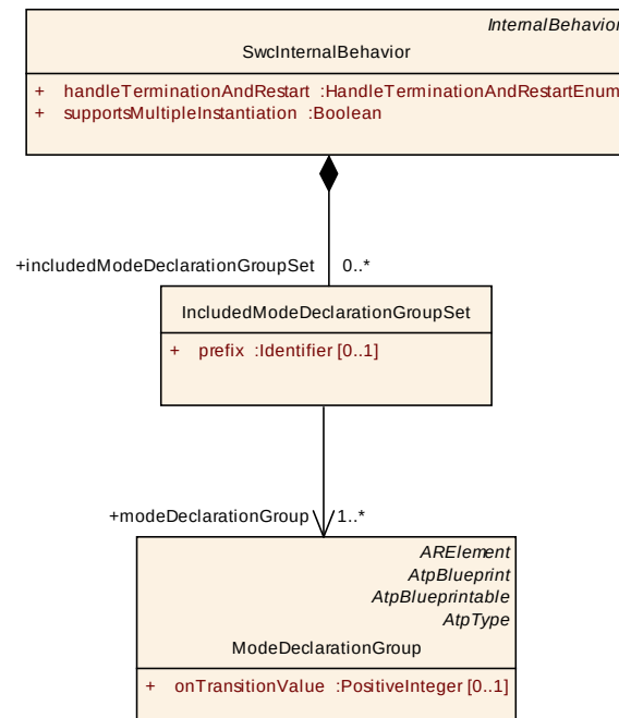
Figure 7.34: Included ModeDeclarationGroups
