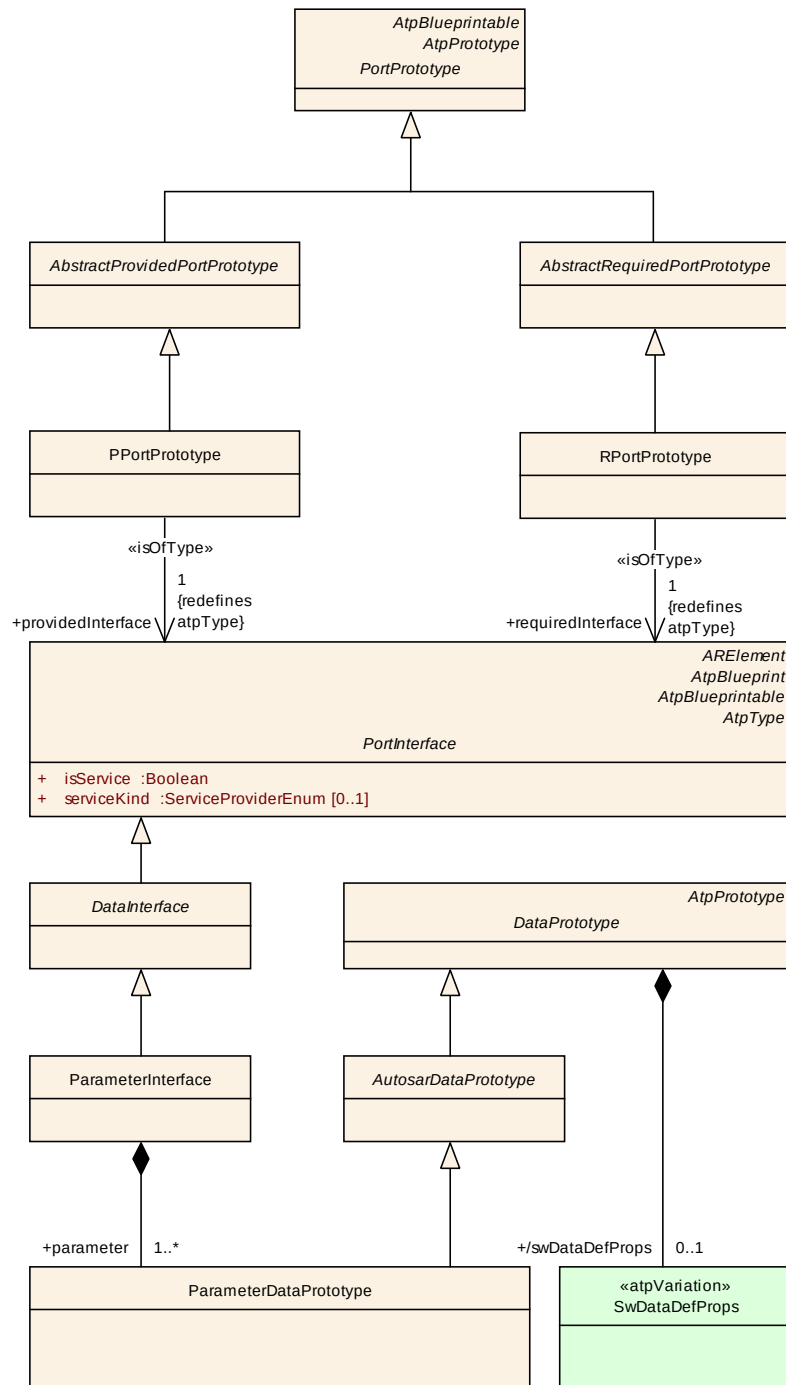
Figure 2.2: ParameterInterface
