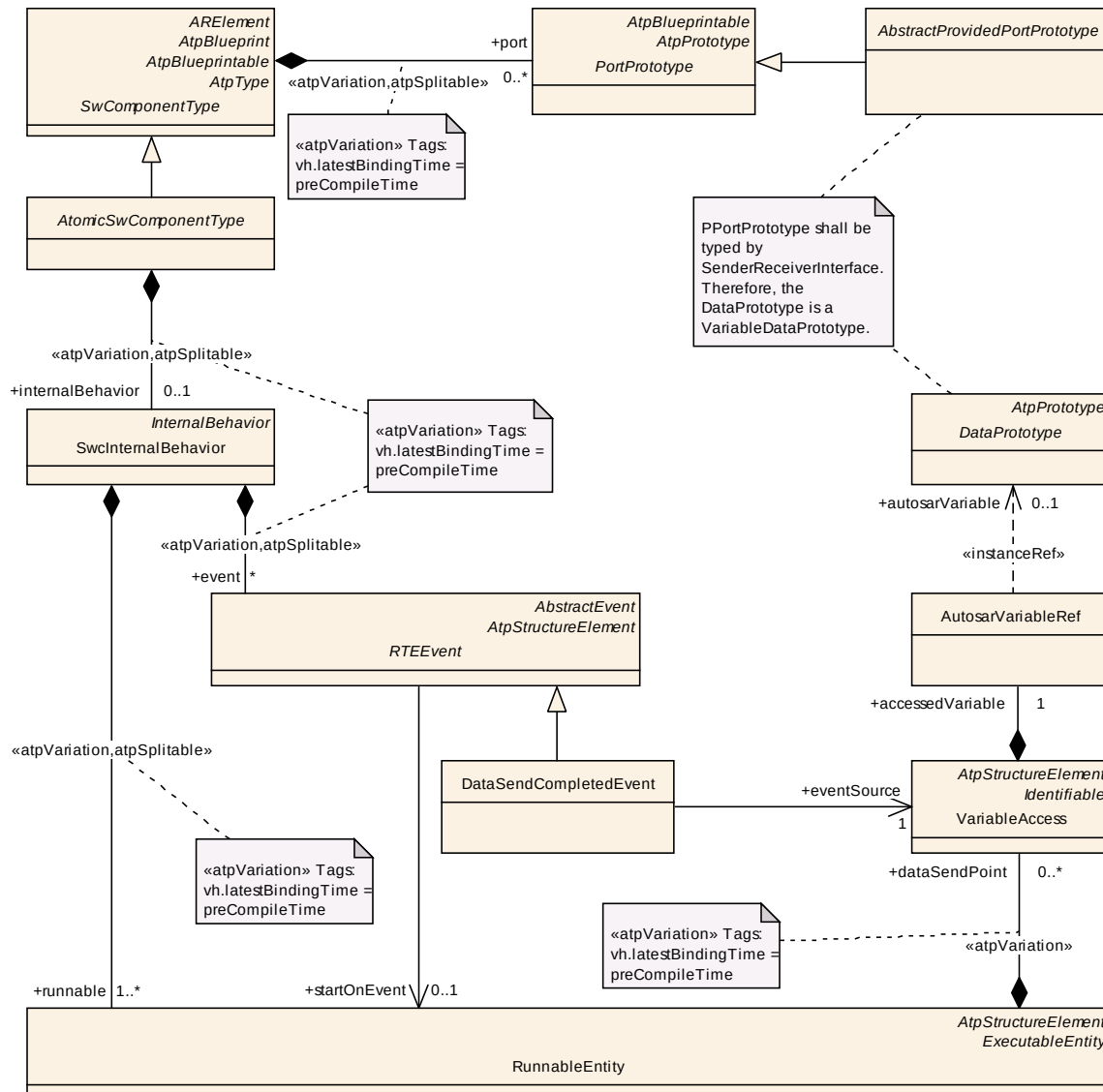
Figure 7.19: DataSendPoint
