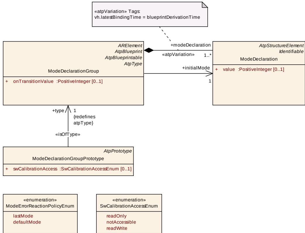
Figure 9.1: ModeDeclaration
