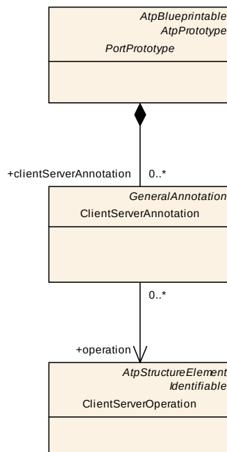
Figure 4.21: ClientServerAnnotation
