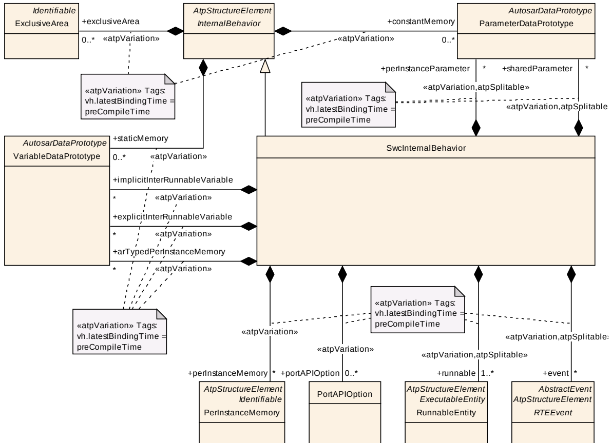
Figure 7.2: SwcInternalBehavior
