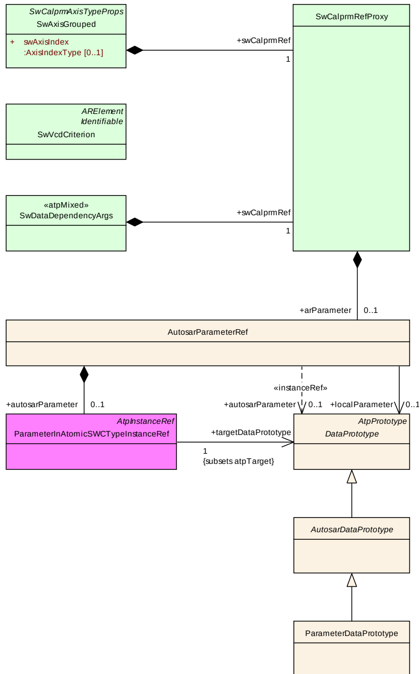
Figure 5.33: Applying Proxy Parameter Reference Mechanism
