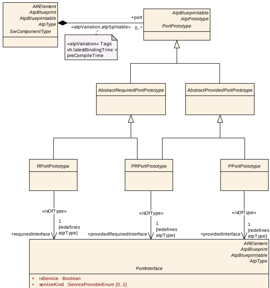
Figure 3.3: Components and Ports
