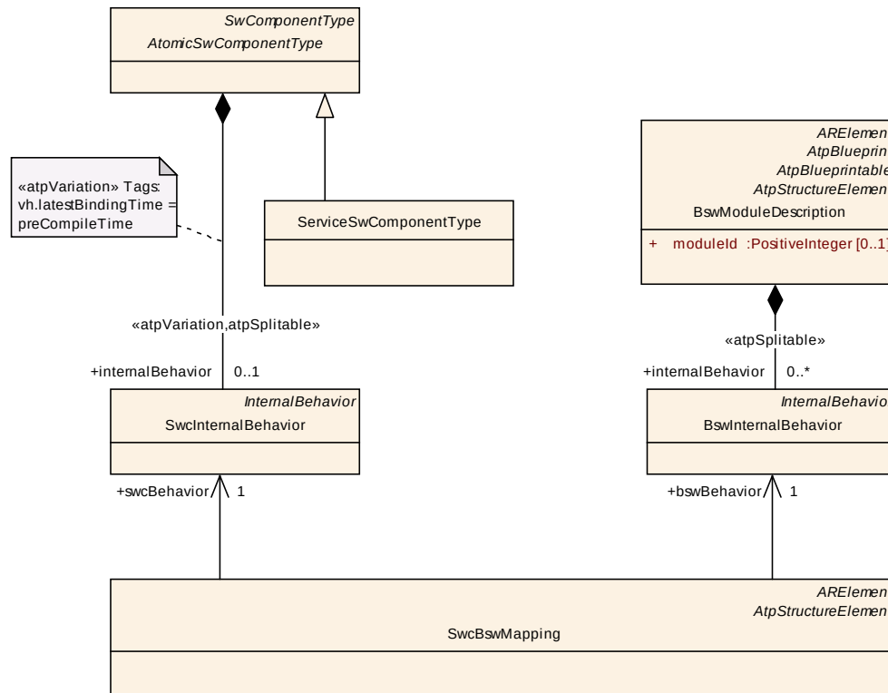
Figure 11.2: ServiceSwComponentType
