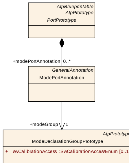
Figure 4.24: ModePortAnnotation
