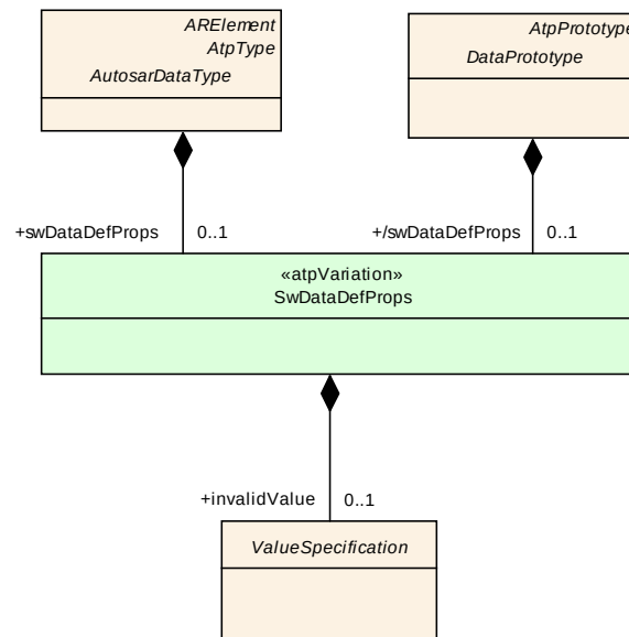
Figure 5.25: Invalid value
