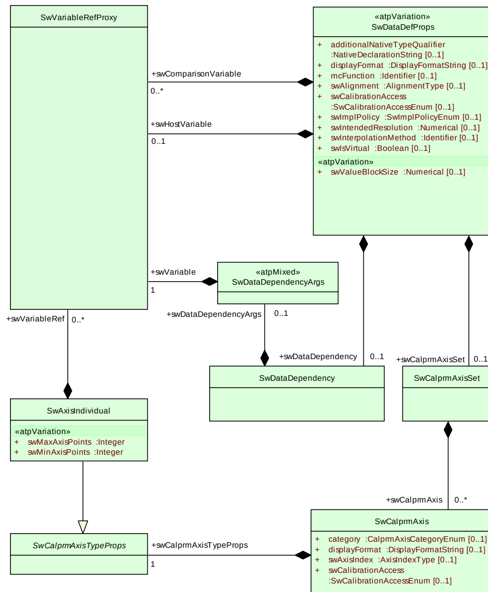
Figure 5.32: Applying Proxy Variable Reference Mechanism
