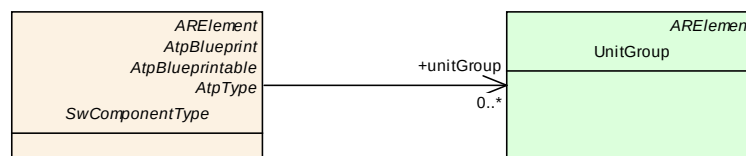
Figure 5.40: Relation of SwComponentType to UnitGroup
