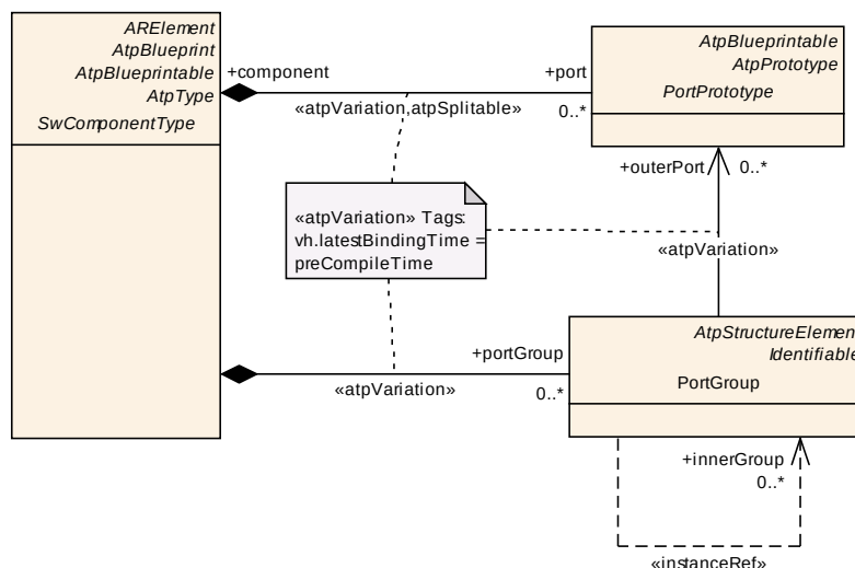
Figure 4.41: Declaration of PortGroups
