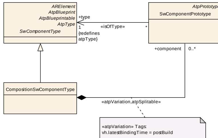
Figure 3.7: The recursive relation of software-components and compositions
