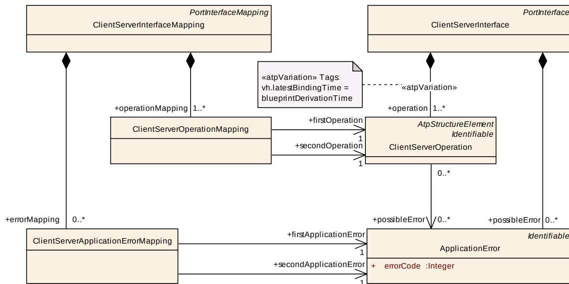
Figure 4.11: Mapping of ClientServerInterface elements and mapping of arguments
