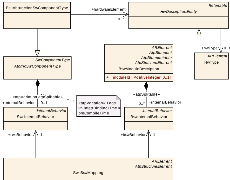
Figure 10.7: EcuAbstractionSwComponentType
