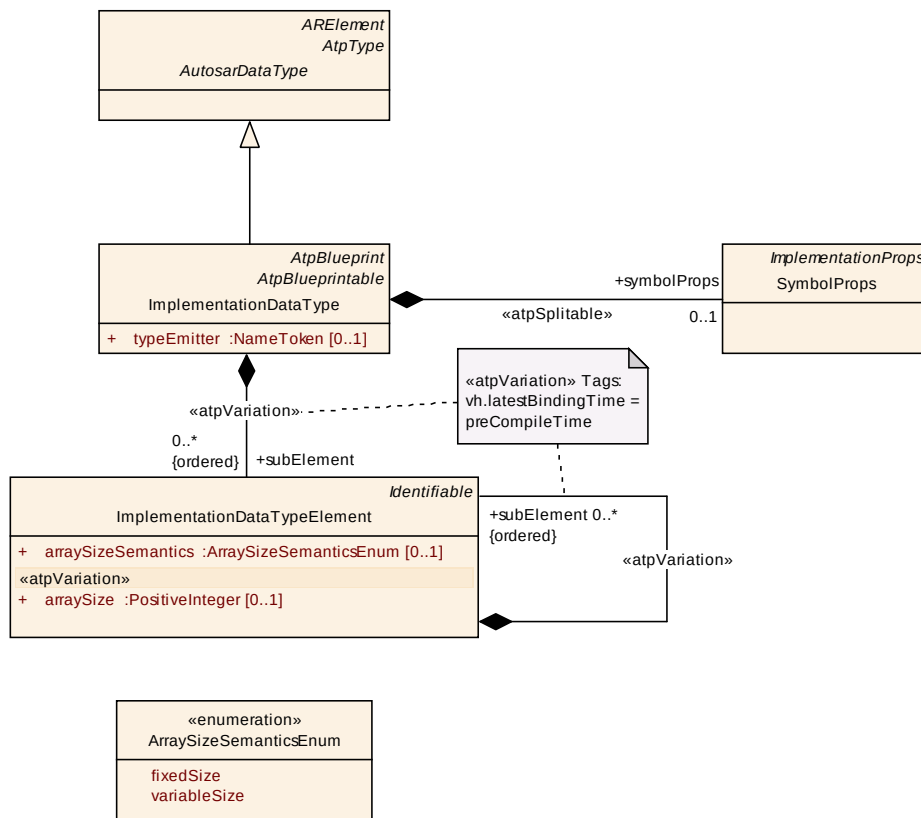
Figure 5.11: ImplementationDataType overview
