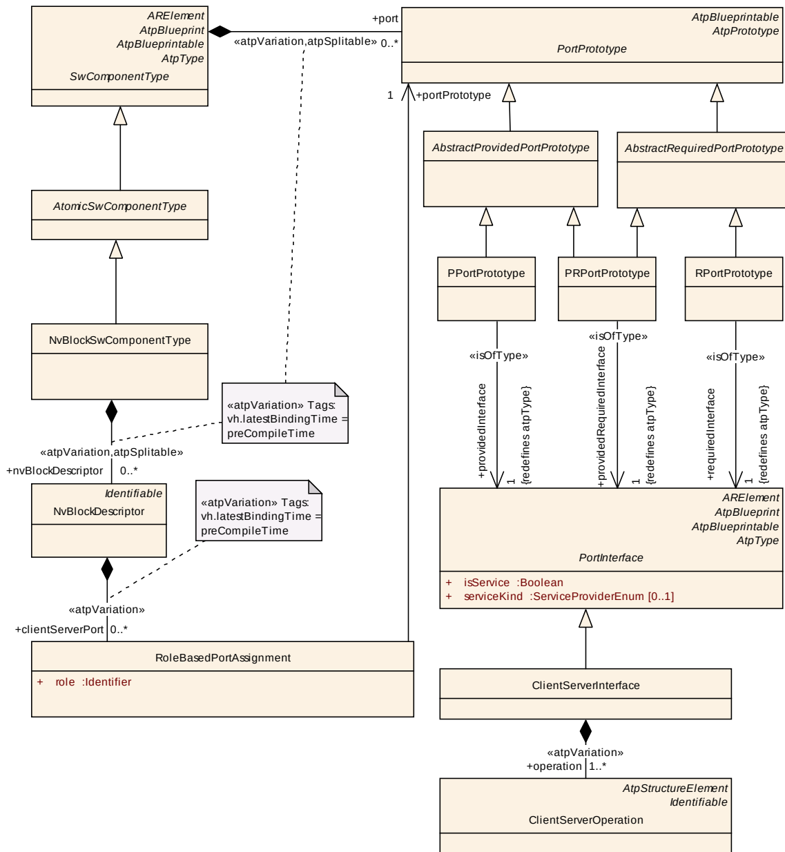
Figure 11.8: NvBlockNotification
