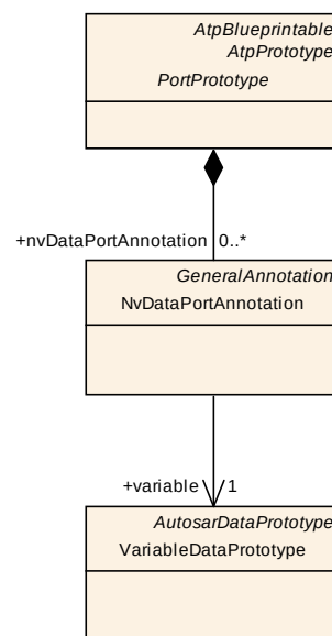
Figure 4.26: NvDataPortAnnotation
