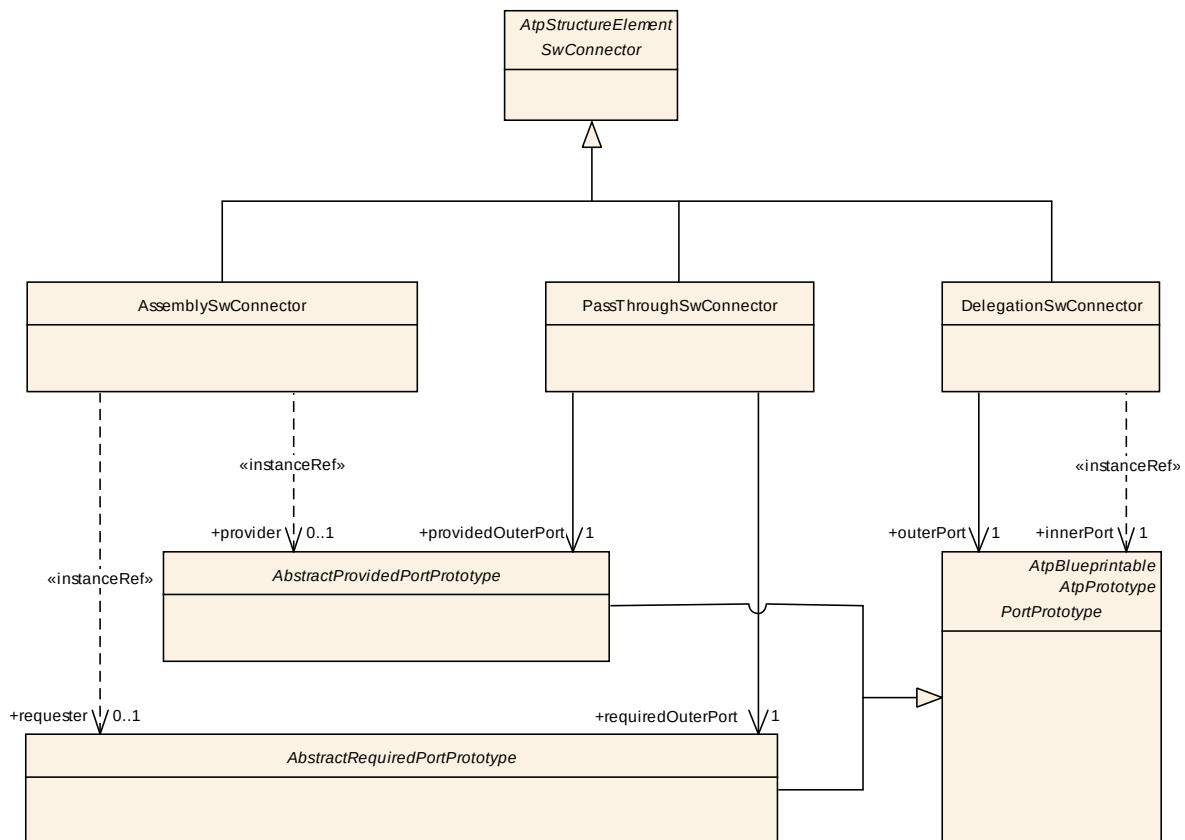
Figure 3.10: Connectors
