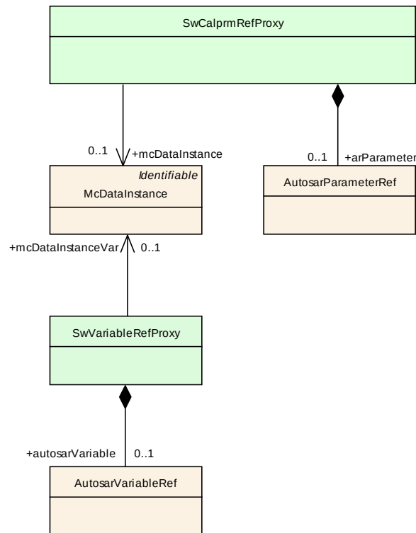
Figure 5.34: Proxy reference classes
