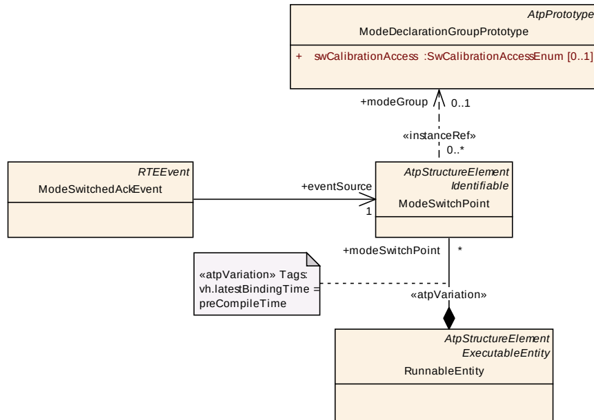
Figure 9.5: ModeSwitchPoint
