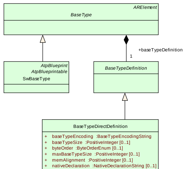
Figure 5.17: BaseType
