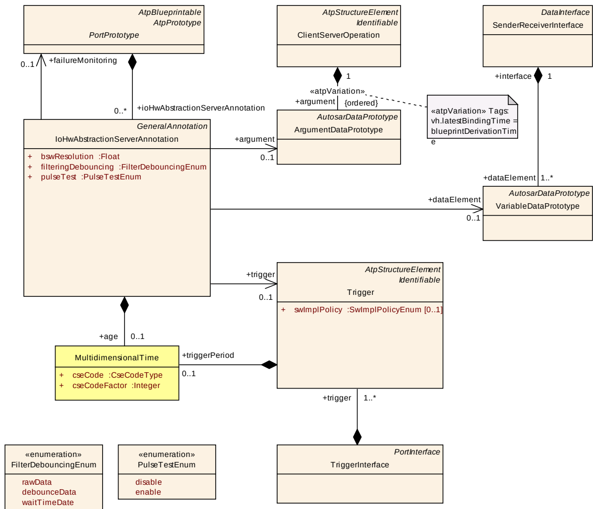
Figure 4.22: IoHwAbstractionServerAnnotation
