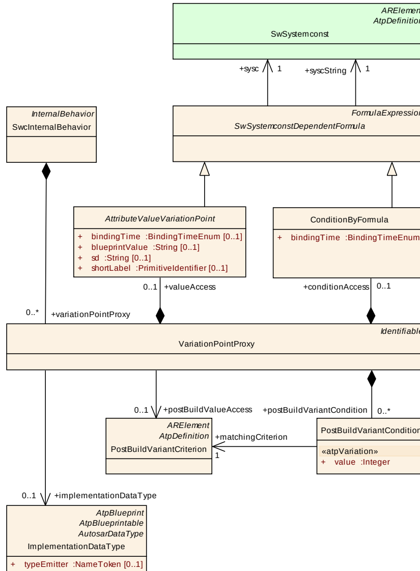
Figure 7.44: VariationPointProxy
