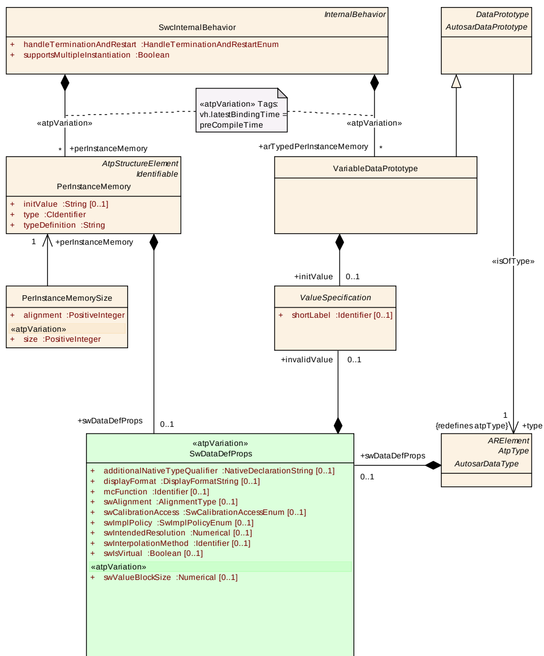
Figure 7.31: PerInstanceMemory
