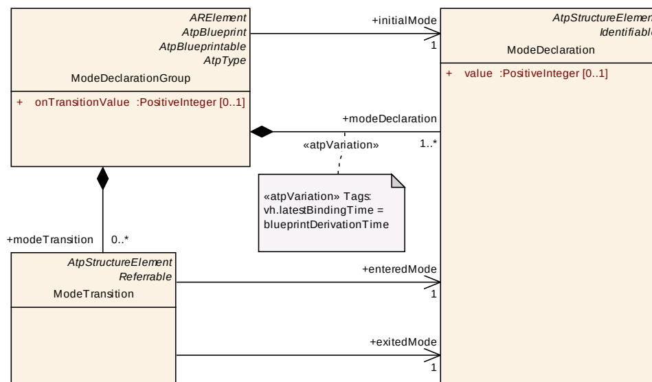
Figure 9.2: ModeTransition
