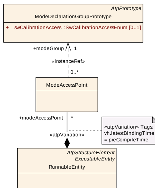
Figure 9.6: ModeAccessPoint
