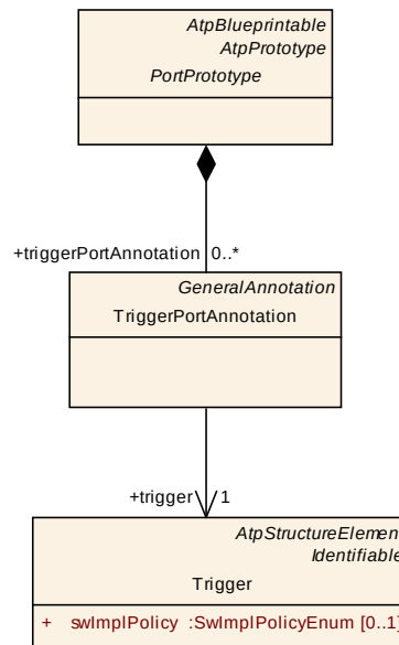
Figure 4.25: TriggerPortAnnotation
