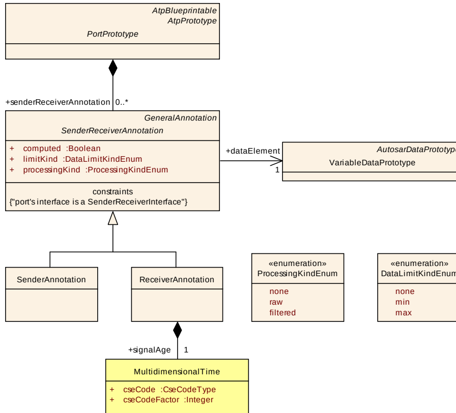
Figure 4.20: SenderReceiverAnnotation
