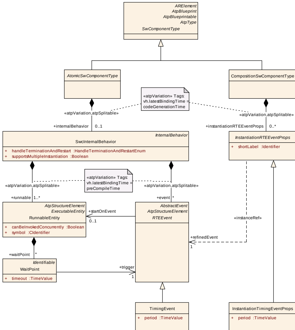
Figure 3.12: Instantiation specific Properties of RTEEvents
