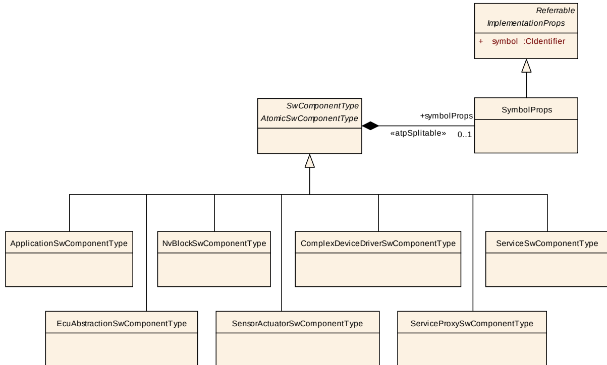
Figure 3.6: Overview of AtomicSwComponentType
