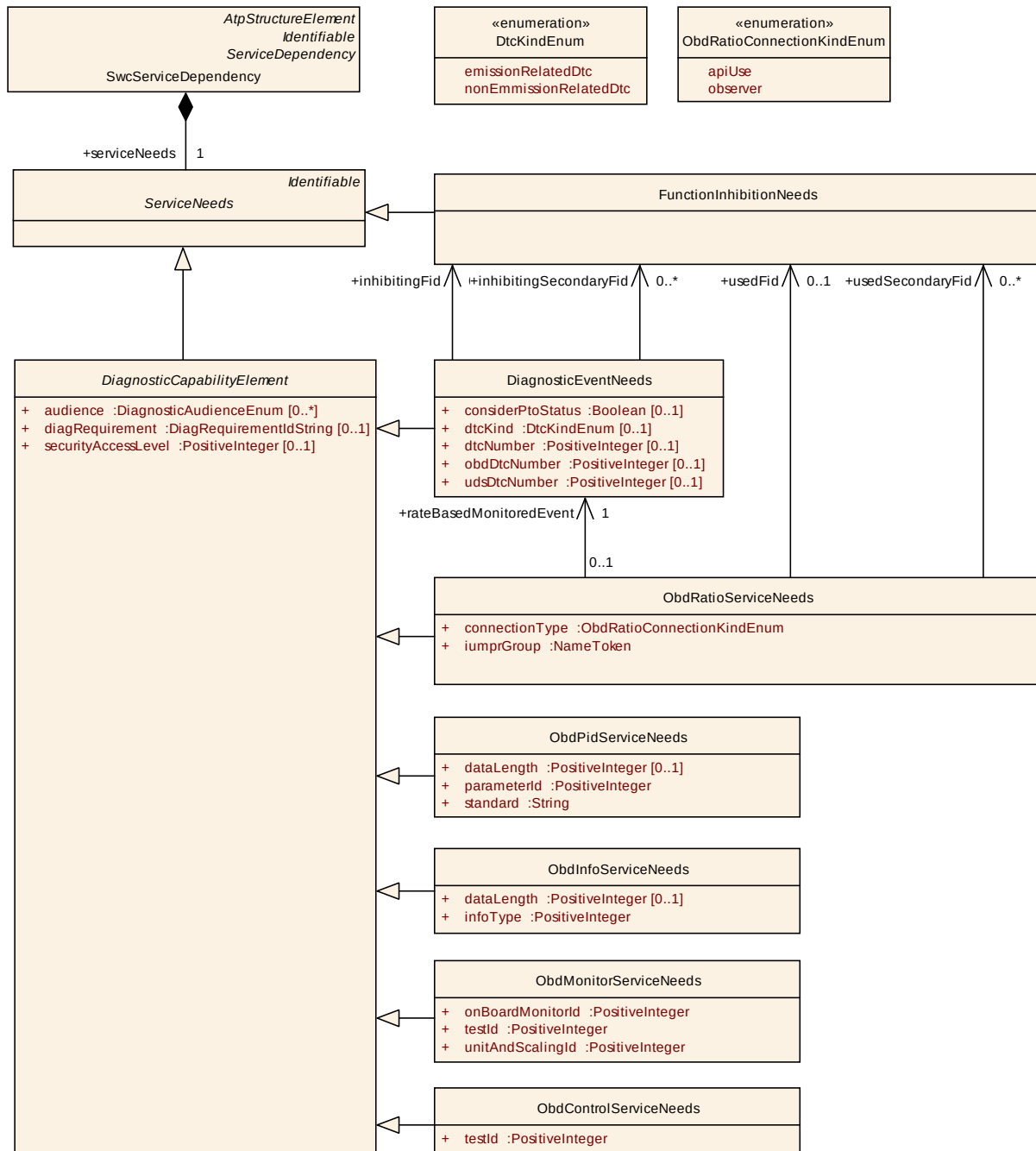
Figure 7.37: ServiceNeeds: Diagnostic-related ServiceNeeds with emphasis on OBD
