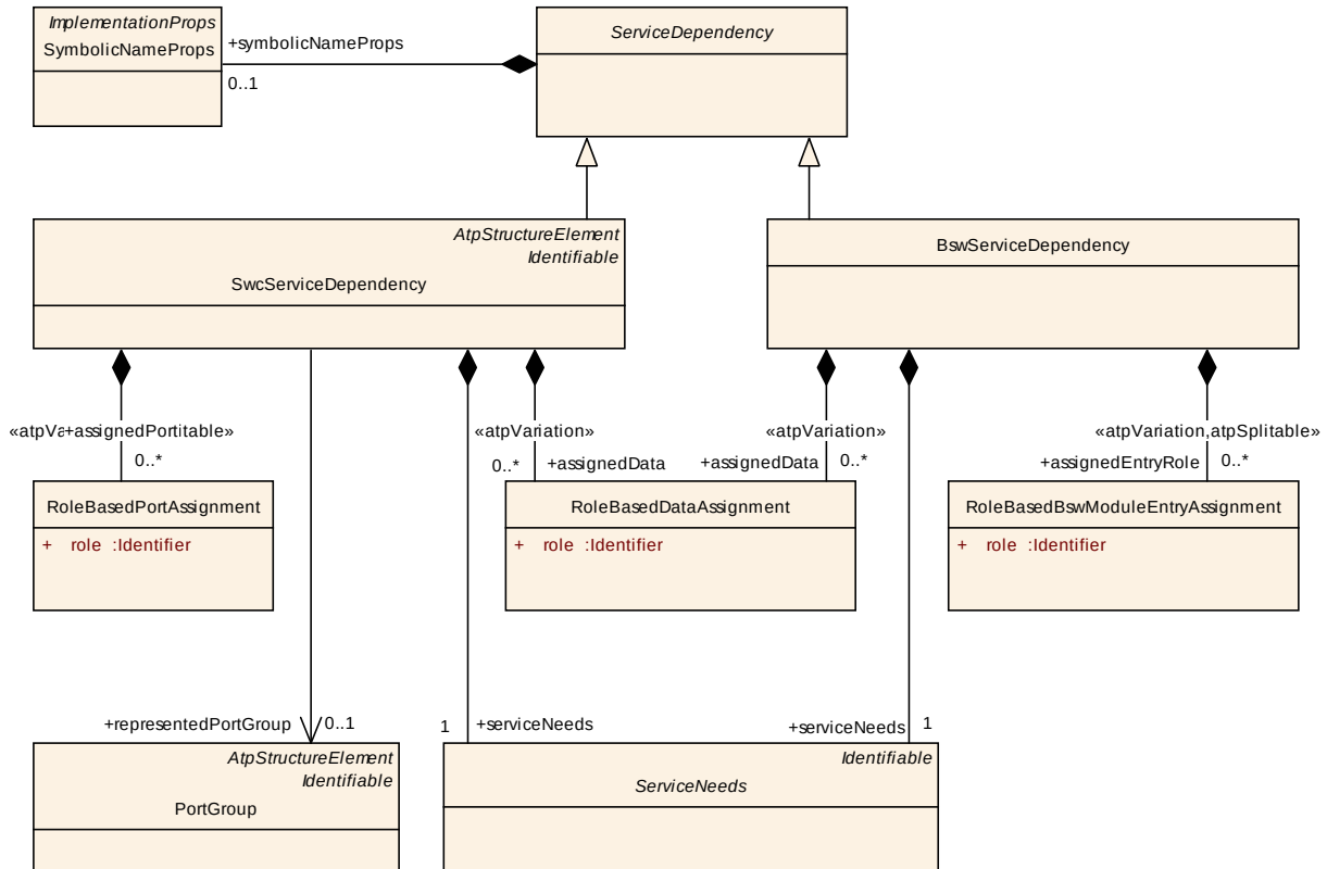
Figure 7.38: ServiceDependency is the abstract base class of SwcServiceDependency
