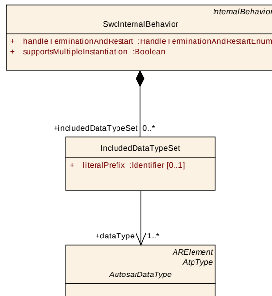
Figure 7.33: Included AUTOSAR Data Types
