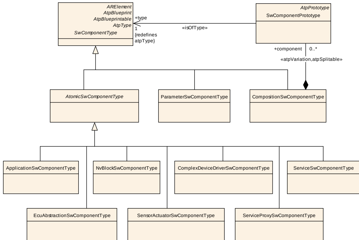
Figure 3.4: Overview of Component Types
