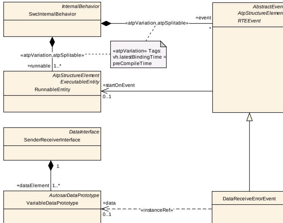
Figure 7.23: DataReceiveErrorEvent references a Runnable and a VariableDataPrototype
