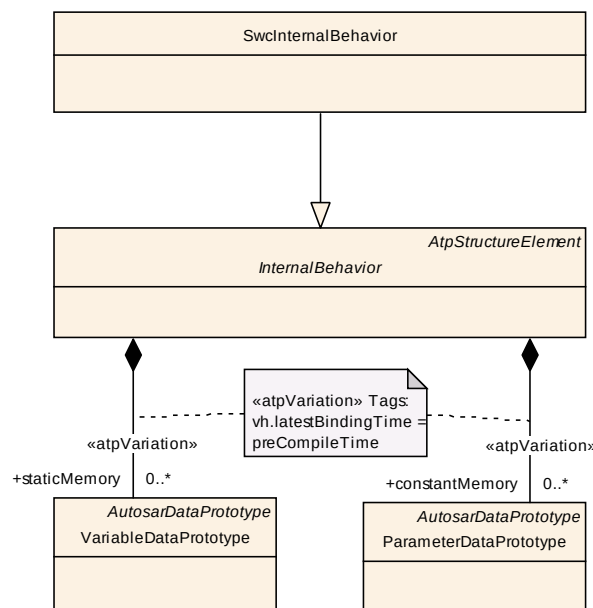
Figure 7.32: Static Memory and Constant Memory
