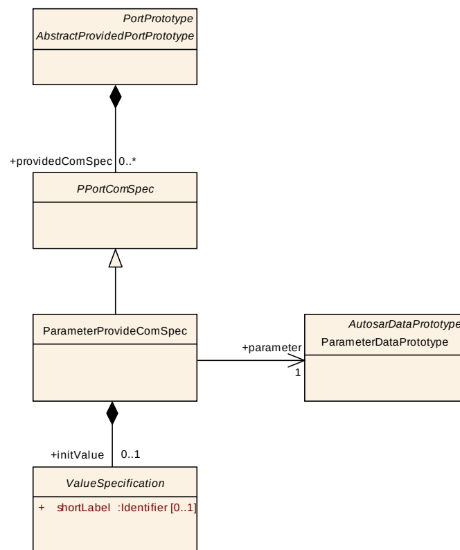
Figure 4.37: Communication attributes of ParameterDataPrototypes with respect to PPortPrototype
