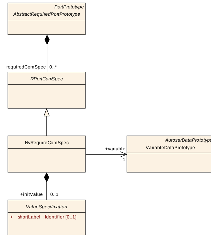
Figure 4.39: Communication attributes of a required VariableDataPrototype used in the context of an NvDataInterface
