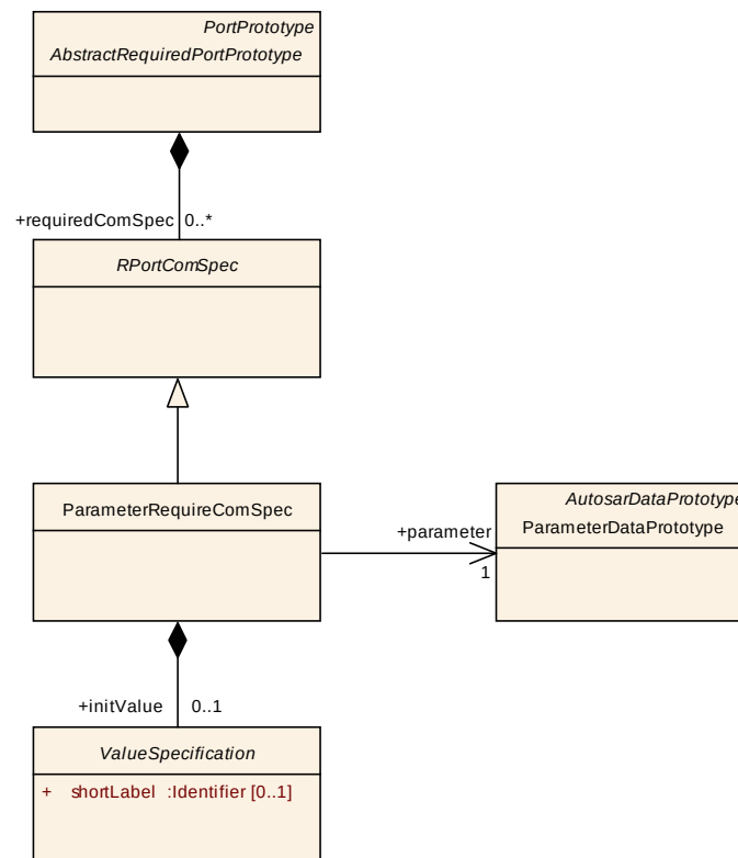
Figure 4.38: Communication attributes of ParameterDataPrototypes with respect to RPortPrototype
