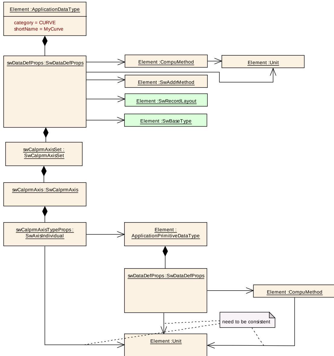
Figure 5.30: Illustration of a Curve in M1
