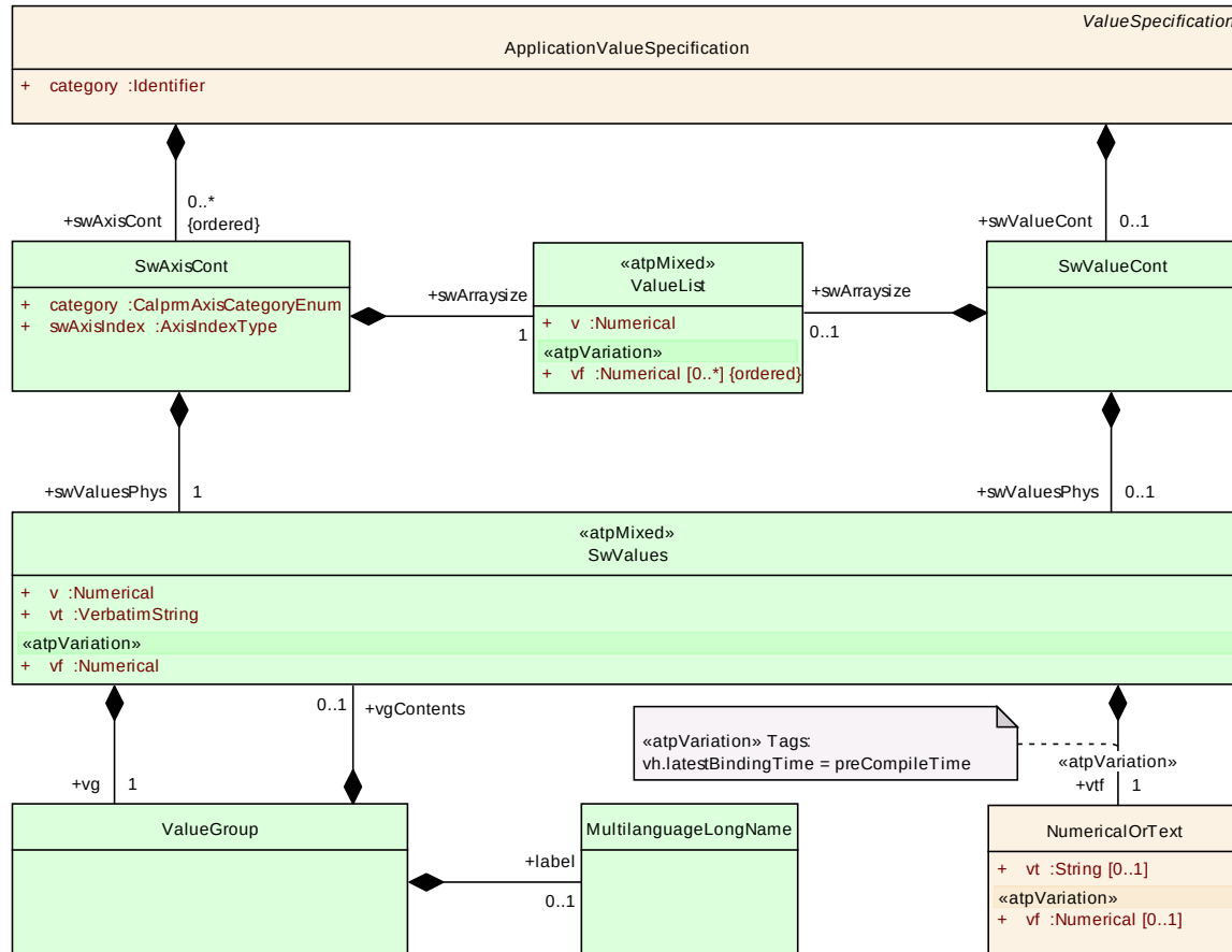
Figure 5.58: Definition of an ApplicationValueSpecification
