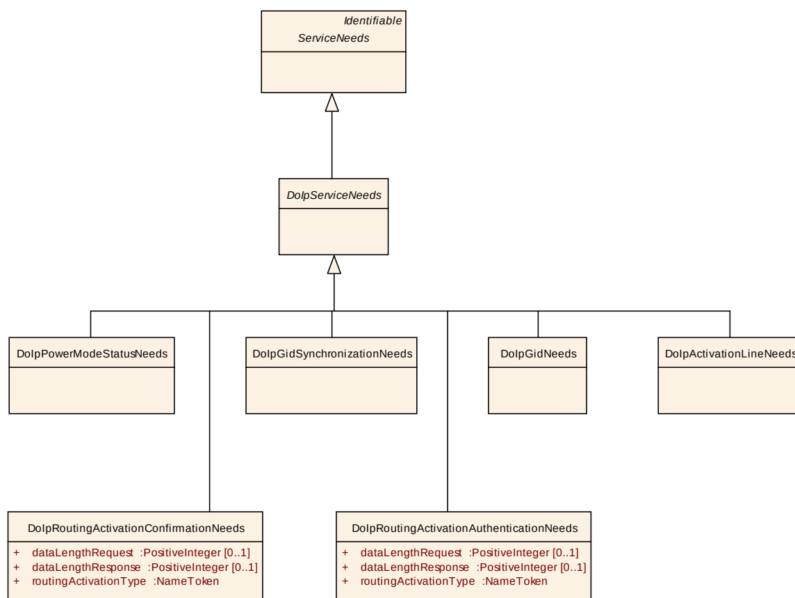
Figure 7.43: Subclasses of ServiceNeeds for implementing diagnostics over IP
