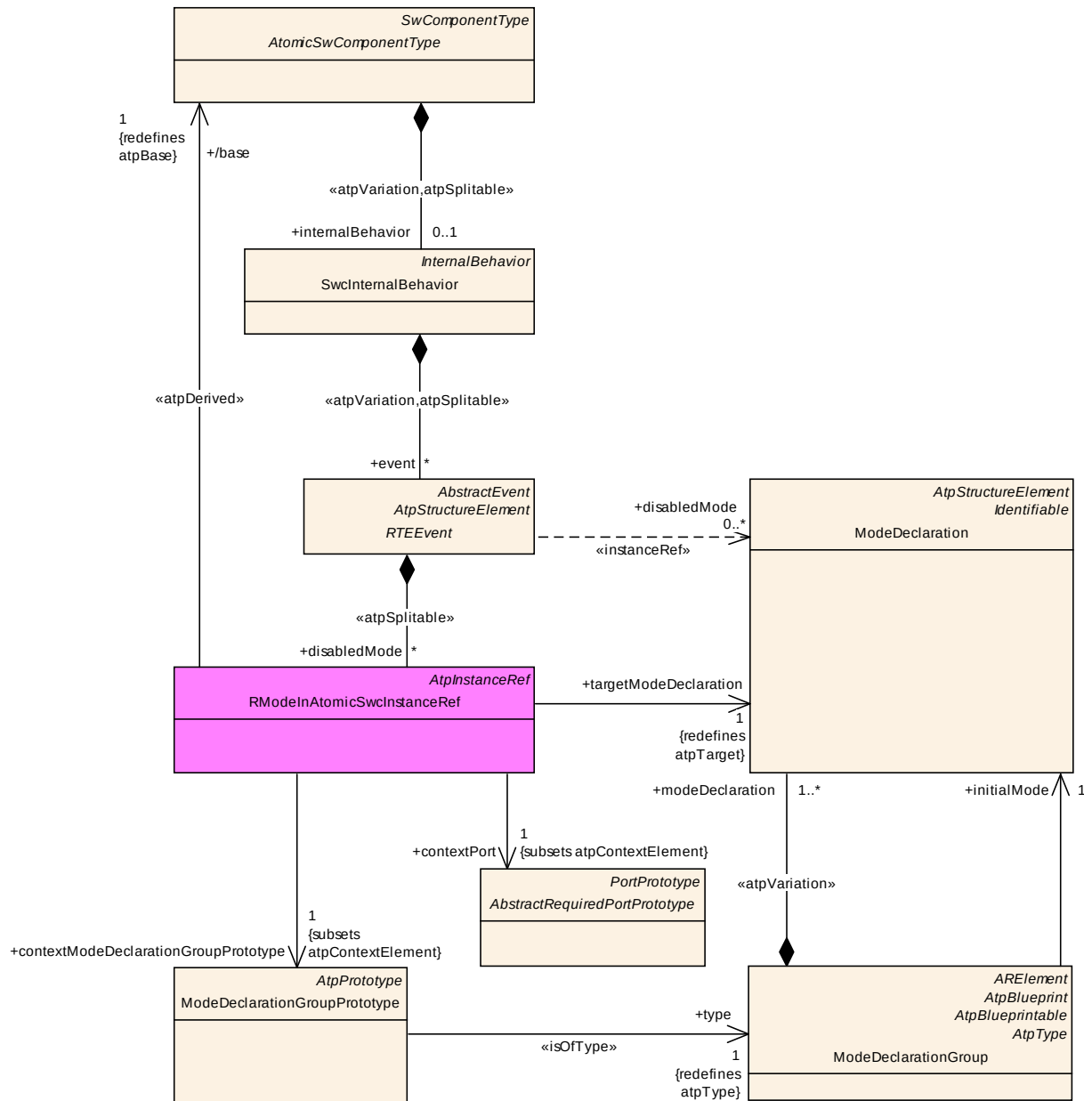
Figure D.30: Modeling of mode disabling
