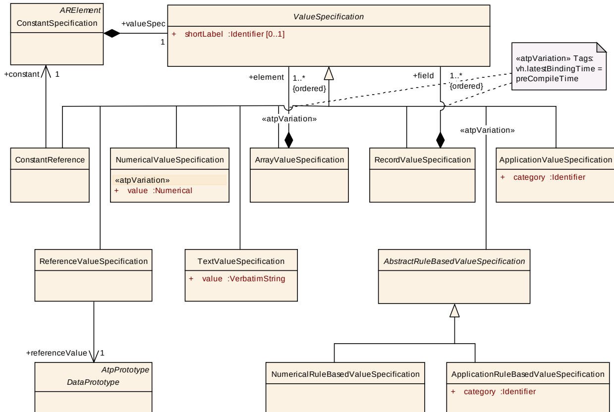
Figure 5.54: Summary of ValueSpecification
