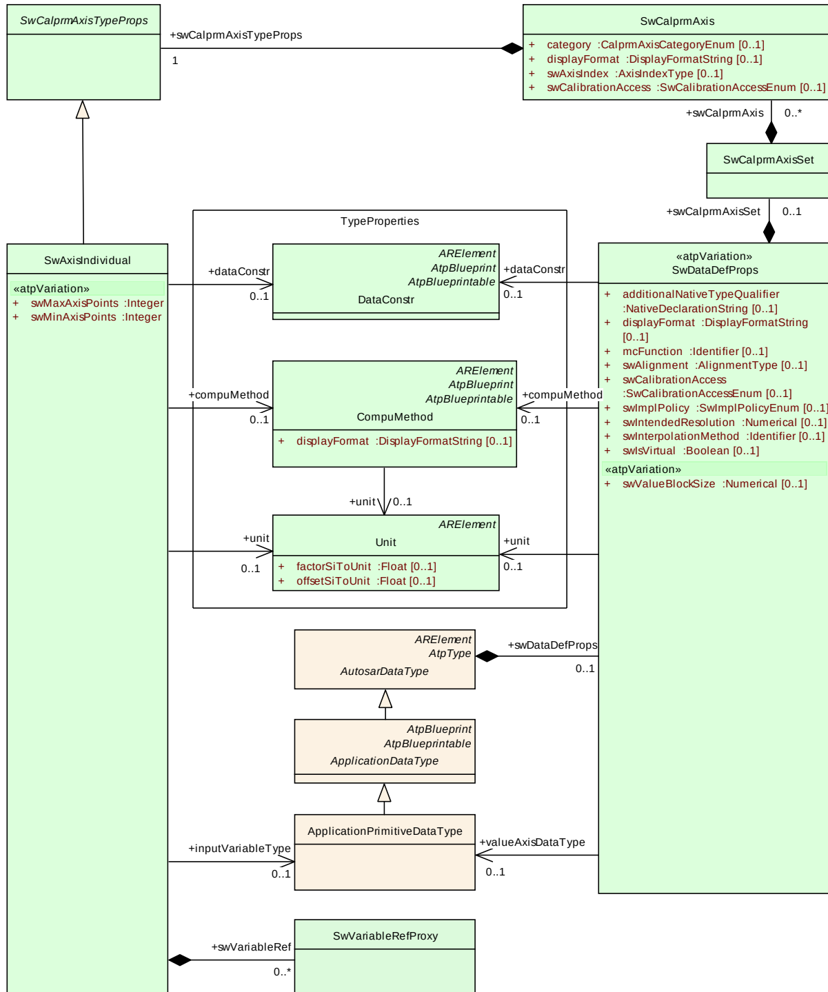
Figure 5.35: Various Attributes in the Context of SwDataDefProps
