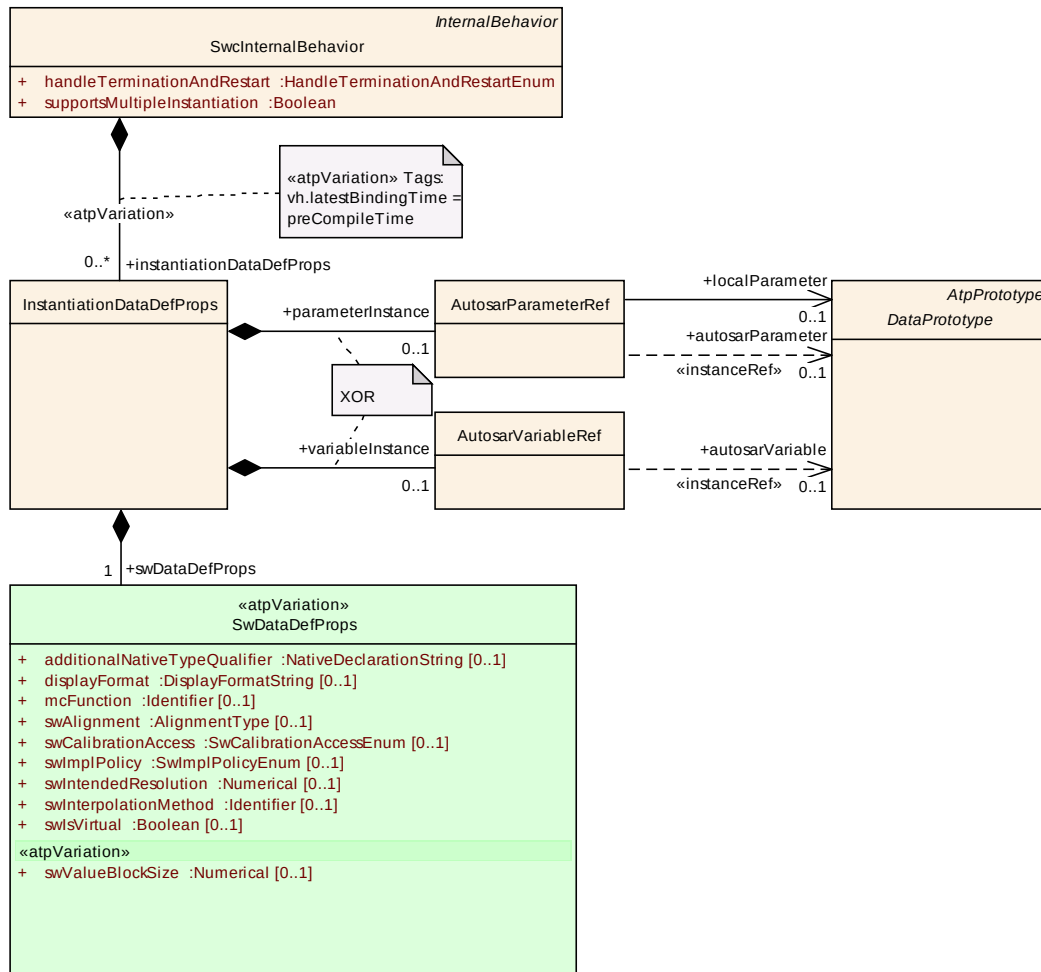
Figure 7.29: applying instantiation specific data definition properties
