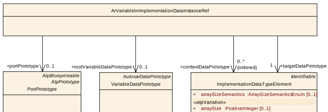
Figure 5.21: Implementation of ArVariableInImplementationDataInstanceRef
