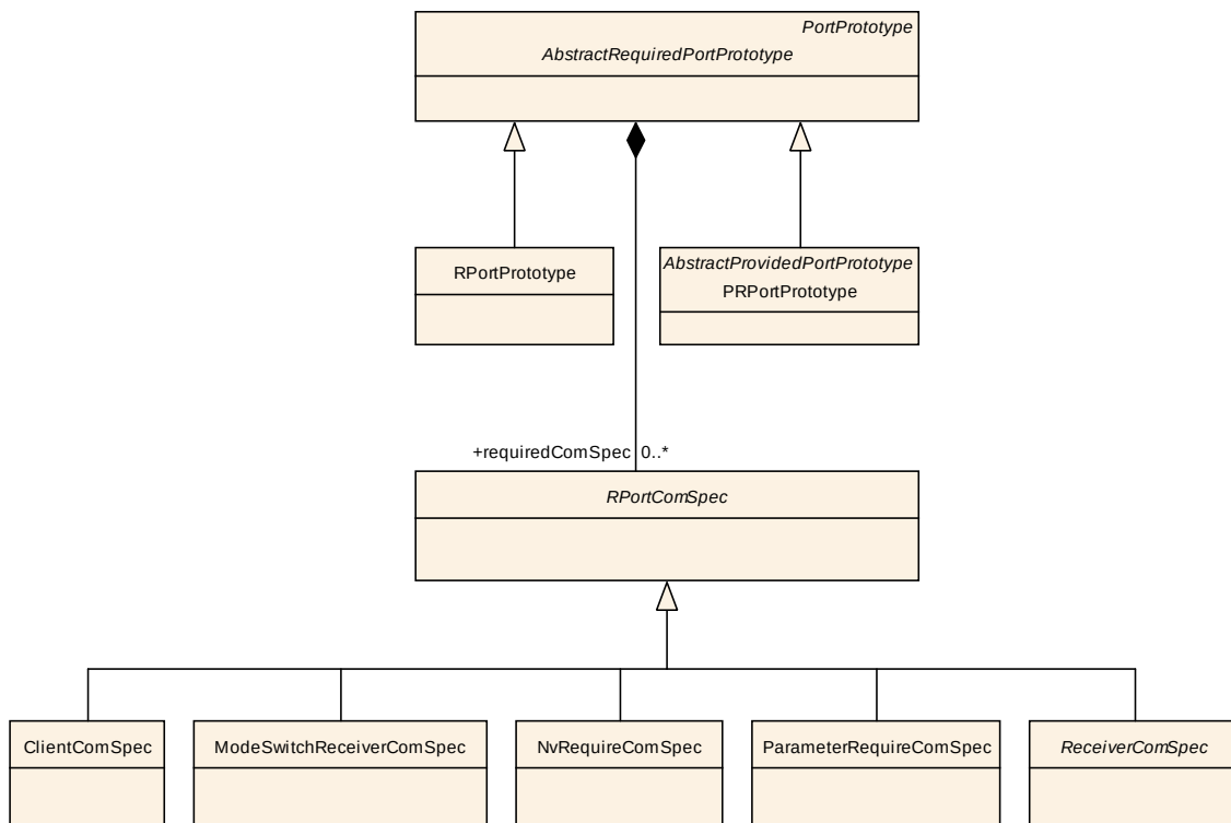
Figure 4.28: Overview of communication attributes of RPortPrototype
