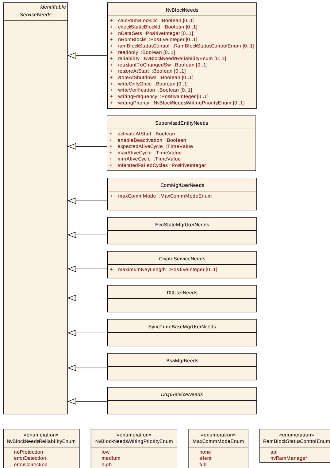
Figure 7.35: ServiceNeeds: General ServiceNeeds
