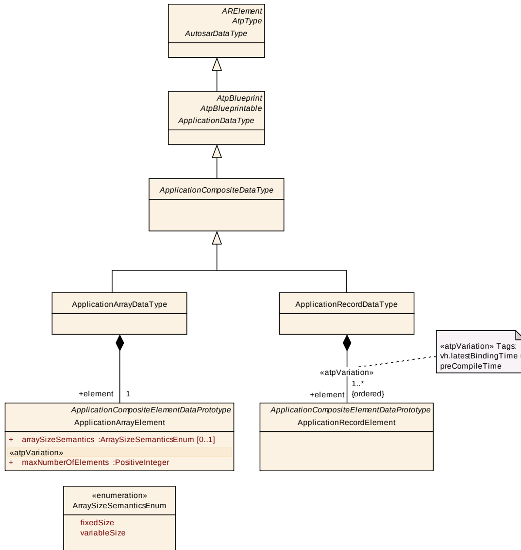
Figure 5.9: Summary of ApplicationCompositeDataType
