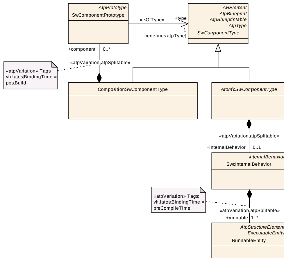
Figure 7.4: Only AtomicSwComponentTypes may have RunnableEntity s
