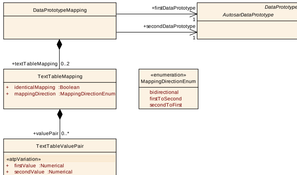
Figure 4.18: Mapping of DataPrototypes which ApplicationDataTypes referring to CompuMethods of category TEXTTABLE
