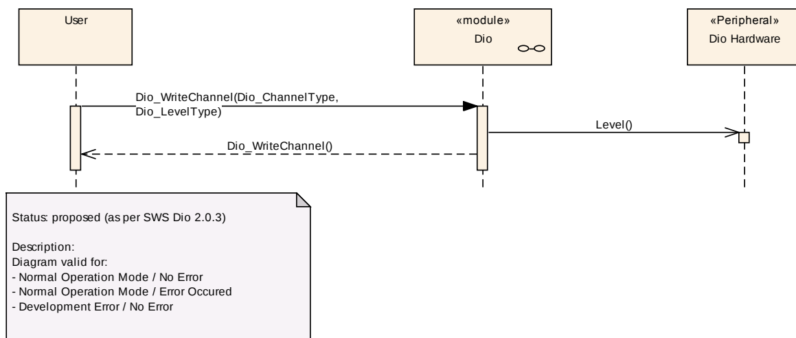
Figure 7: Write Service Sequence Chart (normal operation mode)
