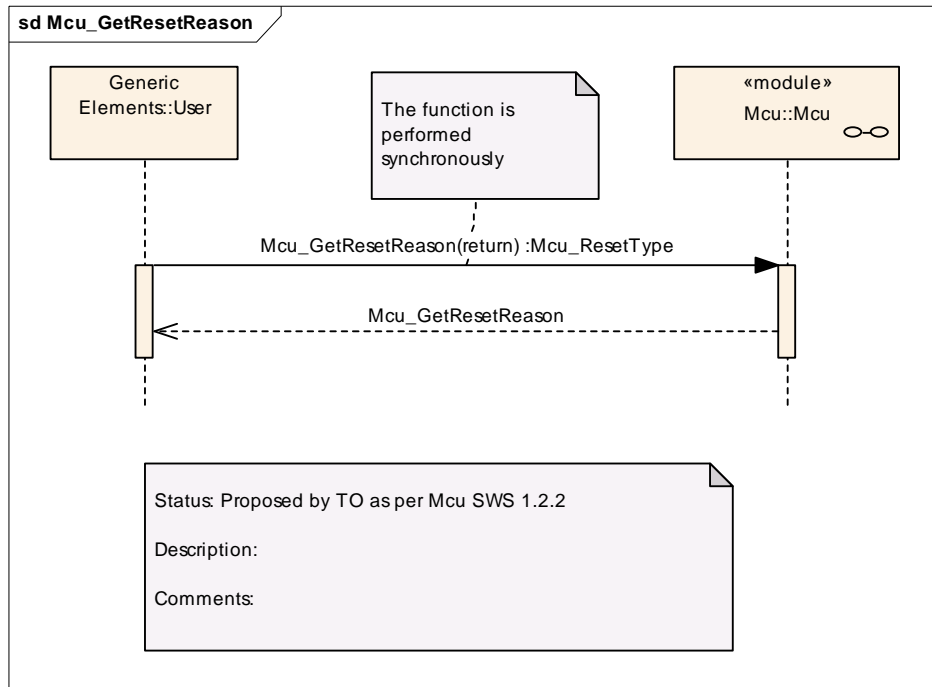
Figure 7: Sequence Diagram – MCU_GetResetReason
