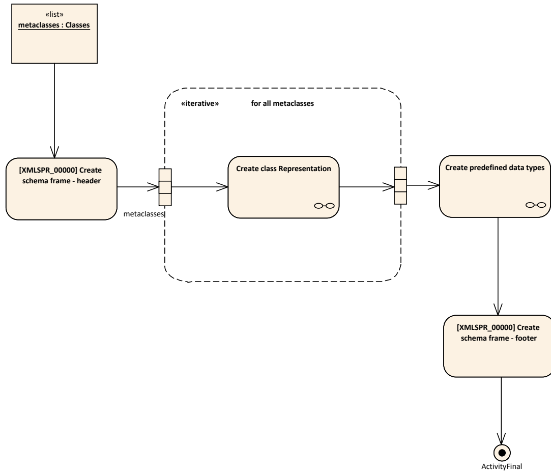
Figure 4.1: Model representation
