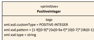
Figure 4.9: UML example - Create a custom simple type
