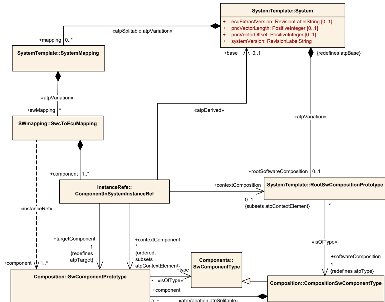
Figure 3.2: Example of an instanceRef association
