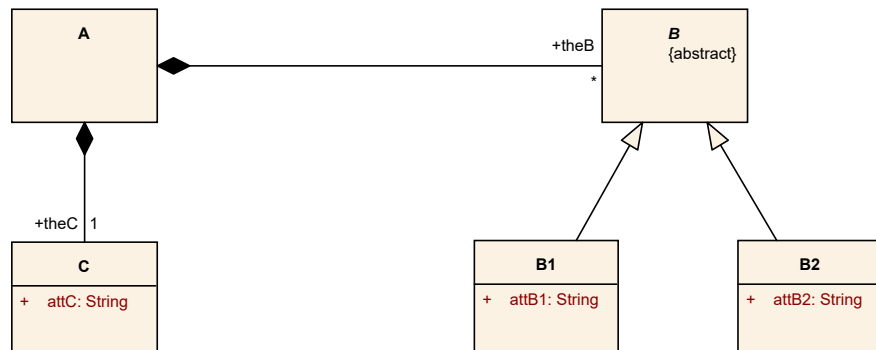
Figure 3.1: Example meta-model
