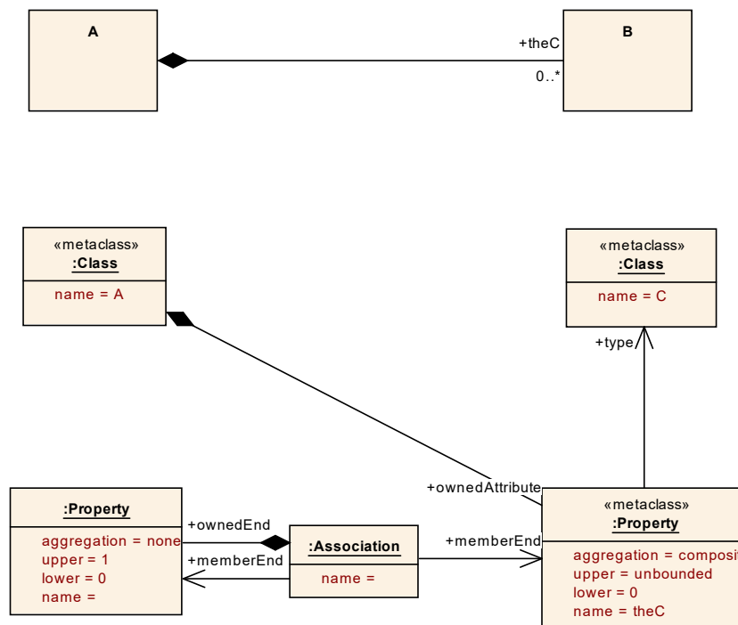
Figure 2.1: Representation of association (aggregation = composite)
