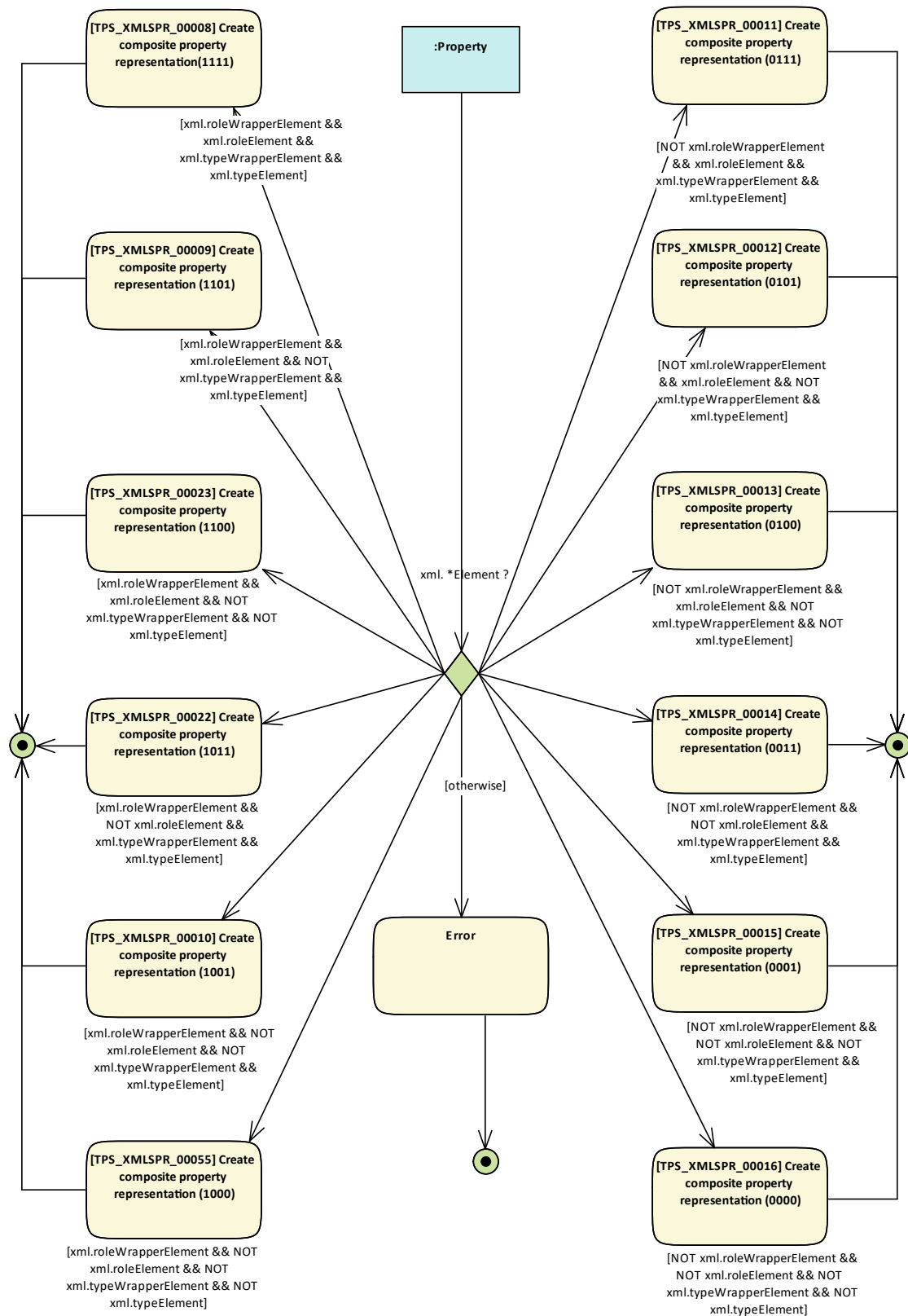
Figure 4.12: Property representation (aggregation = composite)
