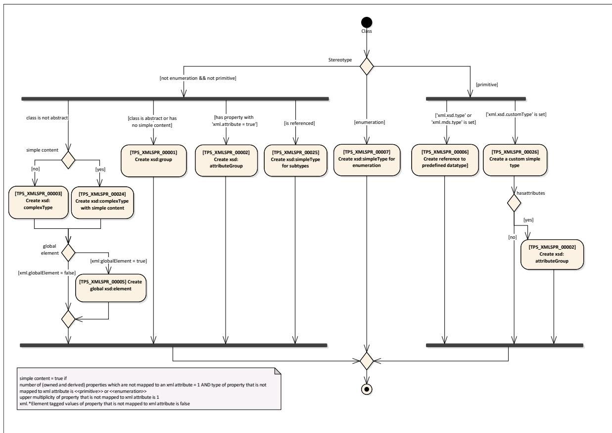
Figure 4.2: Class representation
