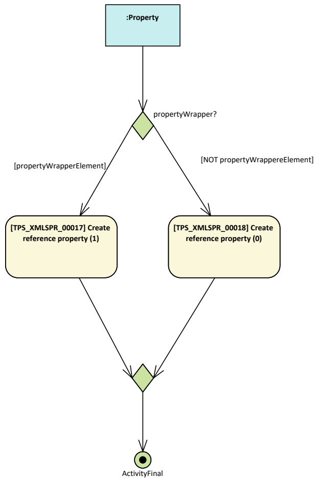
Figure 4.15: Property representation (aggregation = none)
