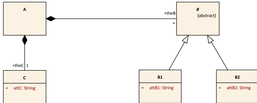
Figure 4.13: Example meta-model of composite property
