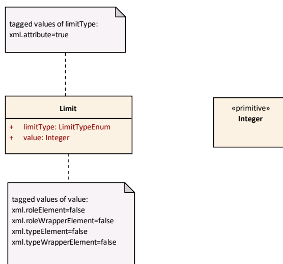
Figure 4.6: UML example - Create xsd:complexType with simple content
