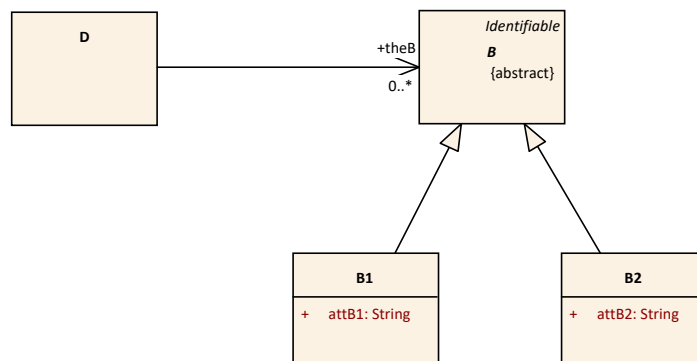
Figure 4.16: Example meta-model using a reference
