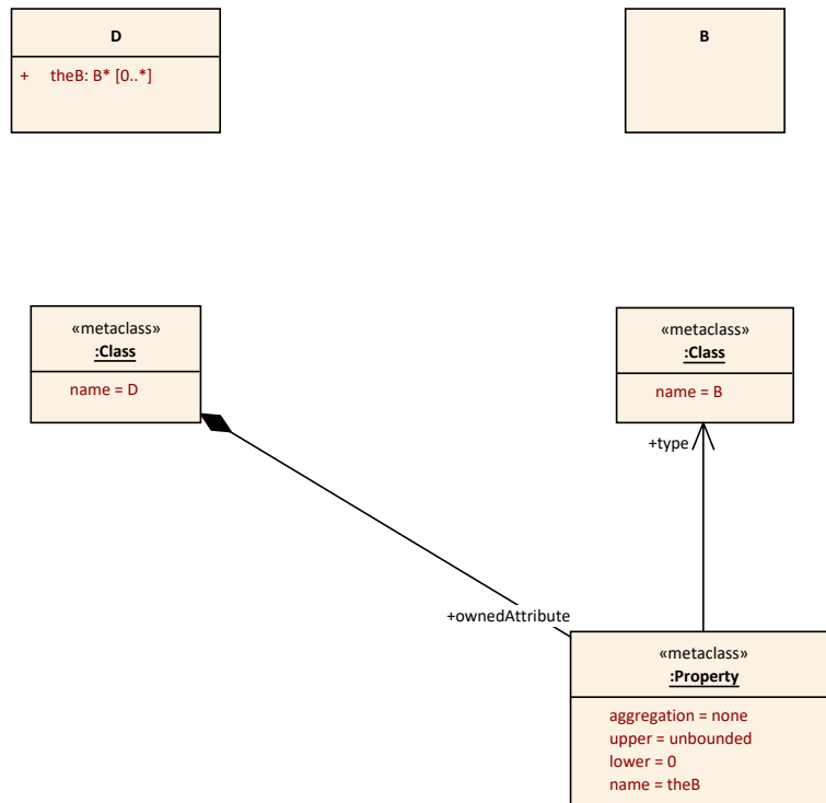
Figure 2.4: Representation of attribute (aggregation = none)
