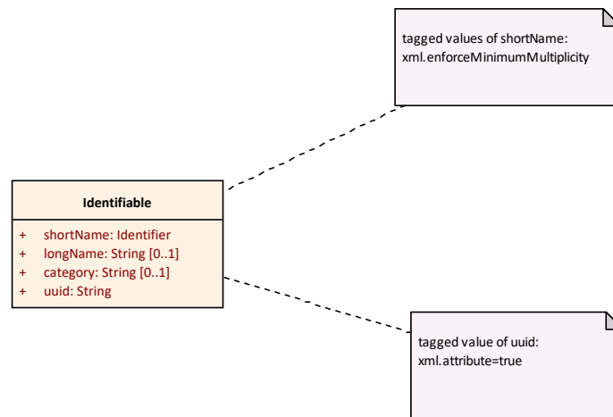
Figure 4.11: UML example - Create xsd:attribute
