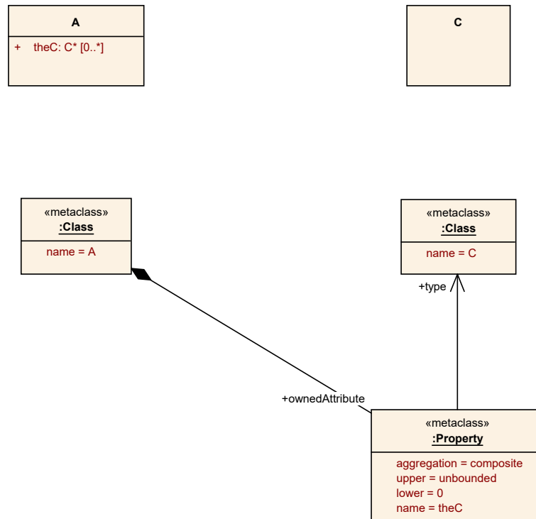
Figure 2.2: Representation of attribute (aggregation = composite)
