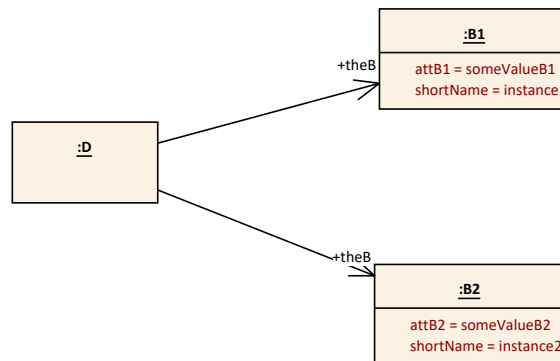
Figure 4.17: Example instance of reference
