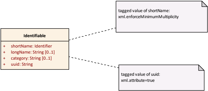
Figure 4.3: UML example - Create xsd:group
