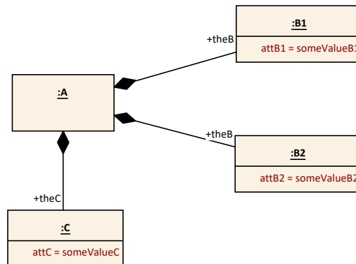
Figure 4.14: Example instance of composite property
