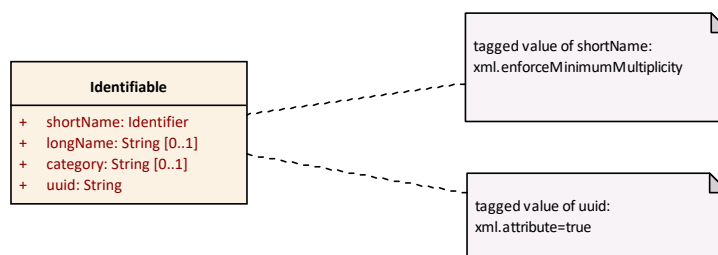
Figure 4.4: UML example - Create xsd:attributeGroup
