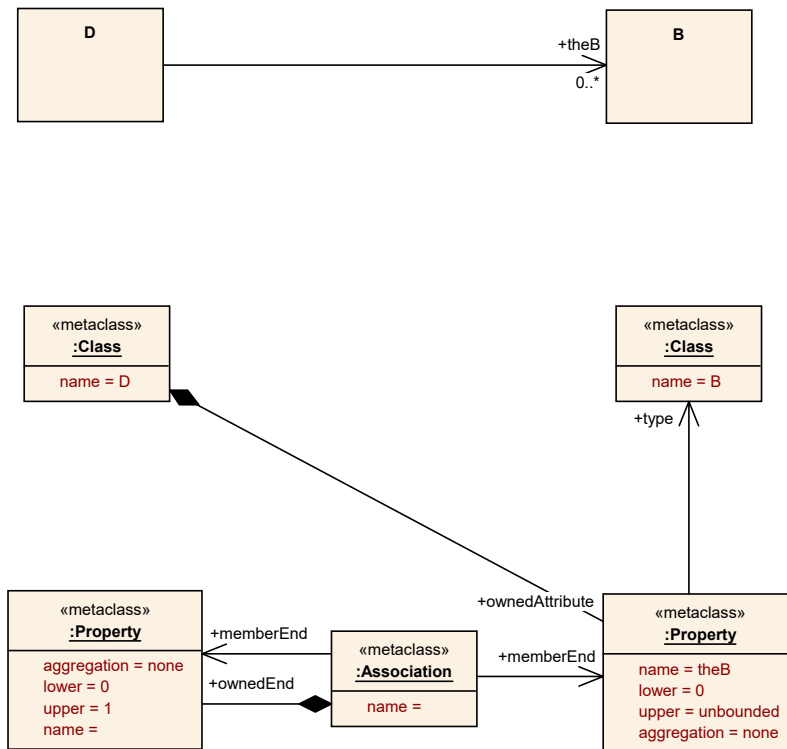
Figure 2.3: Representation of association (aggregation = none)
