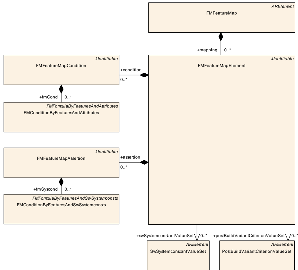
Figure 6.1: Class FMFeatureMap
