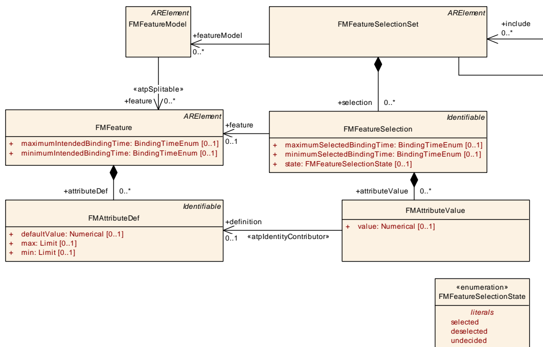
Figure 5.1: Class FMFeatureSelectionSet
