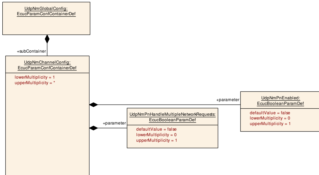
Figure 10.5: UdpNmPnConfig
