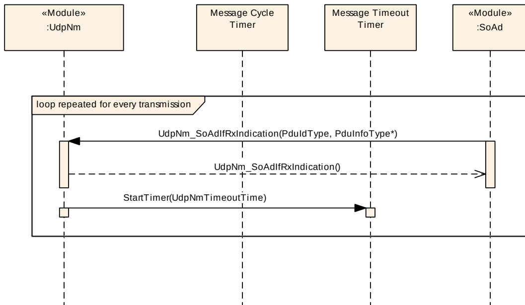
Figure 9.2: Sequence diagram - PDU reception.
