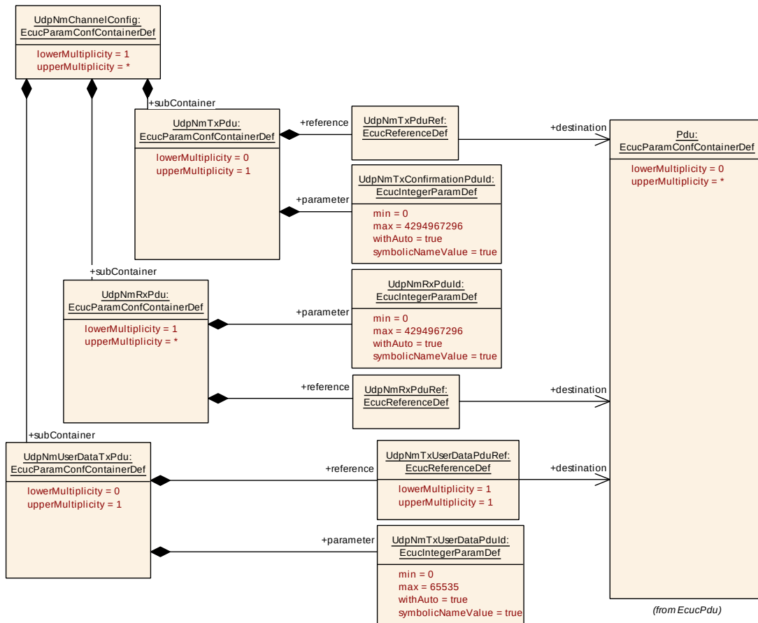
Figure 10.3: UdpNmChannelConfig - part 2
