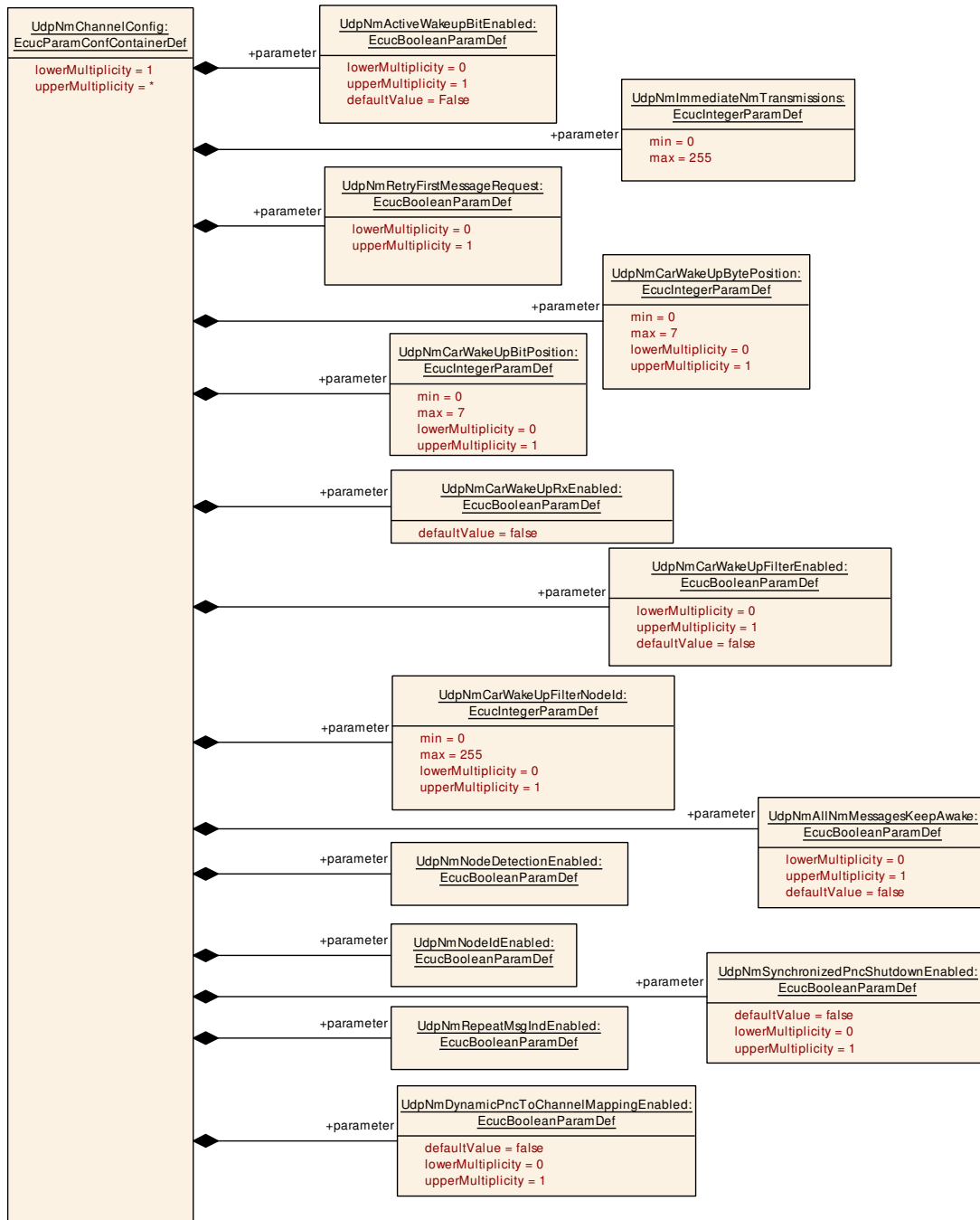
Figure 10.4: UdpNmChannelConfig - part 3
