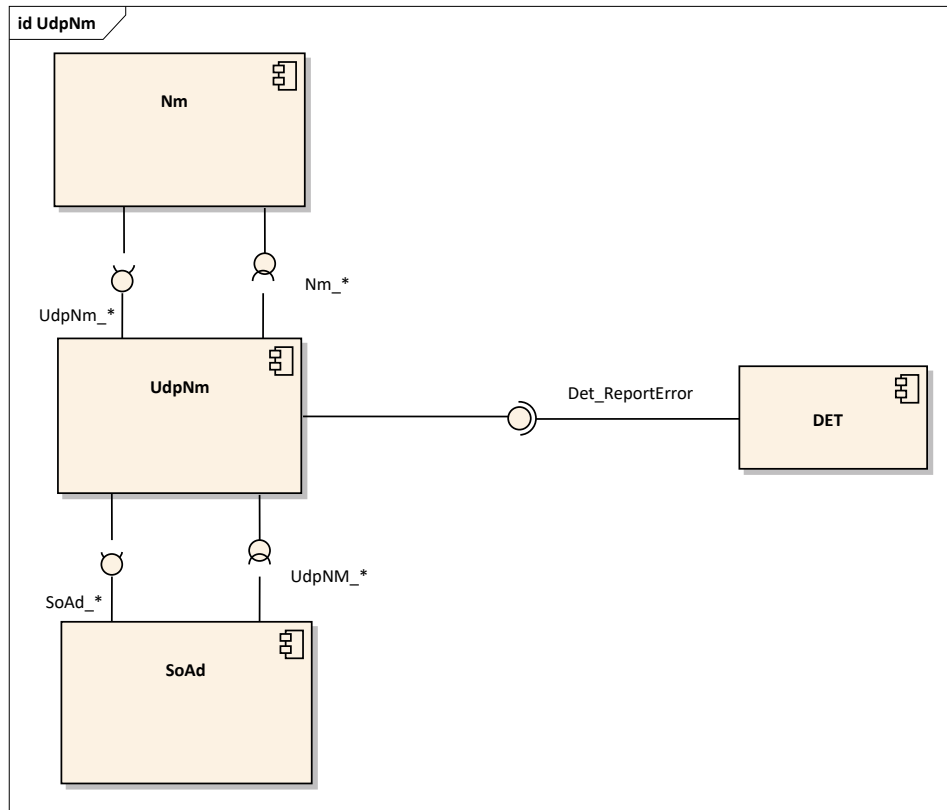
Figure 5.1: Dependencies on other modules.
