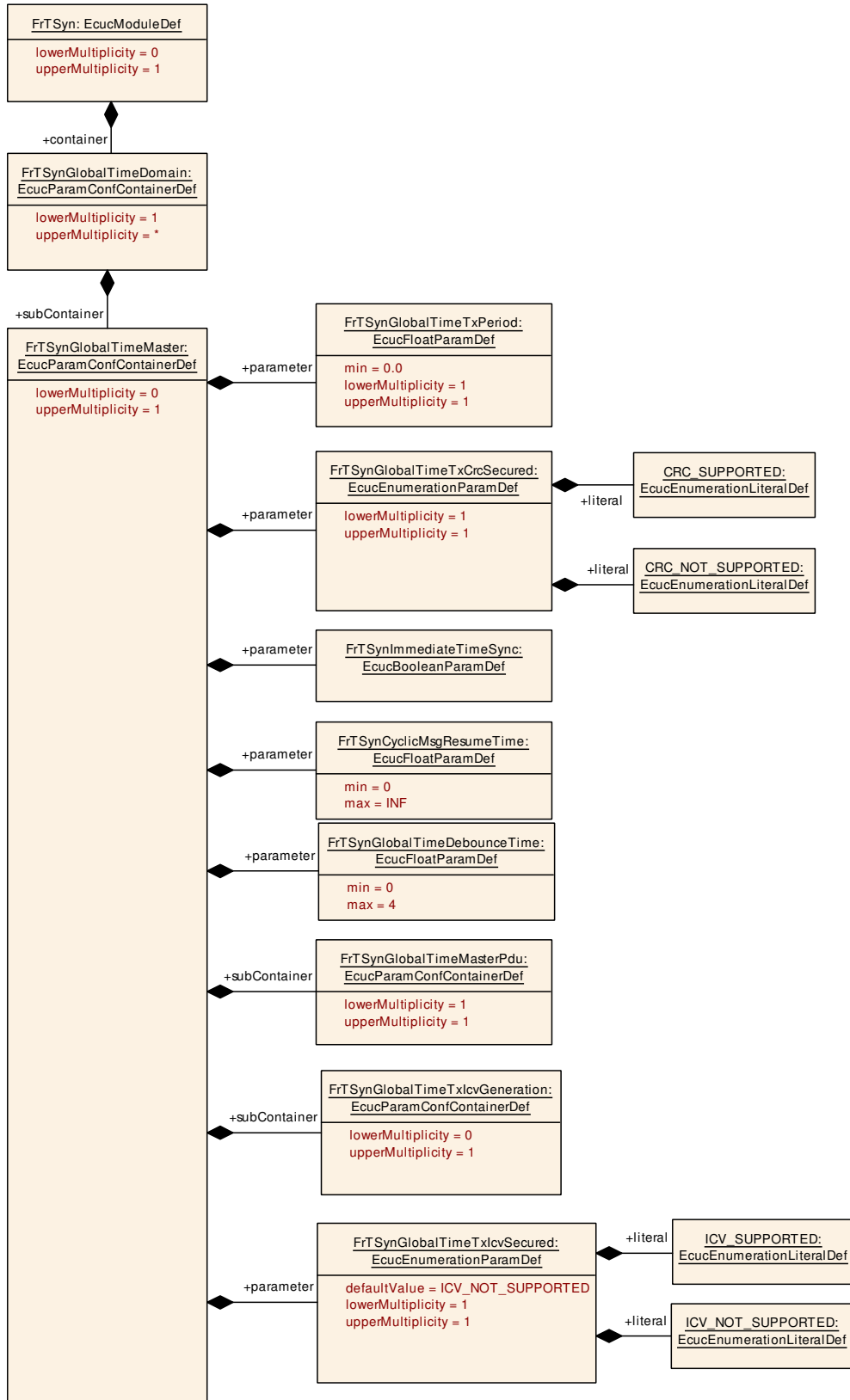
Figure 10.4: FrTSynGlobalTimeMaster
