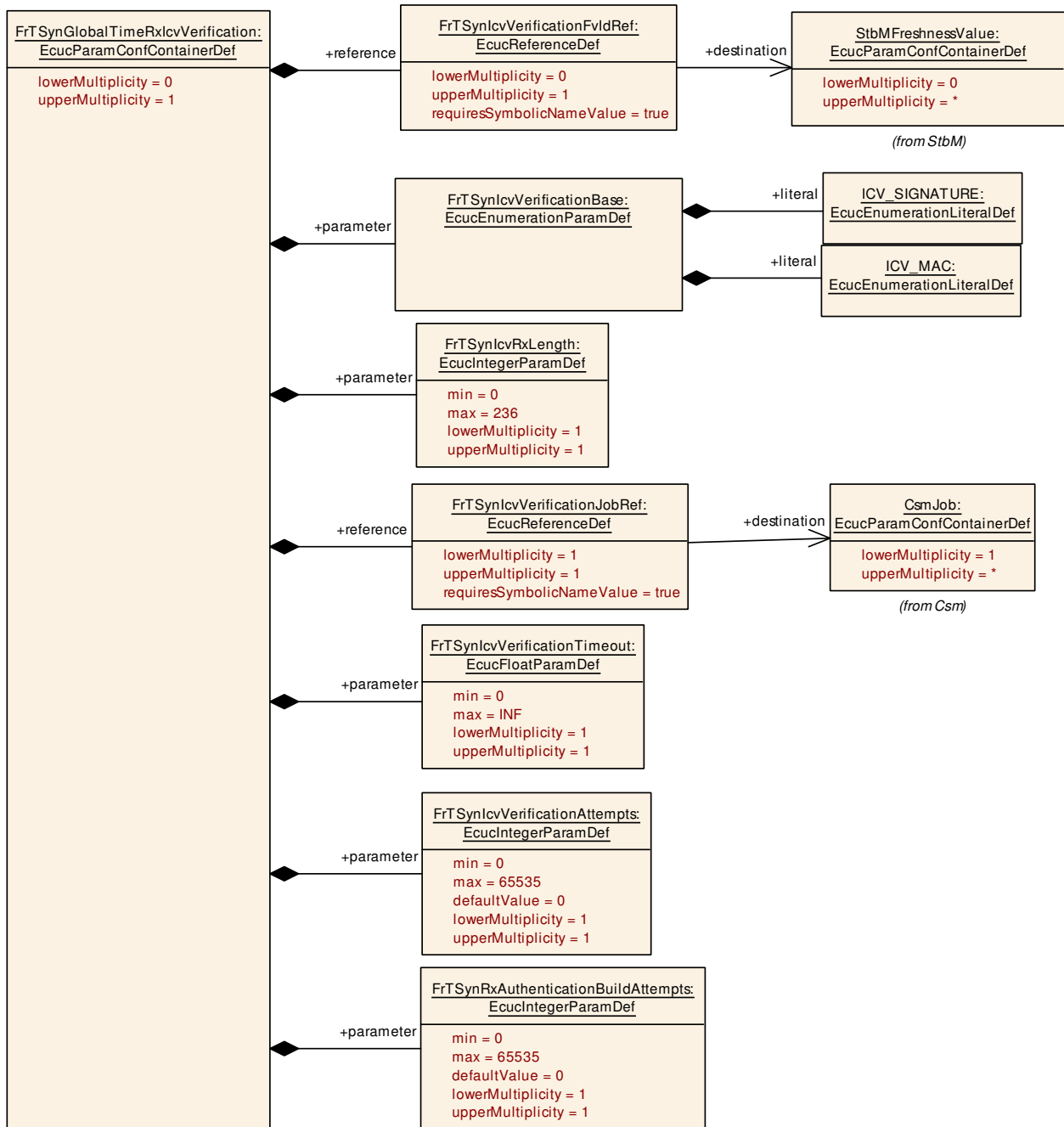
Figure 10.8: FrTSynGlobalTimeRxIcvVerification
