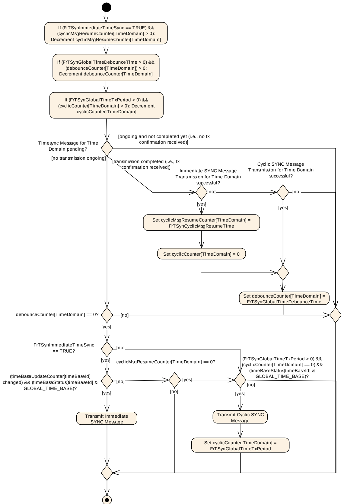
Figure 7.2: Timesync Message Transmission
