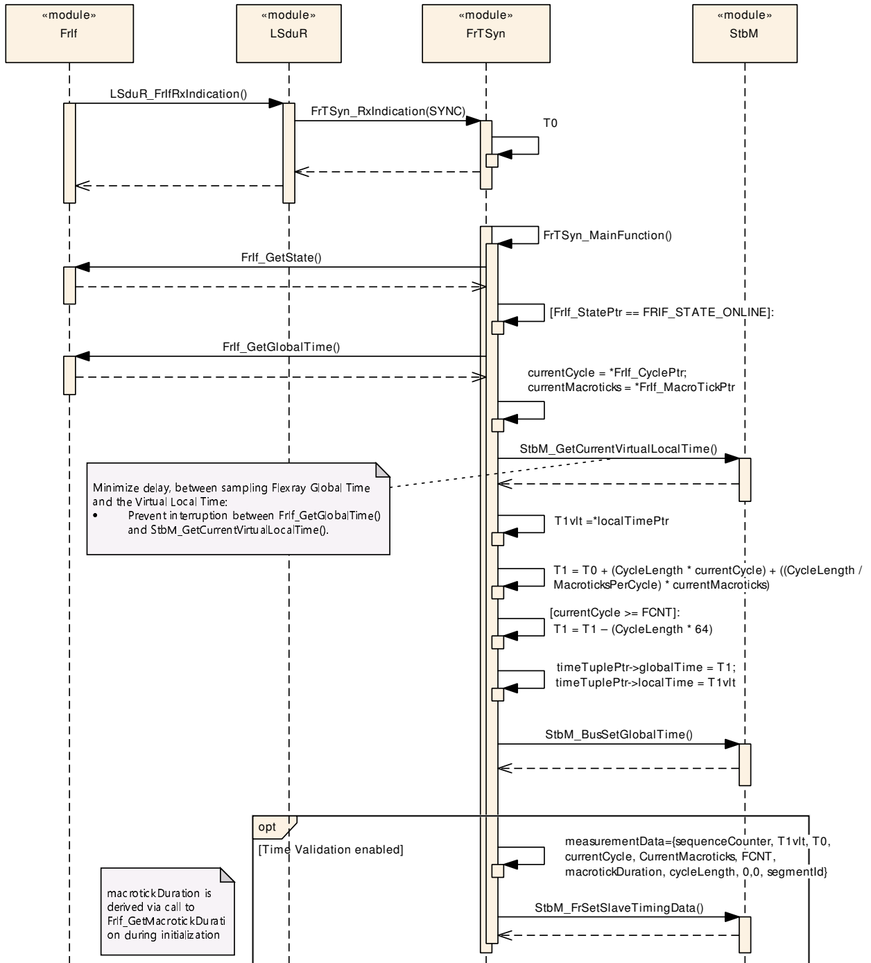
Figure 9.2: FlexRay Time Synchronization (Time Slave)
