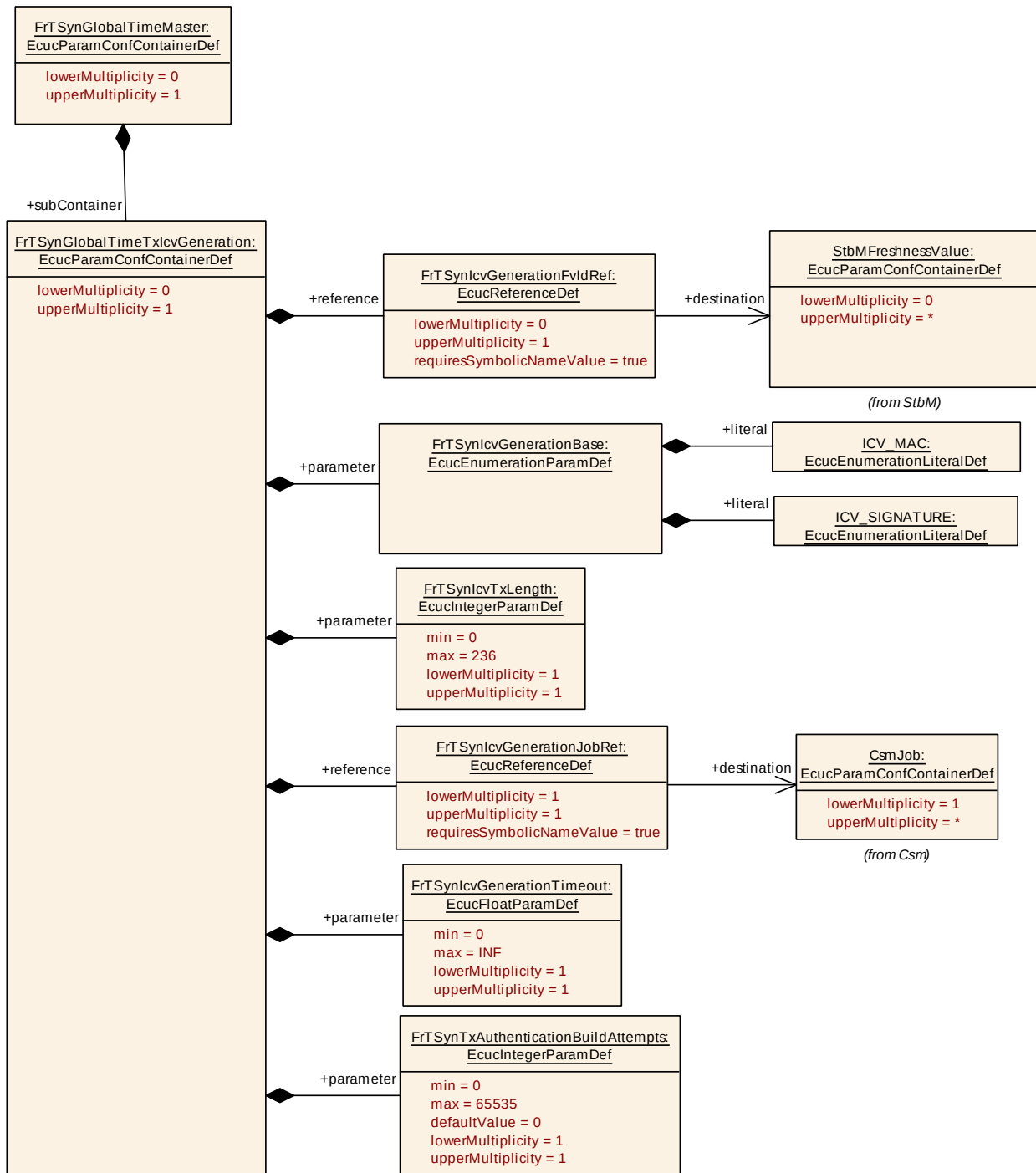
Figure 10.6: FrTSynGlobalTimeTxIcvGeneration
