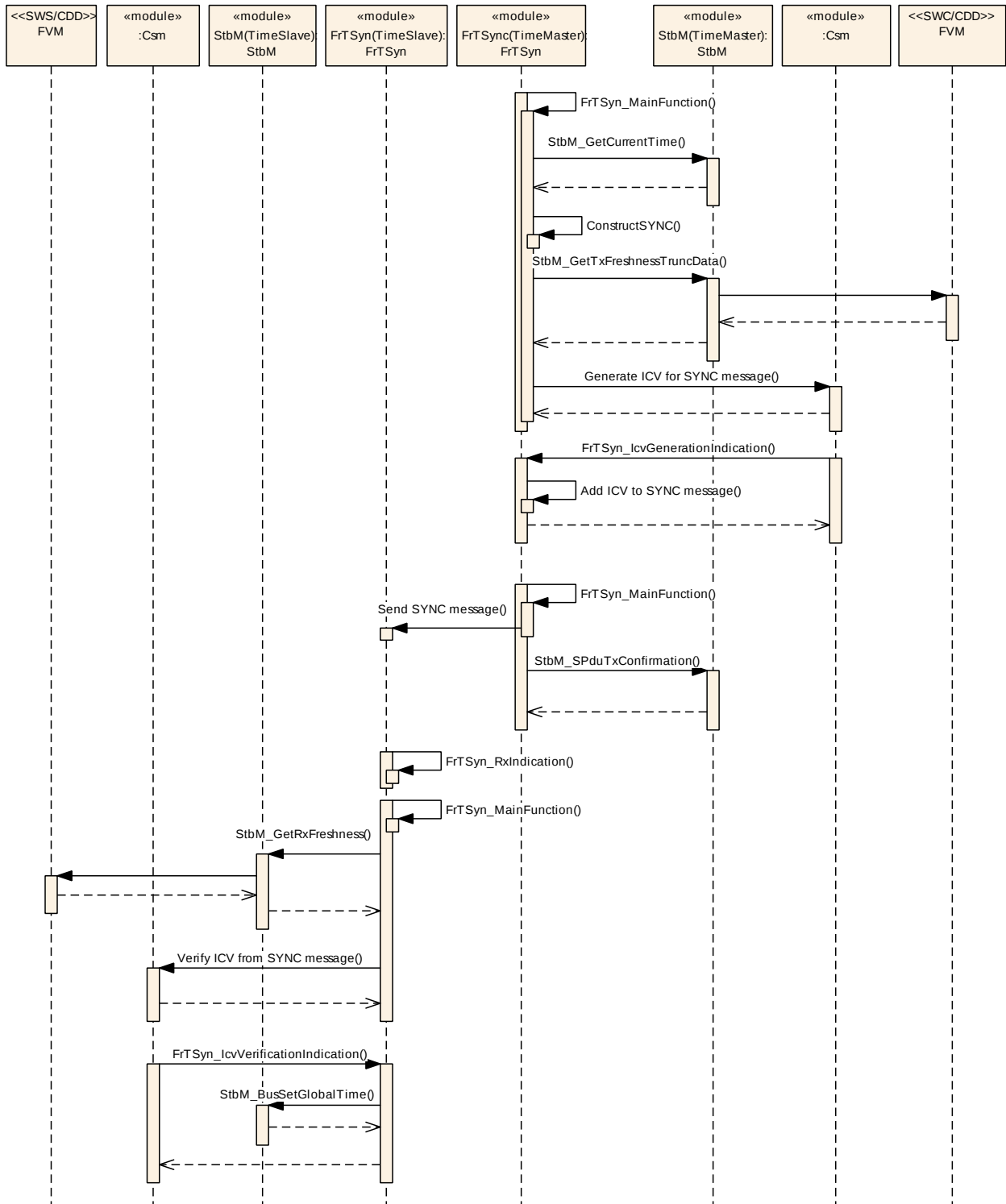
Figure 9.3: FlexRay Secure Time Synchronization Sequence
