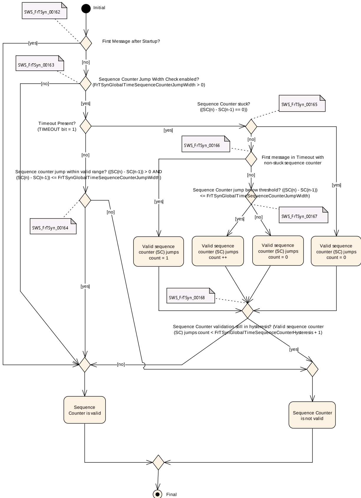
Figure 7.3: Sequence Counter Validation
