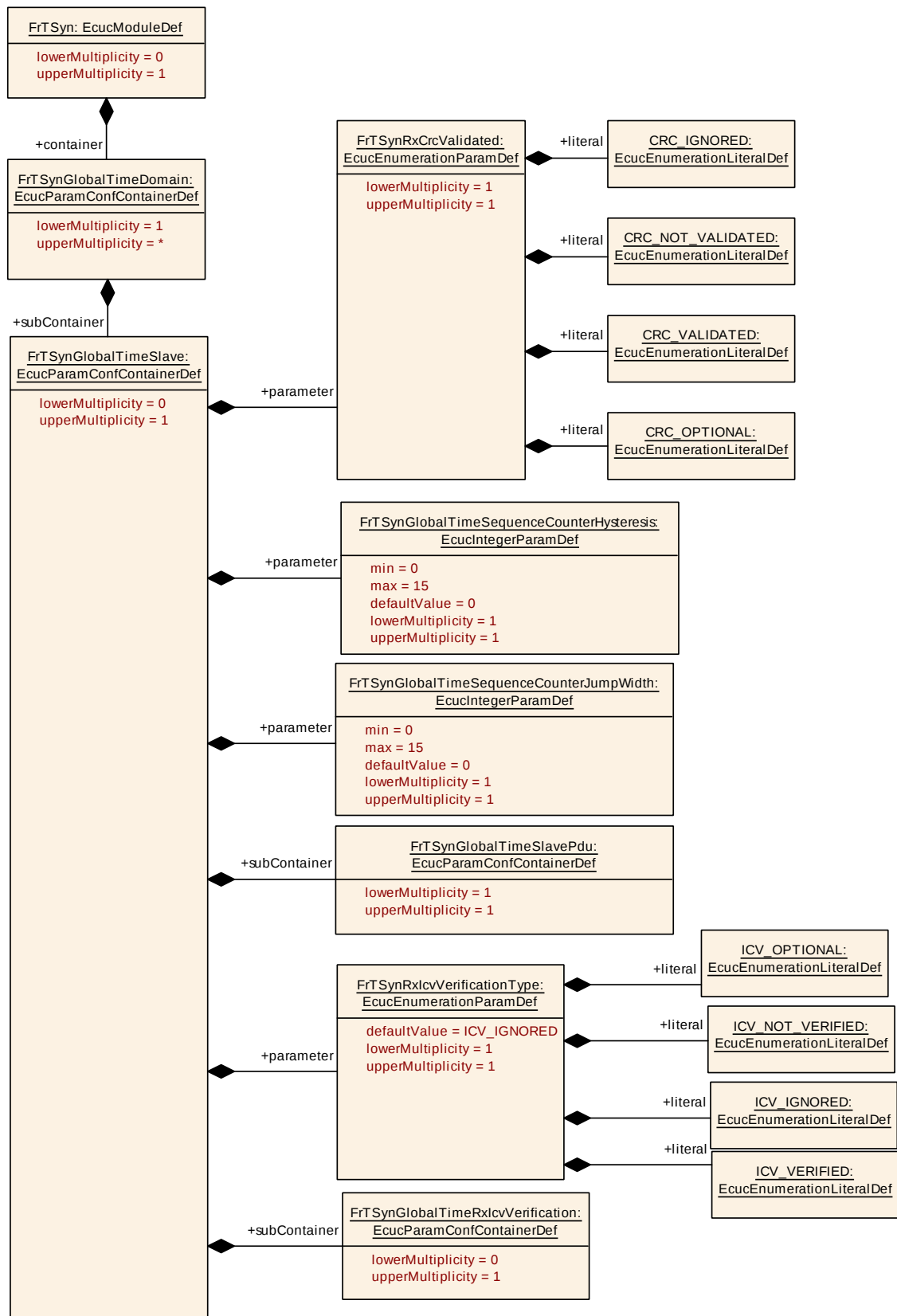
Figure 10.7: FrTSynGlobalTimeSlave
