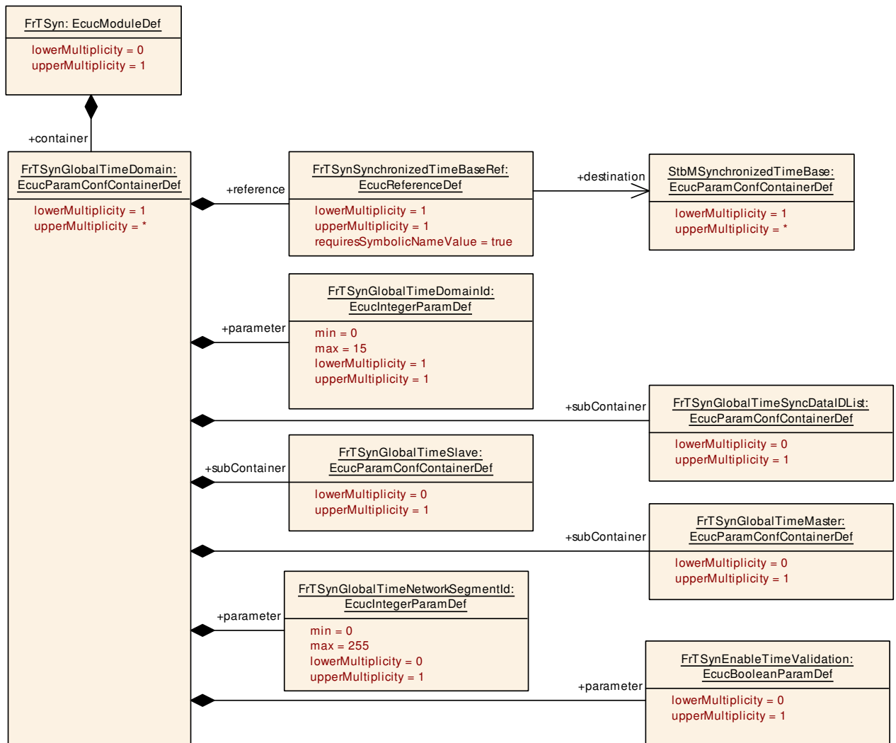
Figure 10.2: FrTSynGlobalTimeDomain
