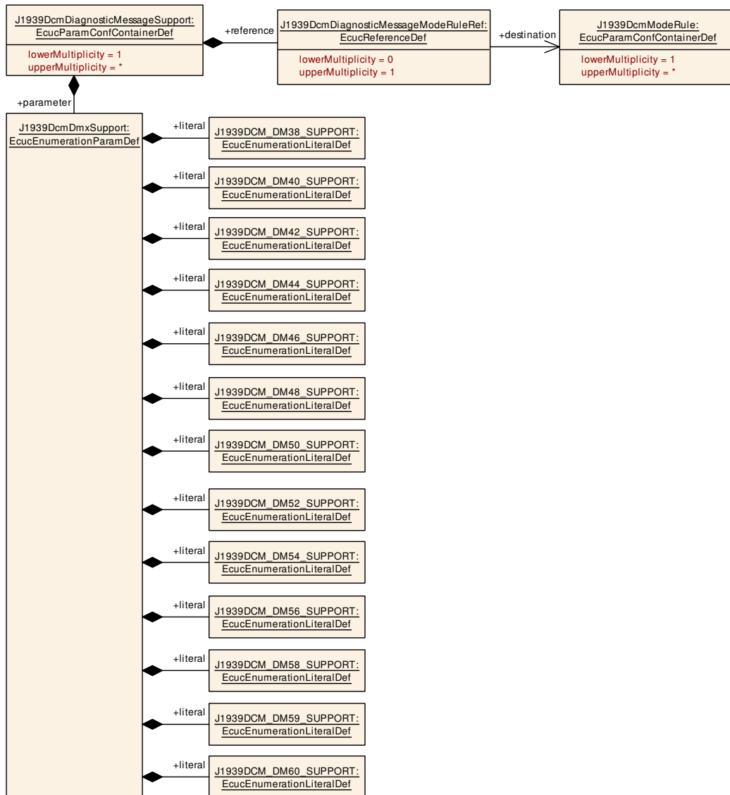
Figure 10.7: Configuration of Diagnostic Messages - Part 2
