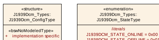
Figure 8.1: Overview of Type Definitions
