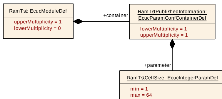
Figure 10.7: RamTstPublishedInformation
