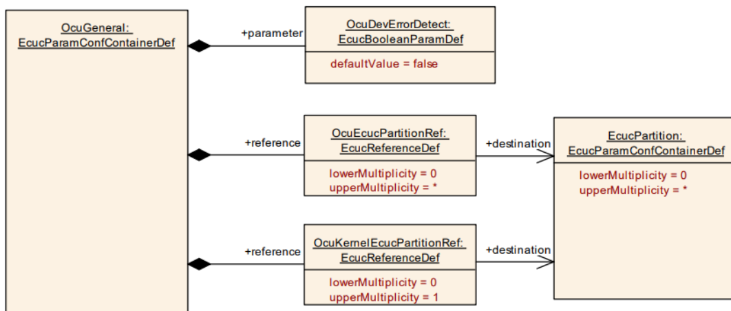
Figure 10.2: Ocu General Configuration
