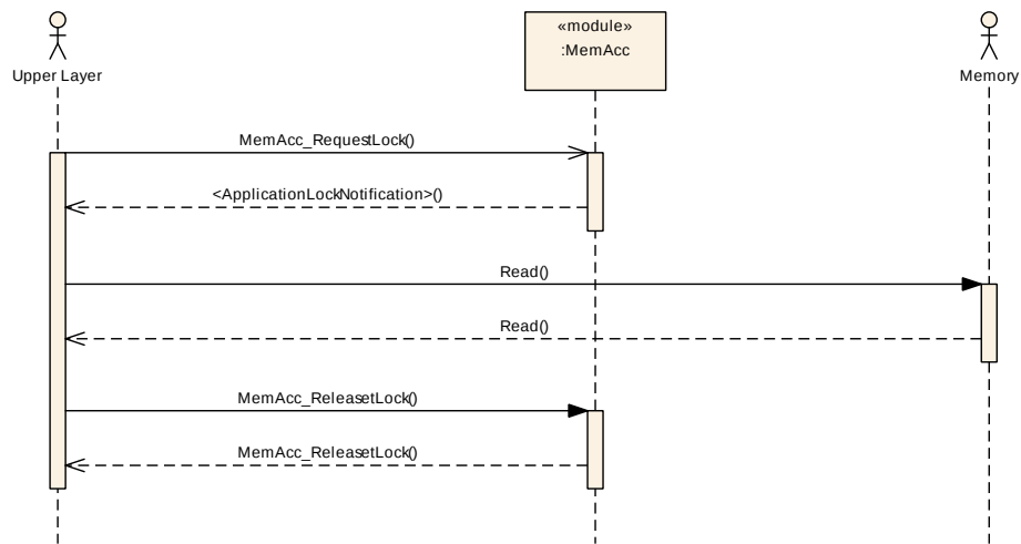
Figure 9.7: Example Lock/Unlock Sequence
