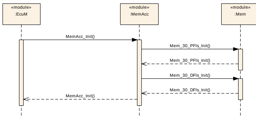
Figure 9.3: Mem Driver Initialization by MemAcc
