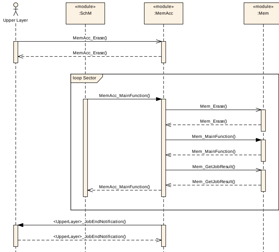
Figure 9.2: Job Handling with Job End Notification
