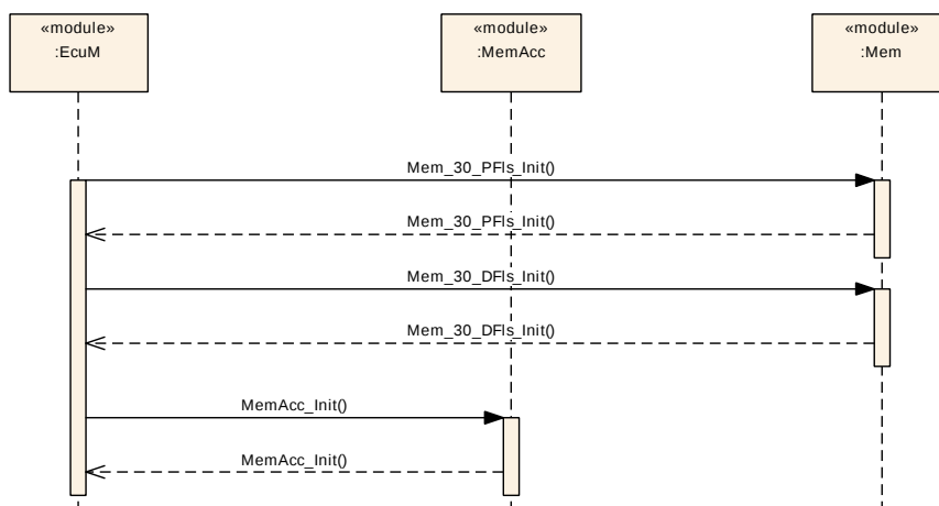
Figure 9.4: Mem Driver initialization by EcuM
