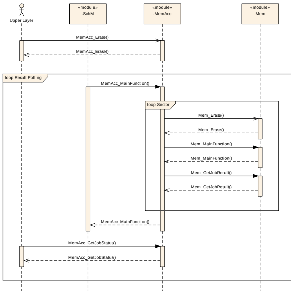
Figure 9.5: Mem Driver Scheduling by MemAcc
