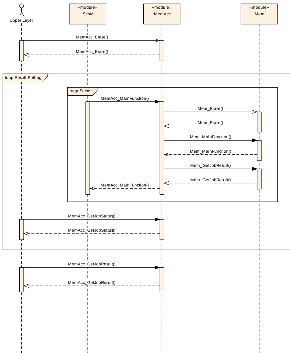
Figure 9.1: Job Handling with Result Polling
