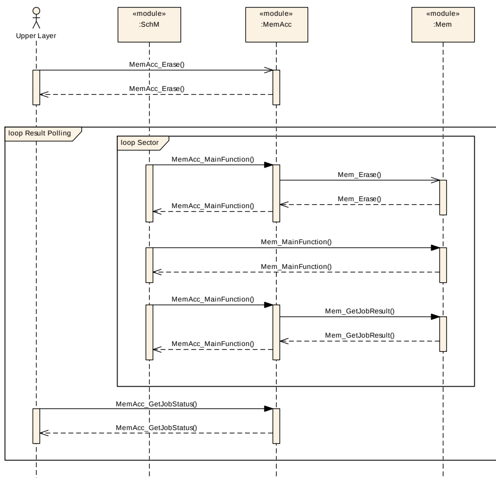
Figure 9.6: Mem Driver Scheduling by SchM
