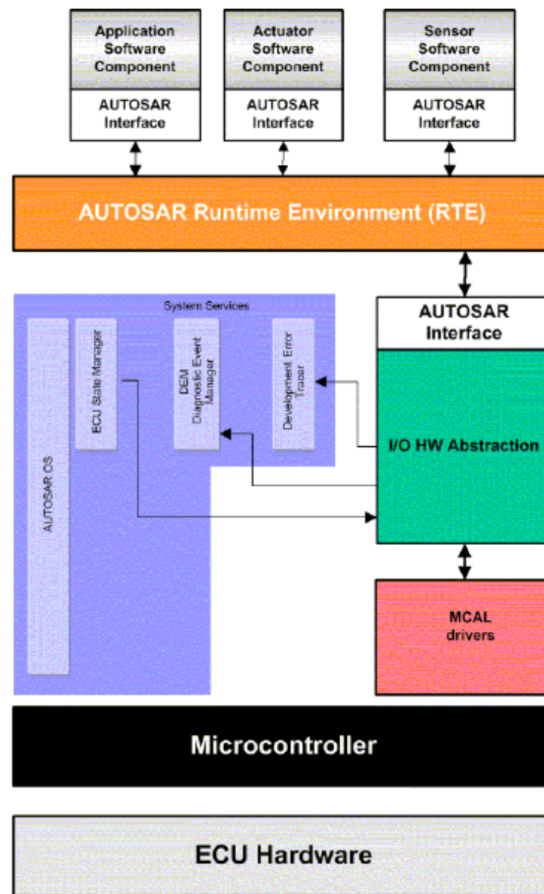
Figure 5.3: Interfaces with system services
