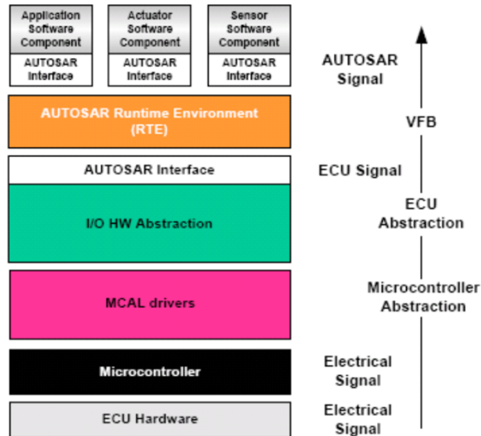
Figure 7.2: ECU signals
