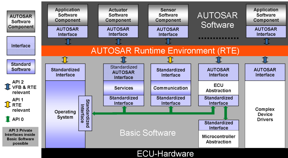
Figure 7.1: AUTOSAR architecture
