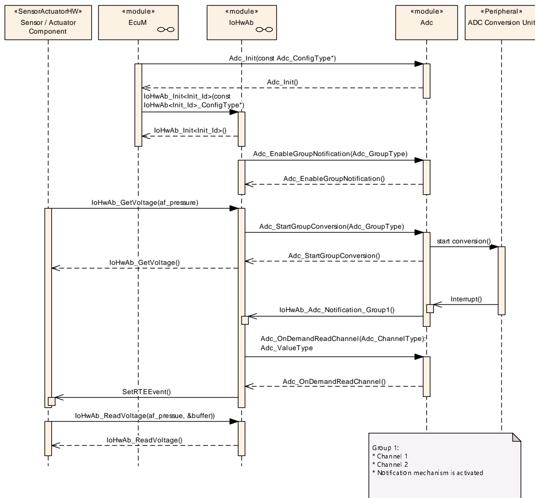
Figure 9.1: Sequence diagram - ADC conversion
