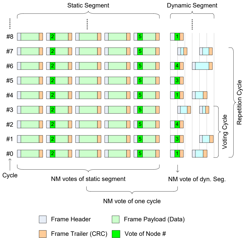
Figure 10.9: Example of NM-Vote in dynamic and static segment
