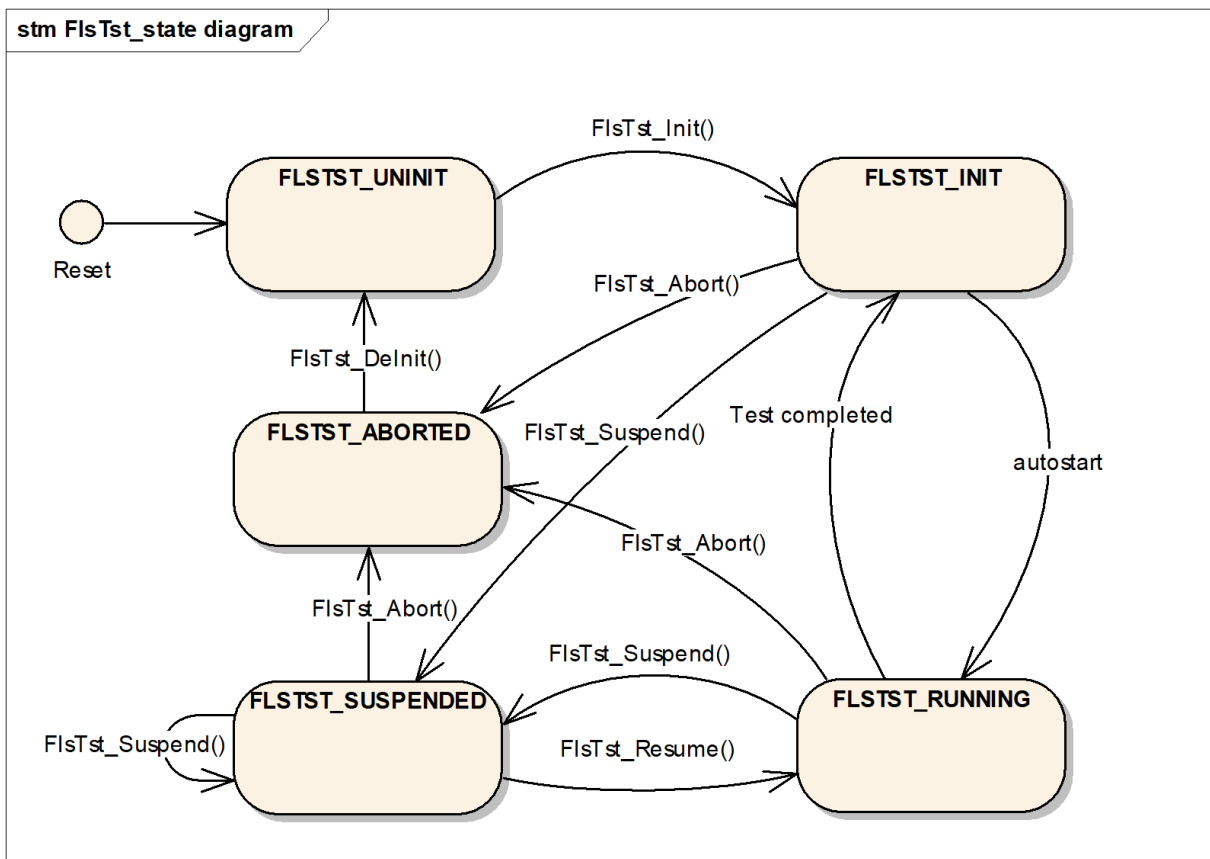
Figure 7.3: State Diagram - Background mode
