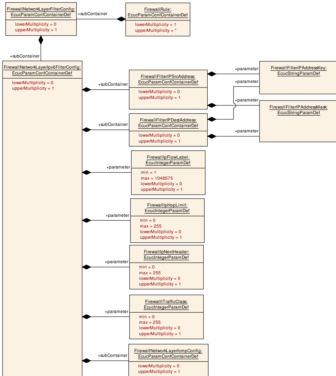
Figure 10.8: IPv6 configuration
