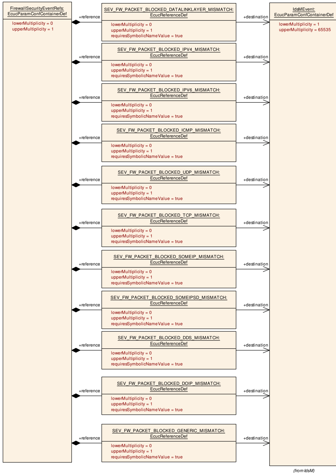
Figure 10.18: Security Events
