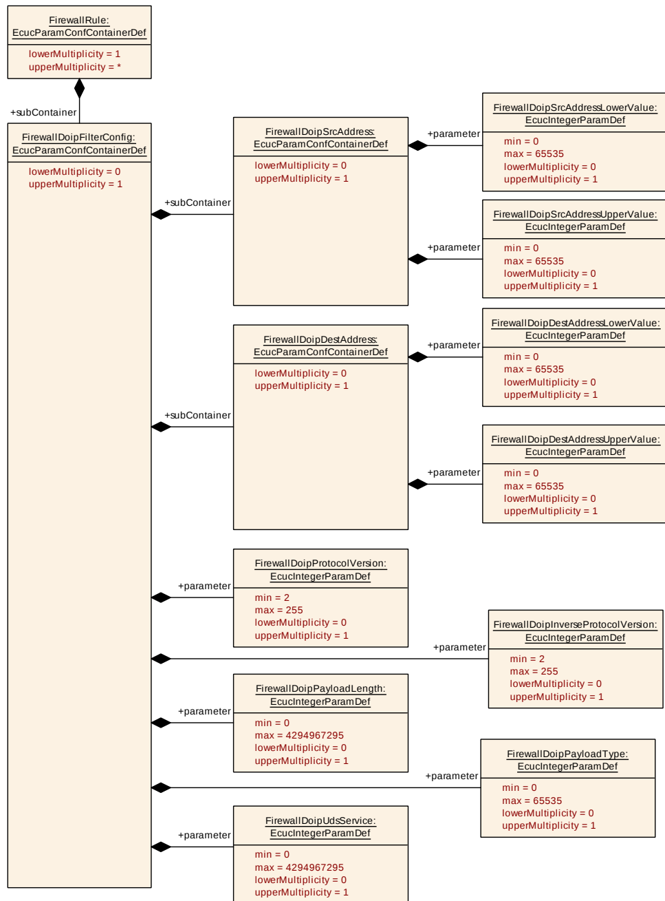
Figure 10.15: DoIP configuration
