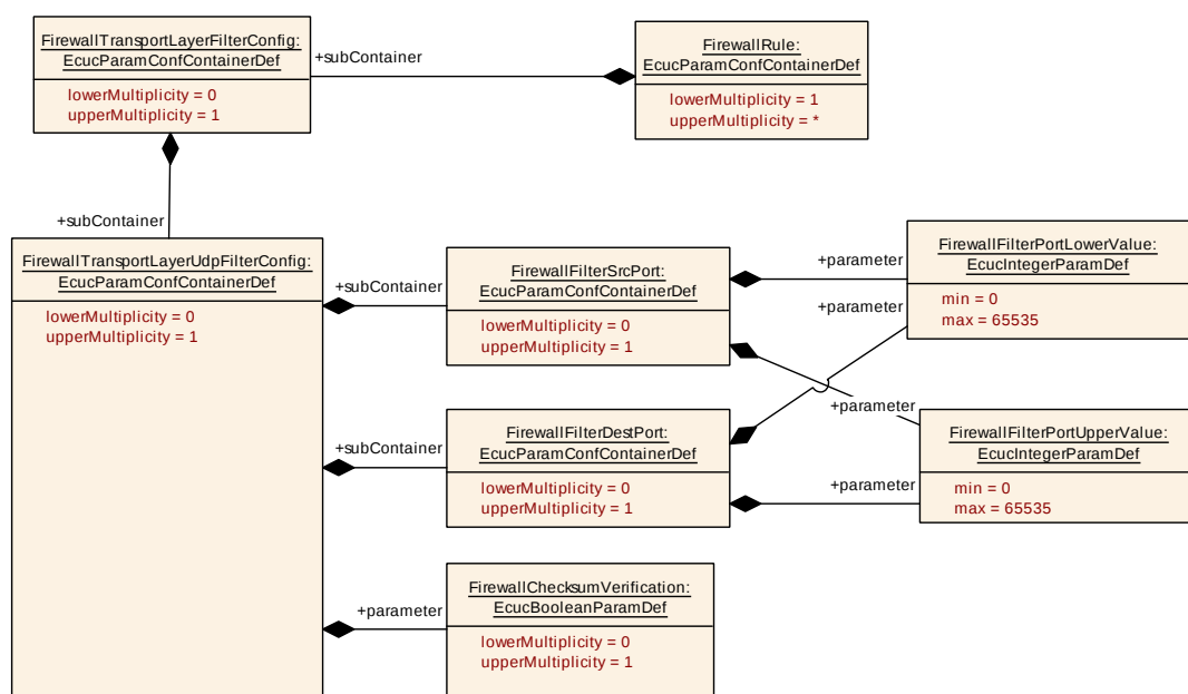
Figure 10.11: UDP configuration
