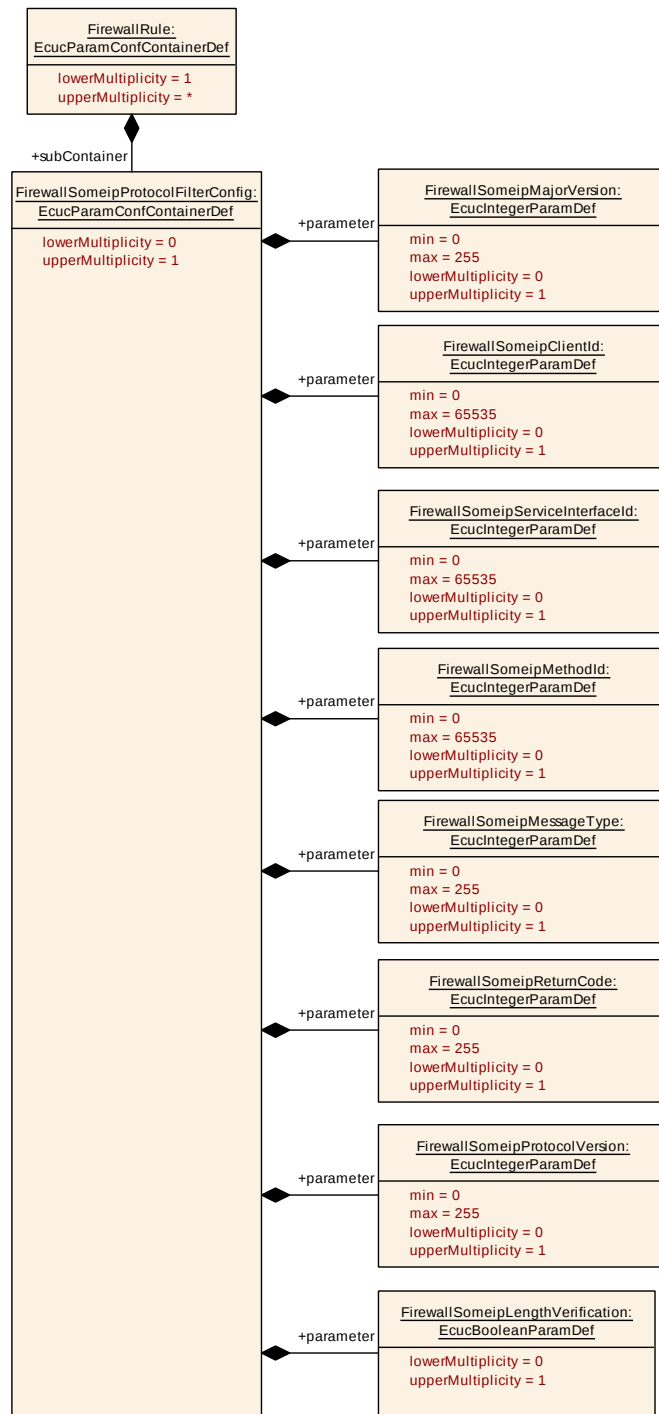
Figure 10.12: SOME/IP configuration
