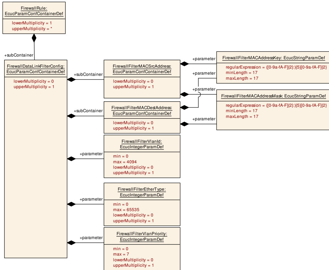
Figure 10.6: Data link layer configuration
