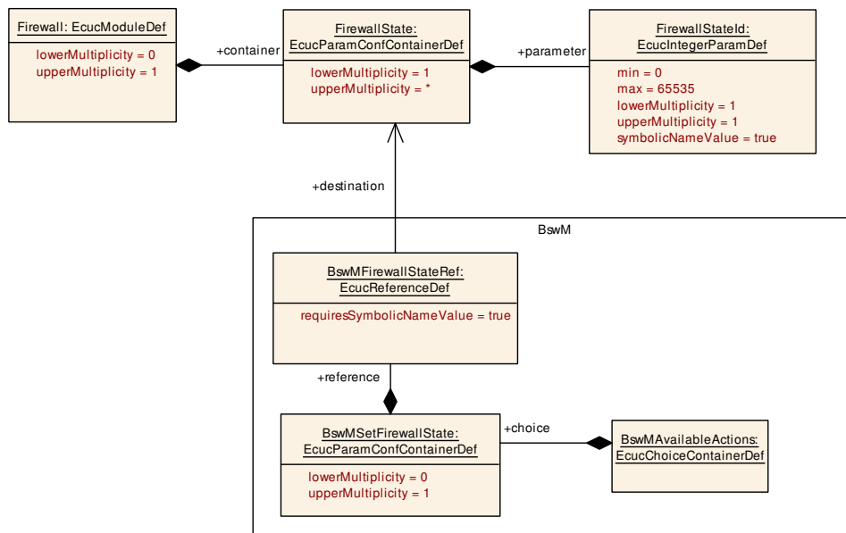
Figure 10.3: Connection to the BswM
