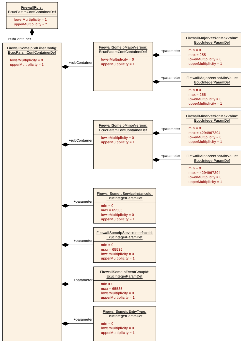
Figure 10.13: SOME/IP-SD configuration
