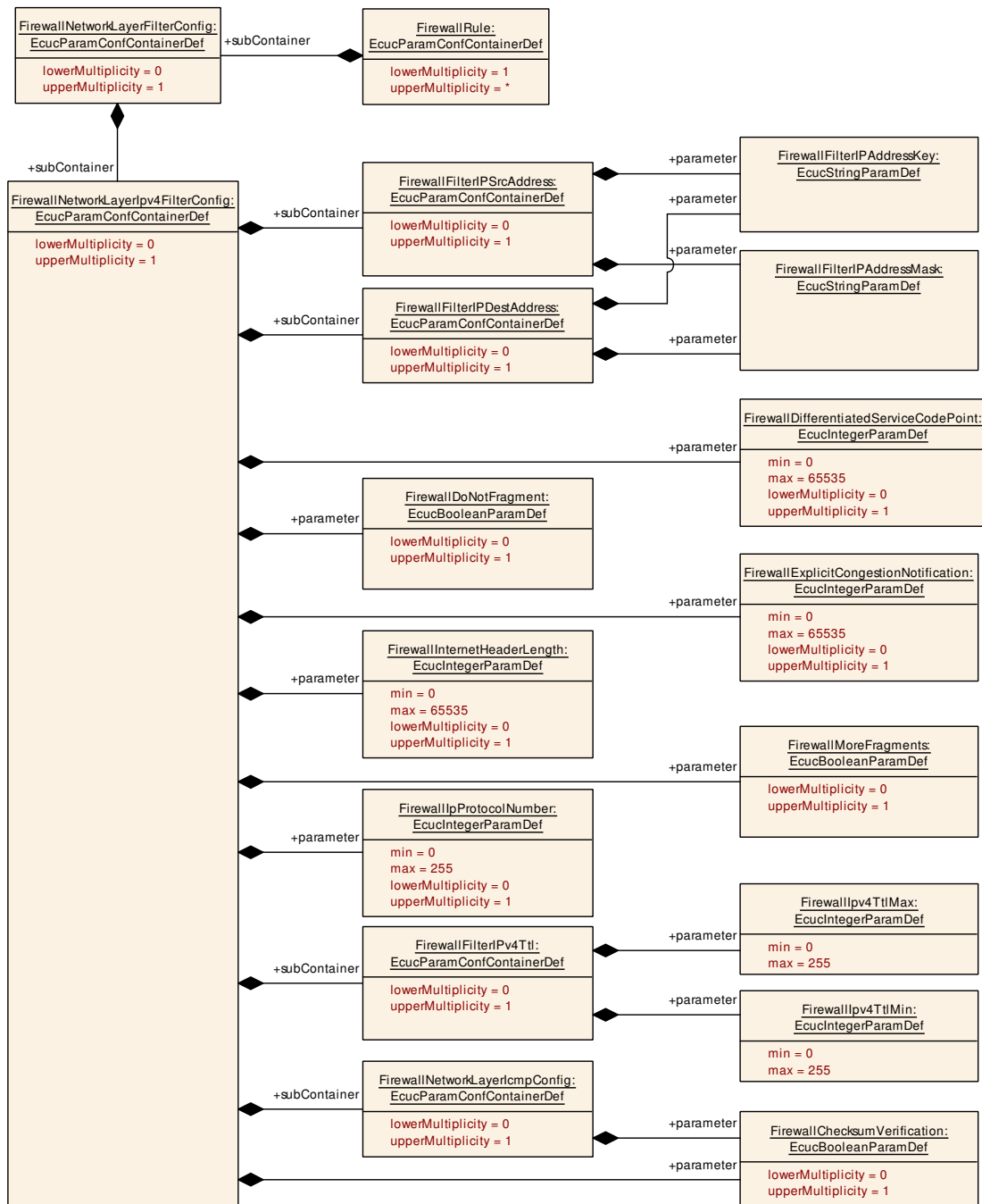
Figure 10.7: IPv4 configuration
