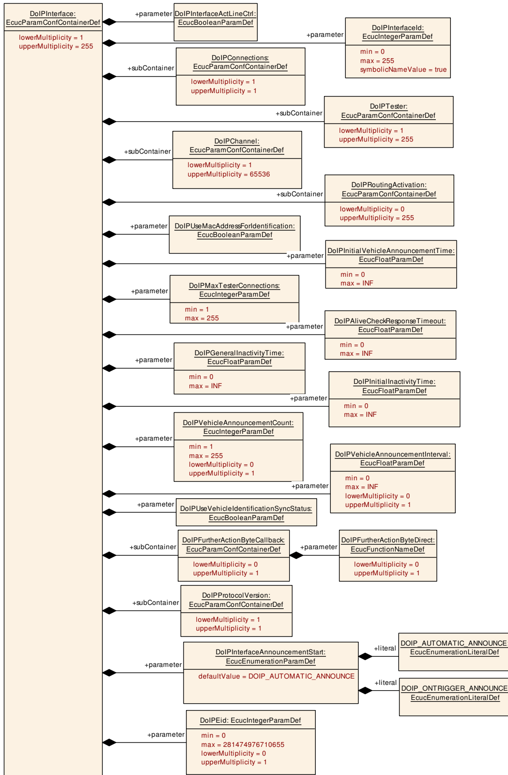
Figure 10.5: DoIPInterface
