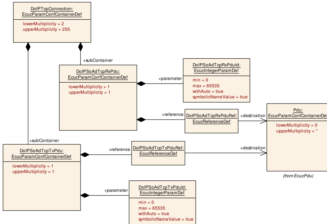
Figure 10.8: DoIPTcpConnection
