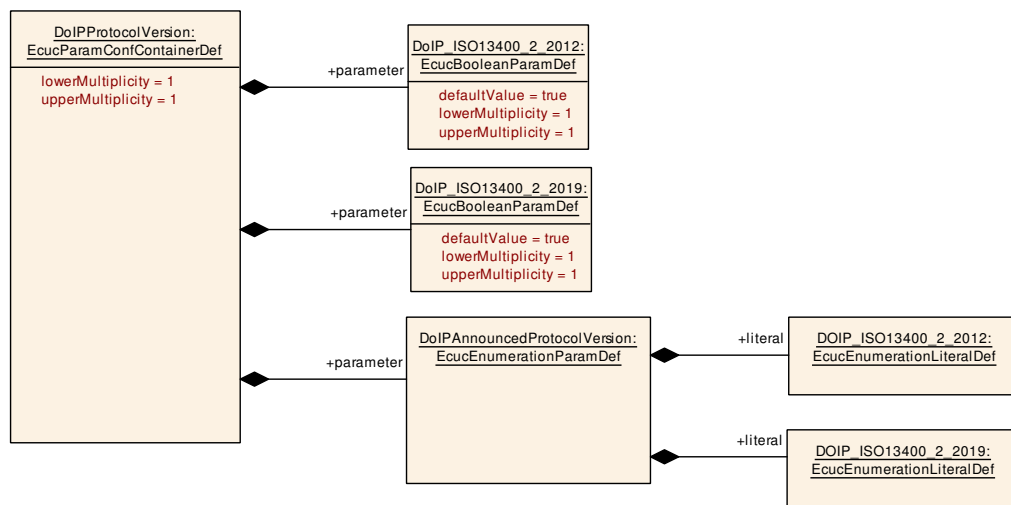
Figure 10.10: DoIPProtocolVersion
