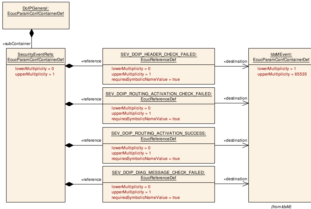
Figure 10.3: SecurityEventRefs
