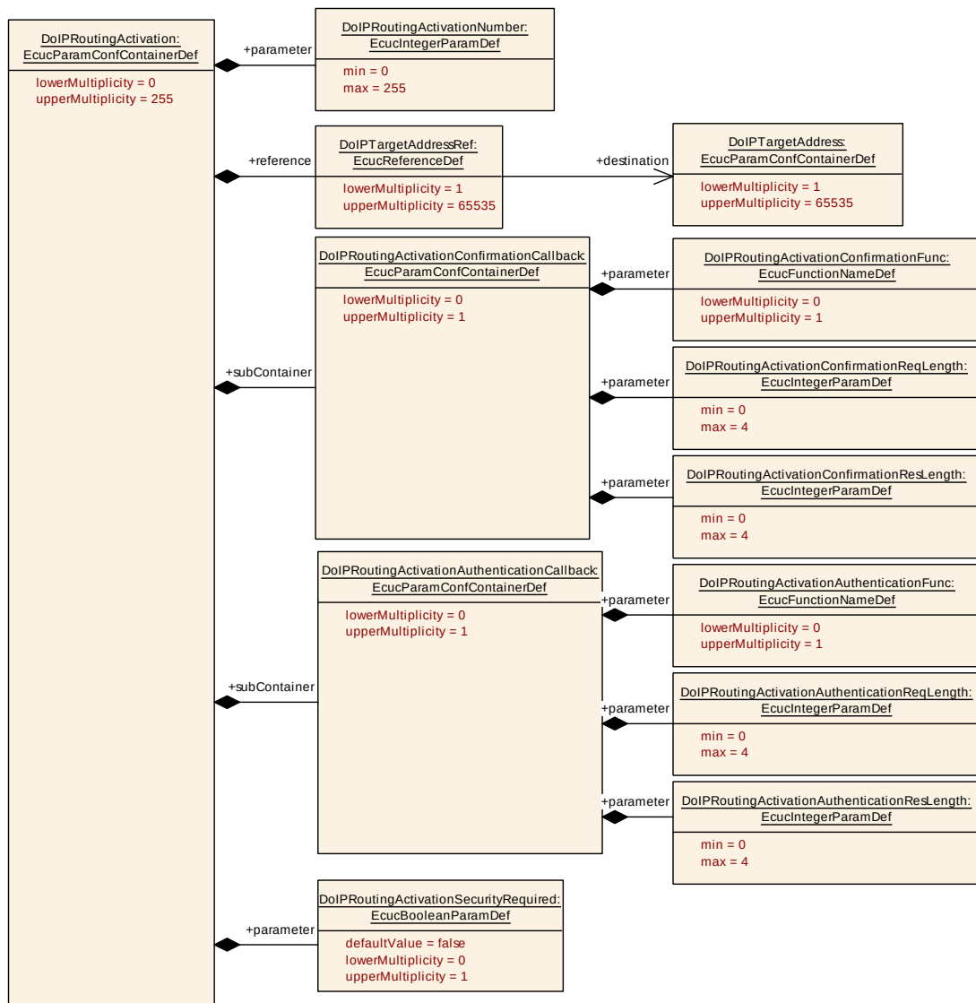
Figure 10.11: DoIPRoutingActivation
