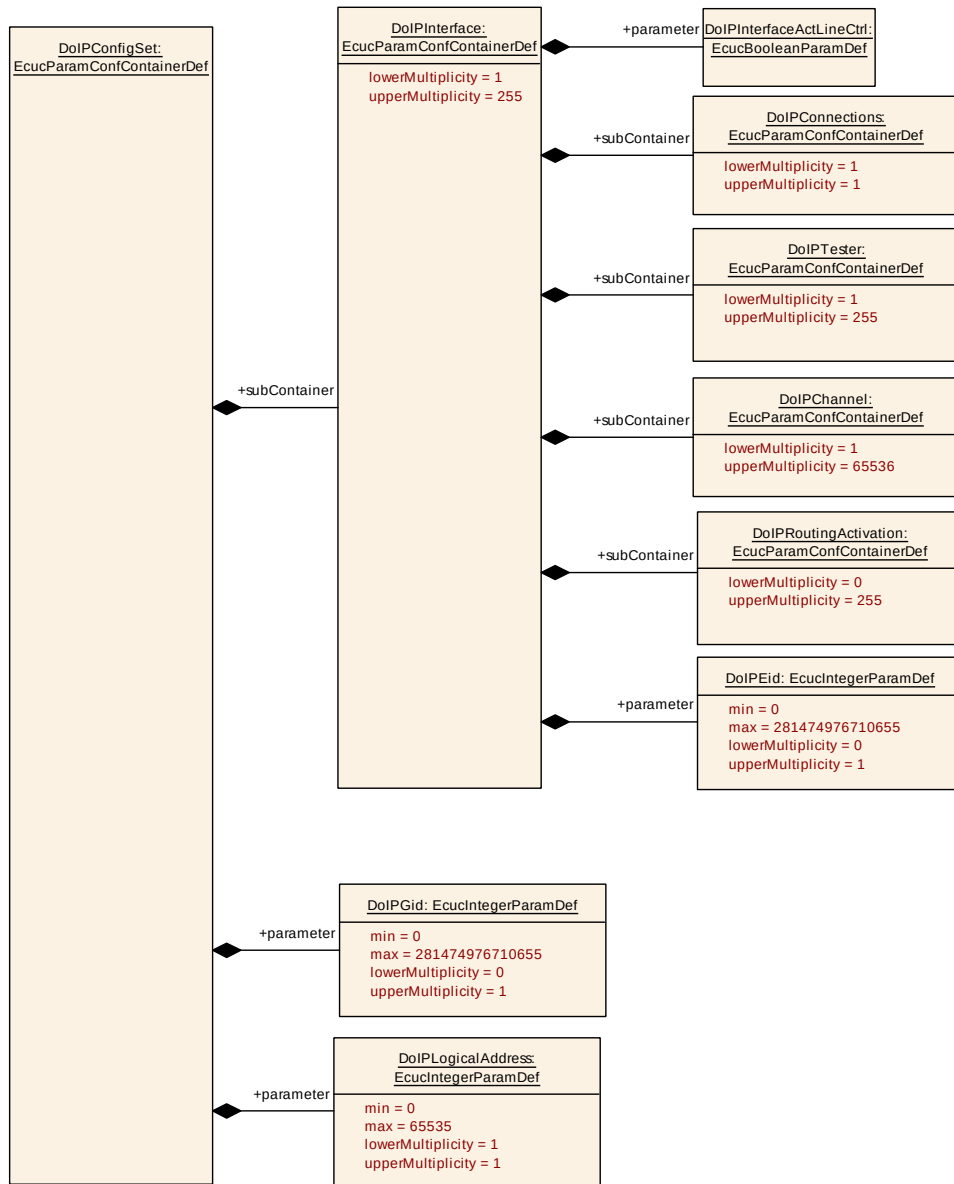
Figure 10.4: DoIPConfigSet
