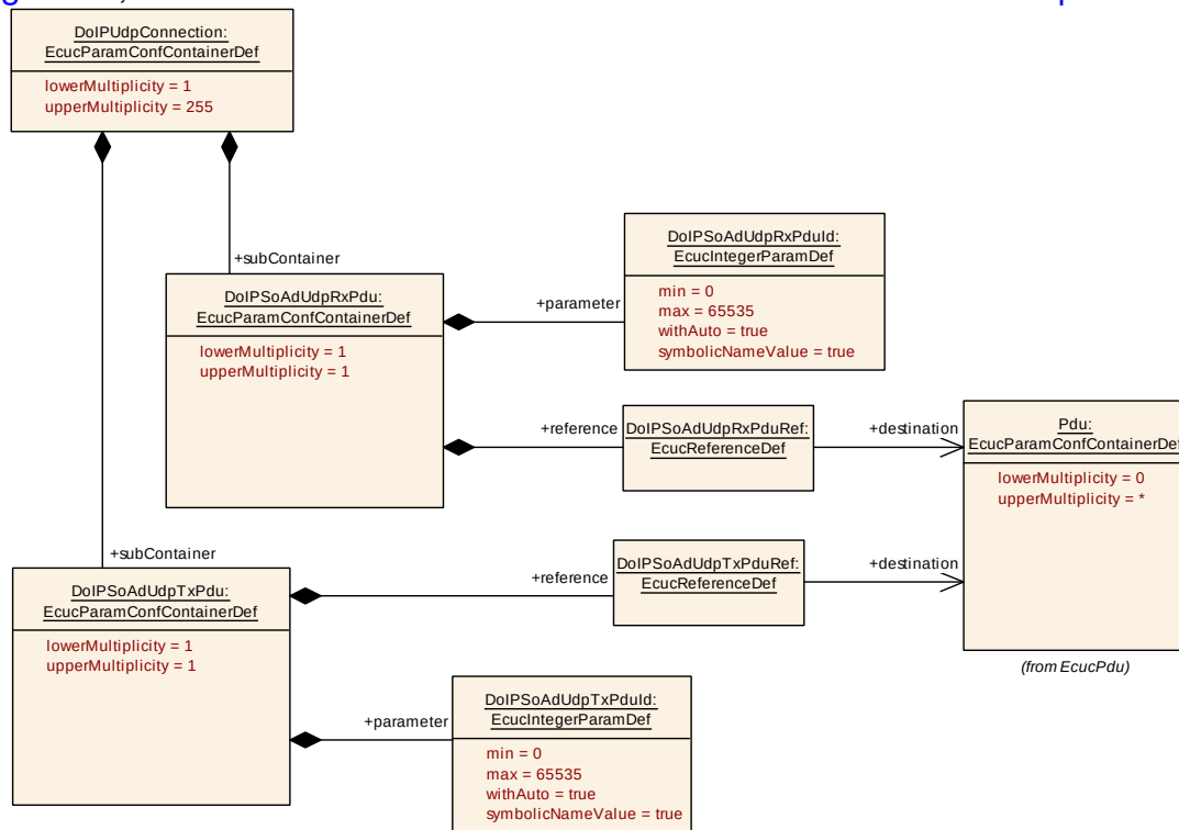
Figure 10.9: DoIPUdpConnection
