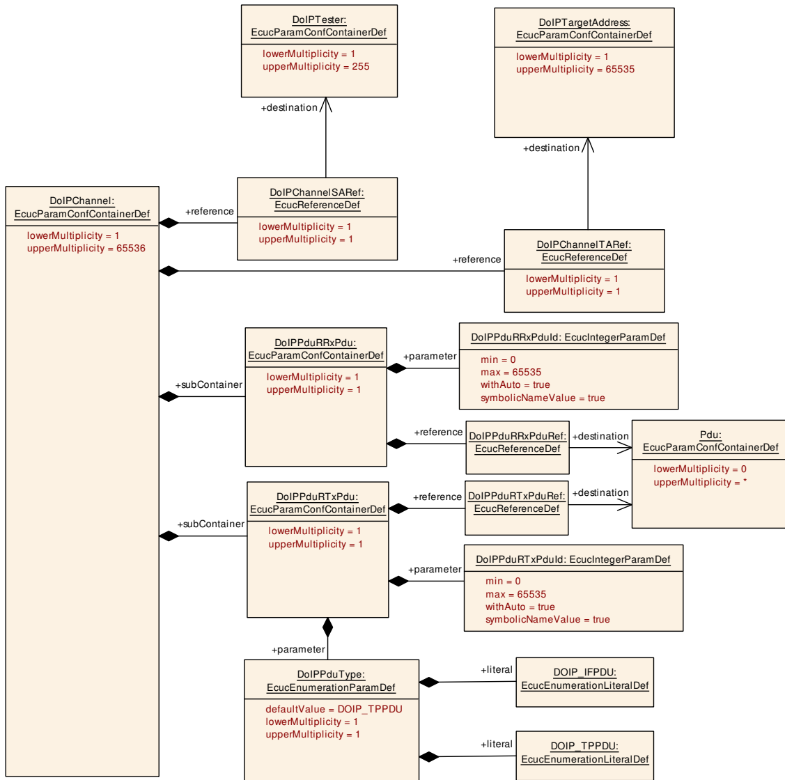
Figure 10.6: DoIPChannel
