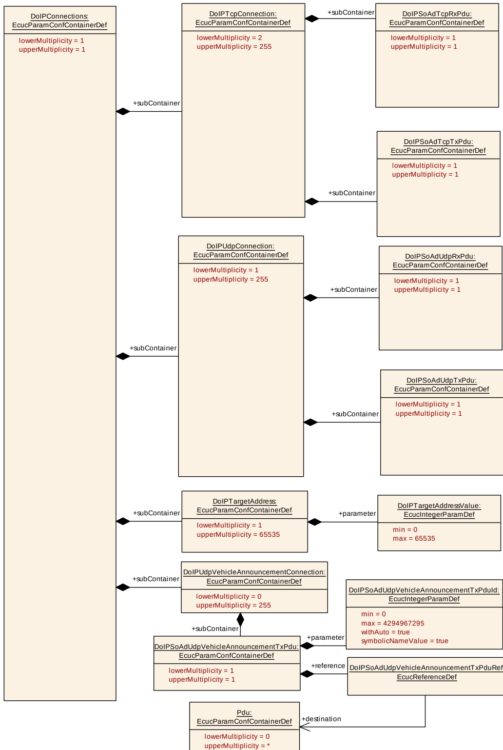
Figure 10.7: DoIPConnections
