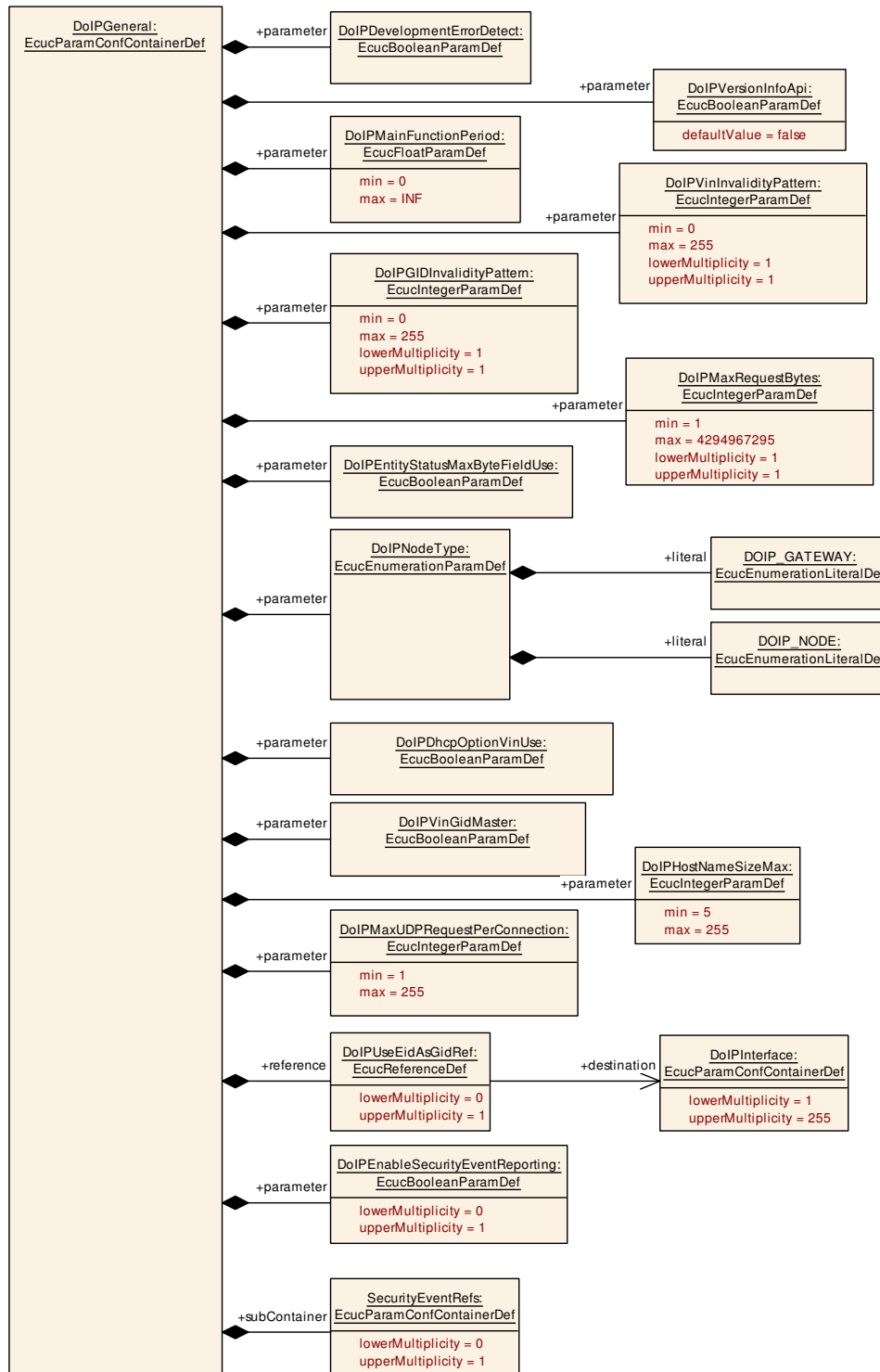
Figure 10.2: DoIPGeneral
