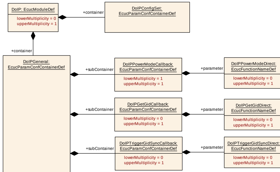
Figure 10.1: DoIP
