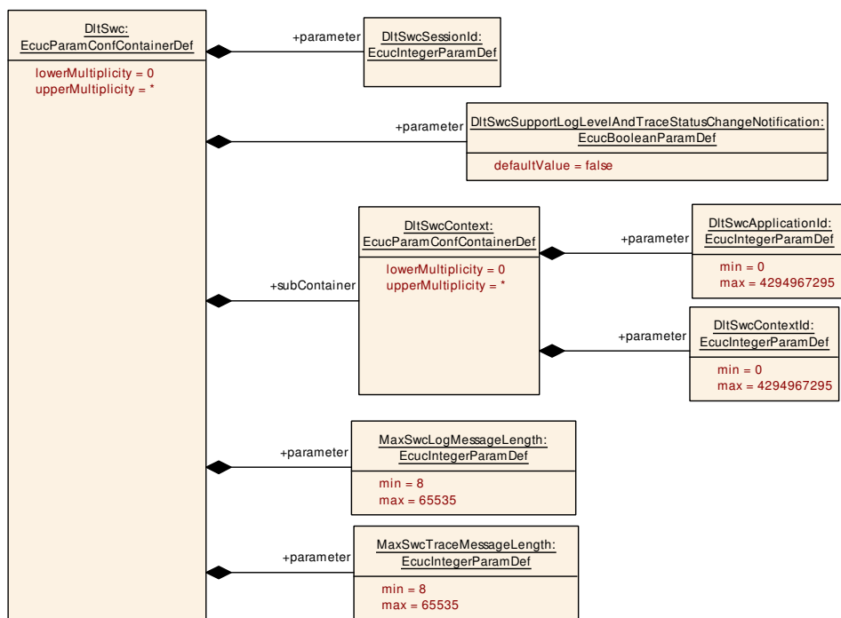
Figure 10.3: DltSwc
