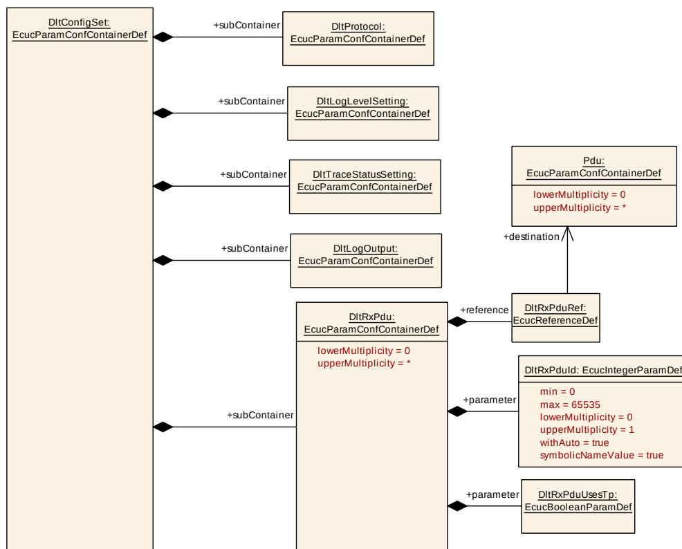
Figure 10.4: DltConfigSet
