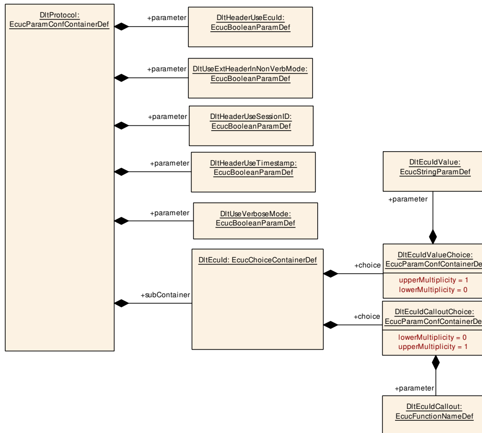
Figure 10.5: DltProtocol
