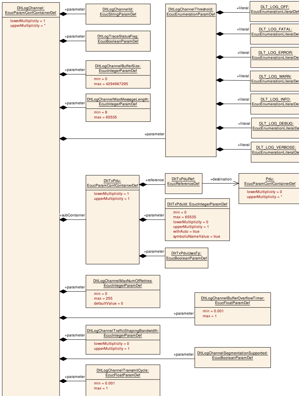
Figure 10.9: DltLogChannel
