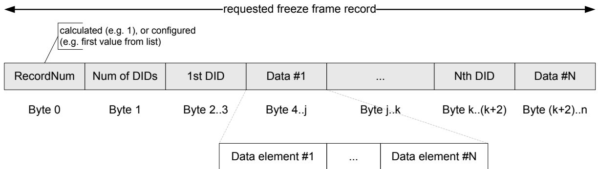
Figure 7.48: Buffer format used by Dem_GetNextFreezeFrameData
