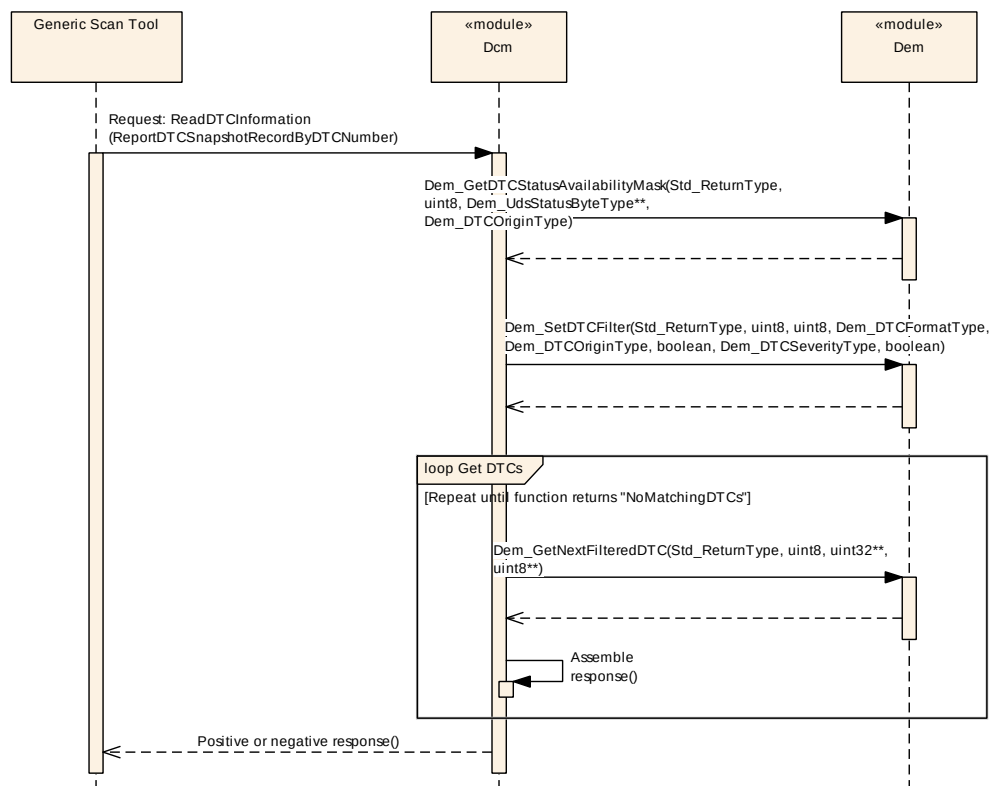
Figure 9.10: Sequence diagram of ReportDTCStatusMask
