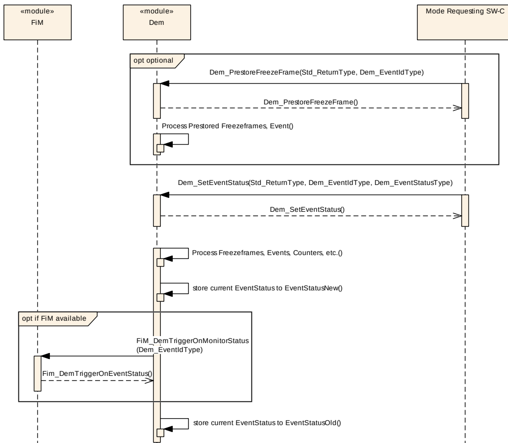
Figure 9.12: Sequence diagram for an example of ProcessEvent Dem-internally
