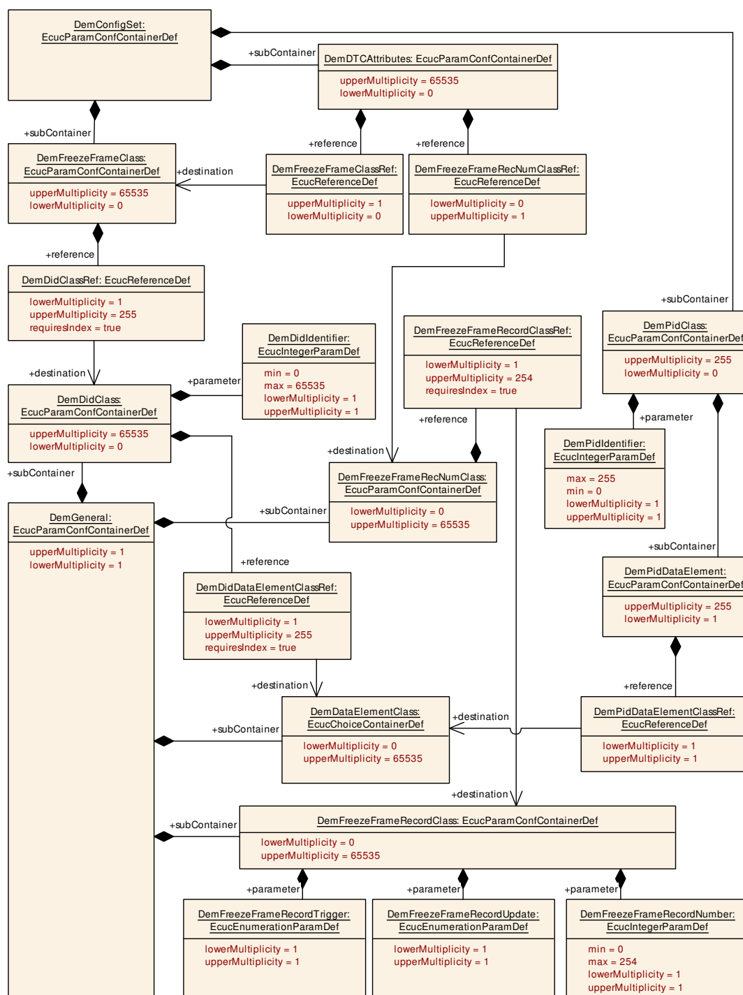
Figure 10.40: DemFreezeFrameClass configuration overview
