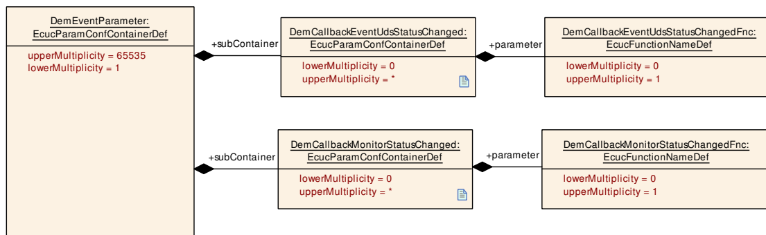
Figure 7.24: EventStatusChanged callback configuration
