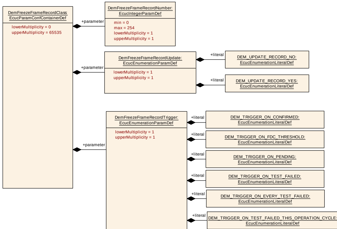
Figure 10.41: DemFreezeFrameRecordClass configuration overview
