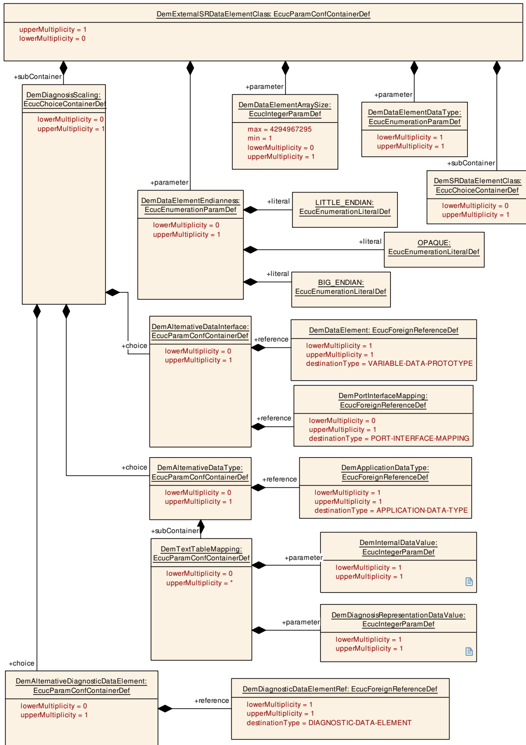
Figure 10.45: DemExternalSRDataElementClass
