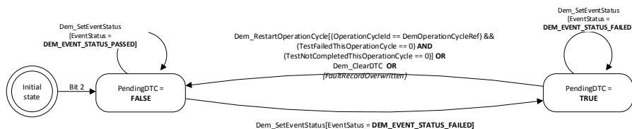
Figure 7.18: UDS status bit 2 PendingDTC logic
