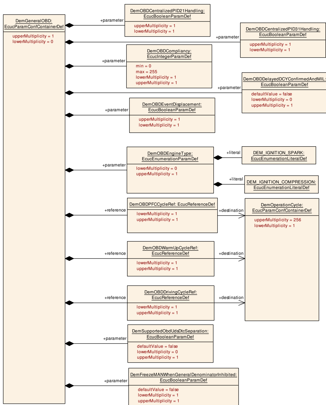
Figure 10.18: DemGeneralOBD configuration overview (part II)
