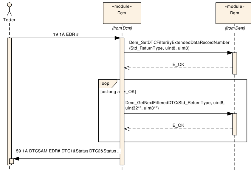
Figure 9.13: Sequence diagram of Dem_GetDTCBasedOnSupportedExtendedDataRecords
