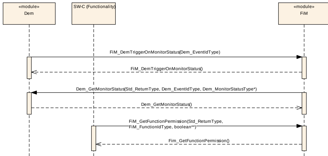
Figure 9.11: Sequence diagram of FiM_DemTriggerOnEventStatus
