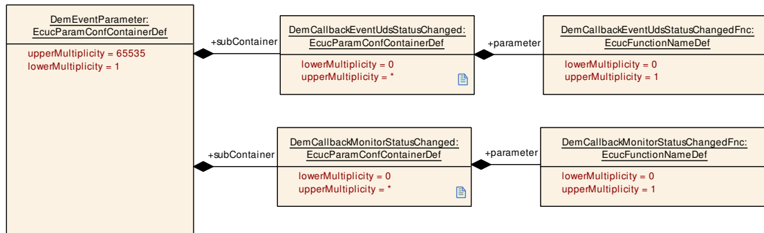
Figure 10.39: Notification of event status changed configuration overview
