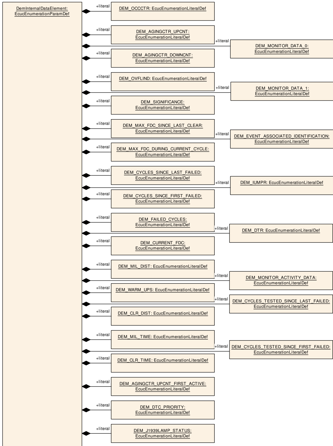
Figure 10.44: DemInternalDataElementClass configuration overview
