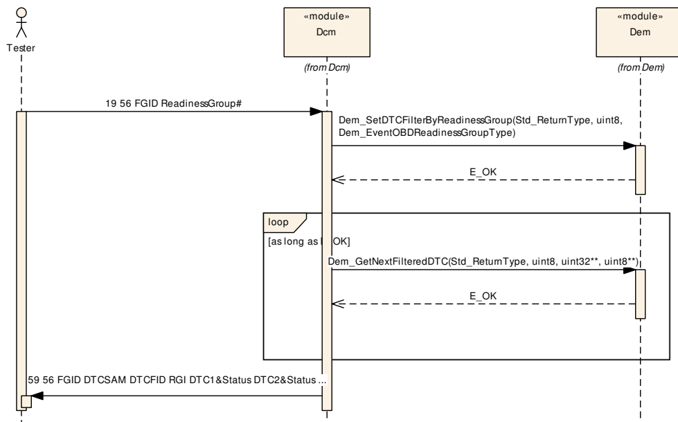
Figure 9.14: Sequence diagram of Dem_GetDTCAssignedToDTCReadinessGroup
