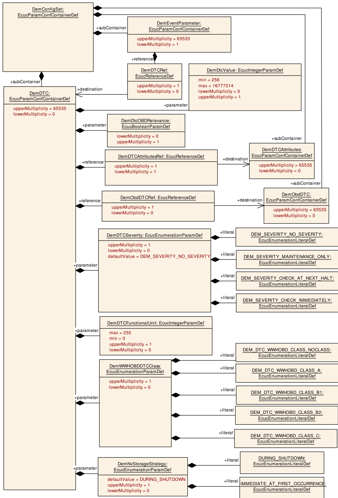
Figure 7.6: DTC configuration
