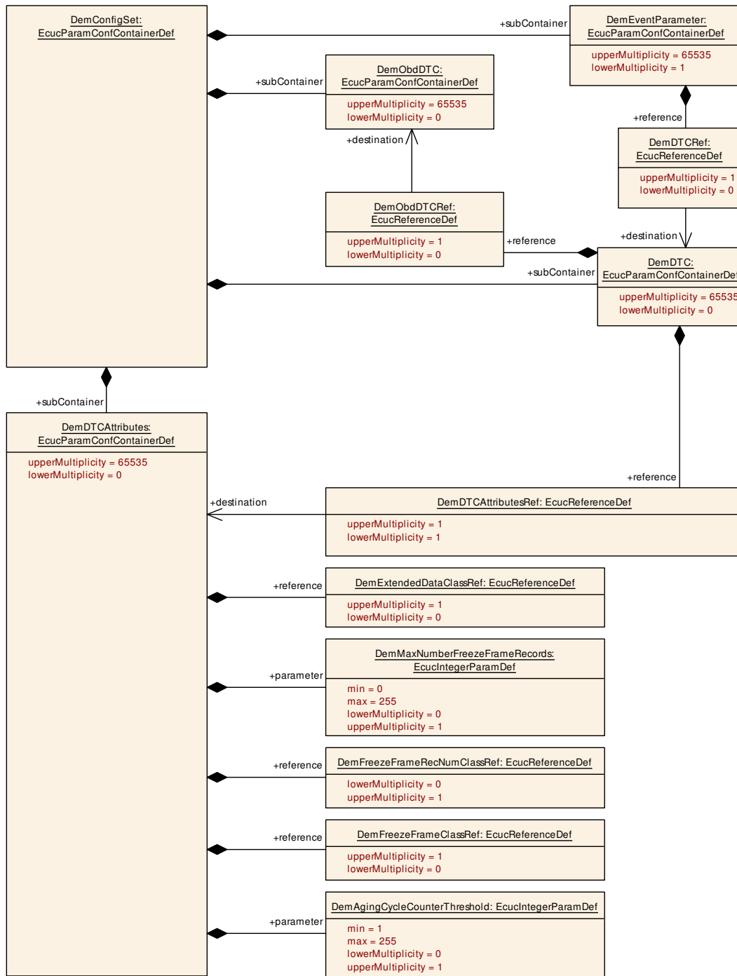
Figure 10.5: DTC attribute configuration overview (part I)
