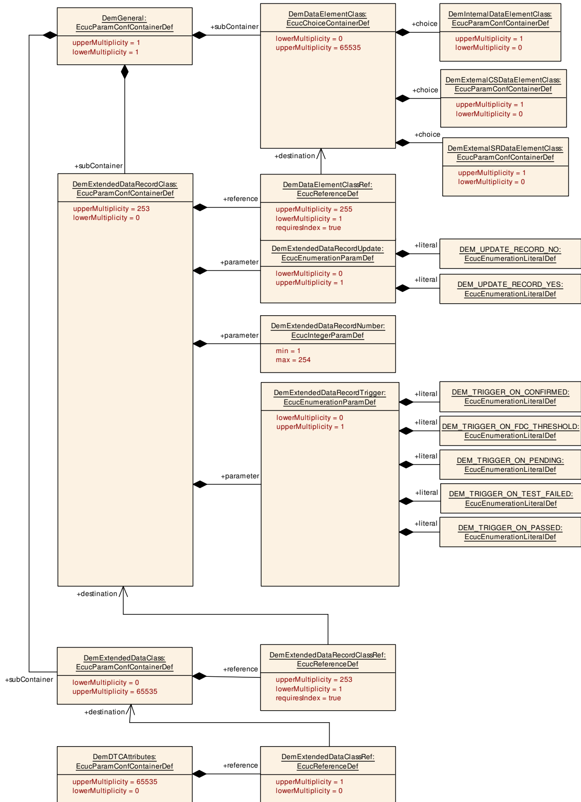
Figure 10.42: DemExtendedDataClass configuration overview
