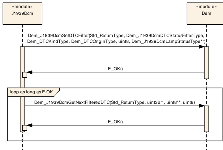
Figure 9.9: Sequence diagram of Dem_J1939DcmGetNextFilteredDTC
