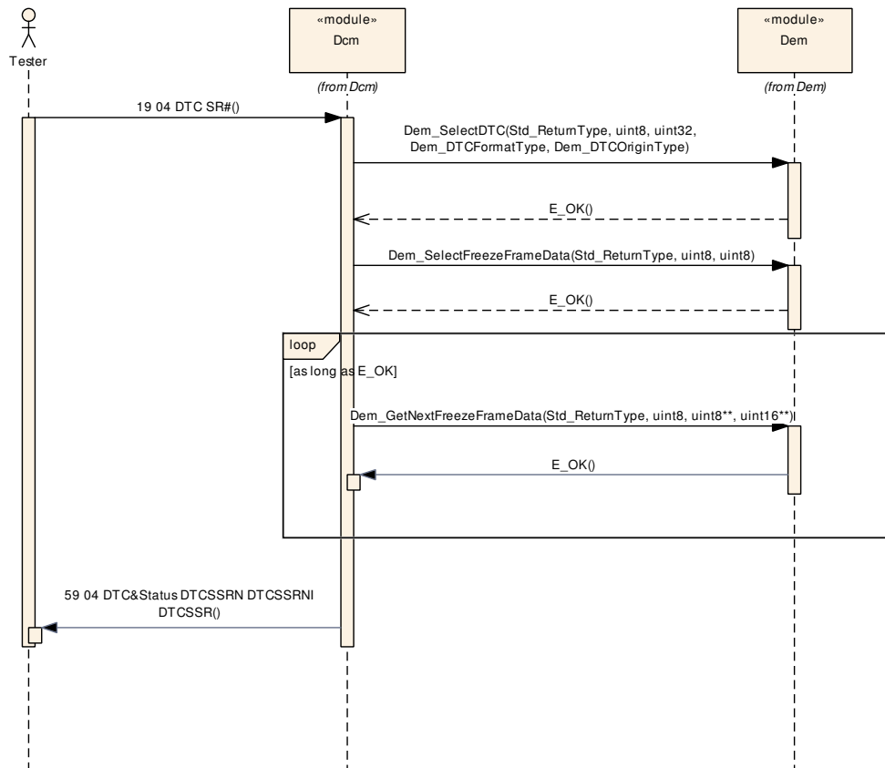
Figure 9.7: Sequence diagram to retrieve freeze frames
