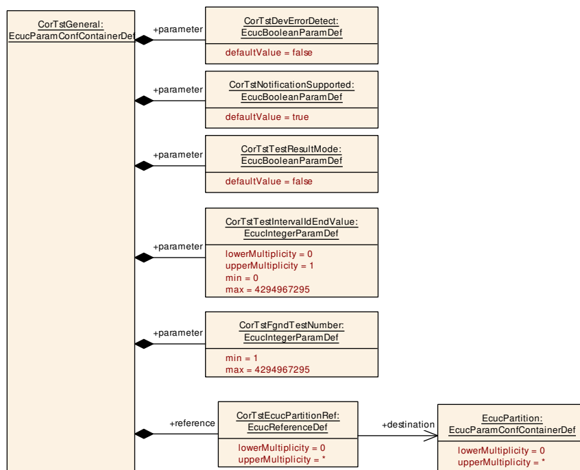
Figure 10.2: CorTstGeneral
