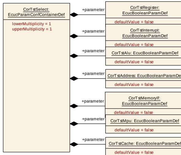
Figure 10.3: CorTstSelect
