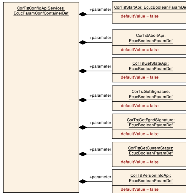
Figure 10.4: CorTstConfigApiServices
