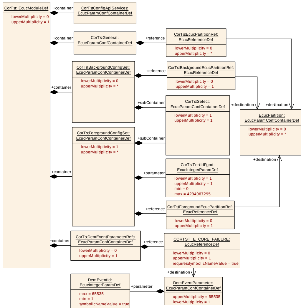
Figure 10.1: CorTst
