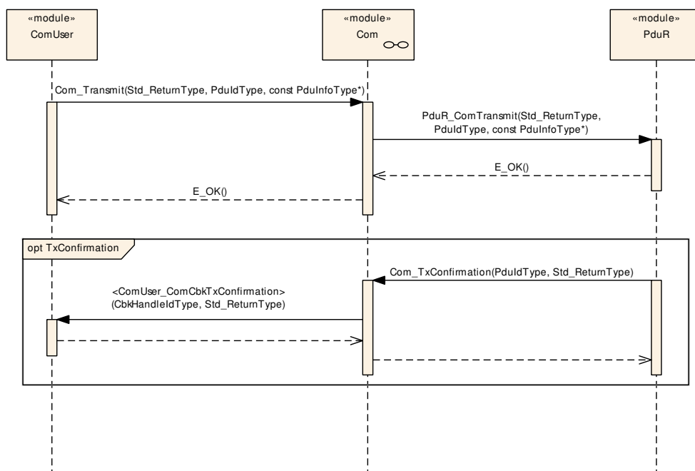
Figure 9.5: Transmission via Large Data Path using IF API
