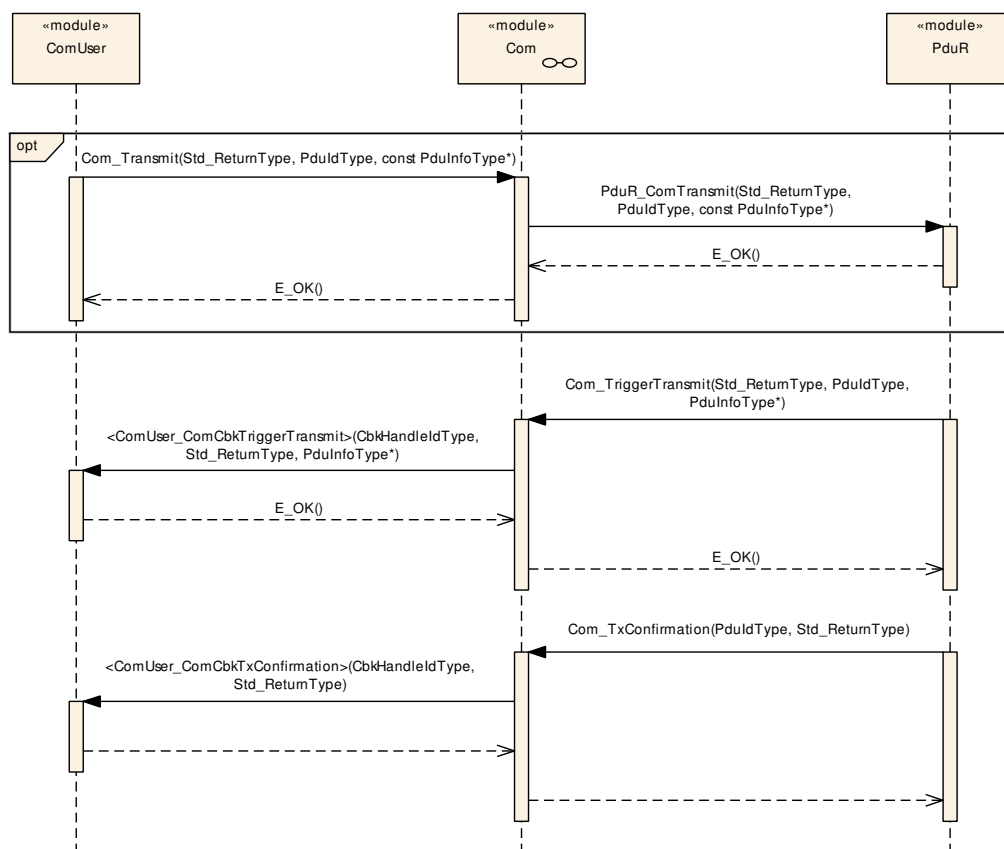
Figure 9.6: Transmission via Large Data Path using TriggerTransmit
