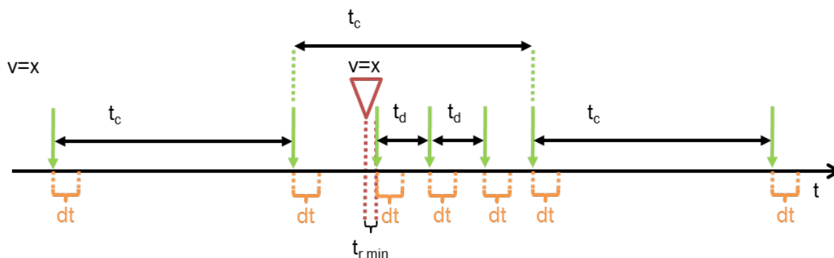
Figure B.9: Use case 5 scenario a, TM MIXED, here n = 2 (without TMS switch)
