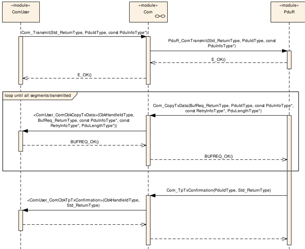
Figure 9.4: Transmission via Large Data Path using TP API
