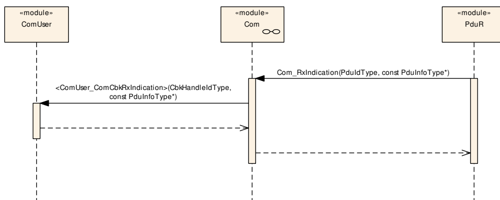
Figure 9.8: Reception via Large Data Path using IF API
