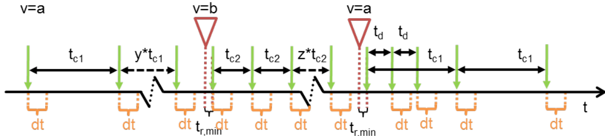
Figure B.11: Use Case 6, TM MIXED , here n = 2 + \text{PERIODIC} (with TMS switch)
