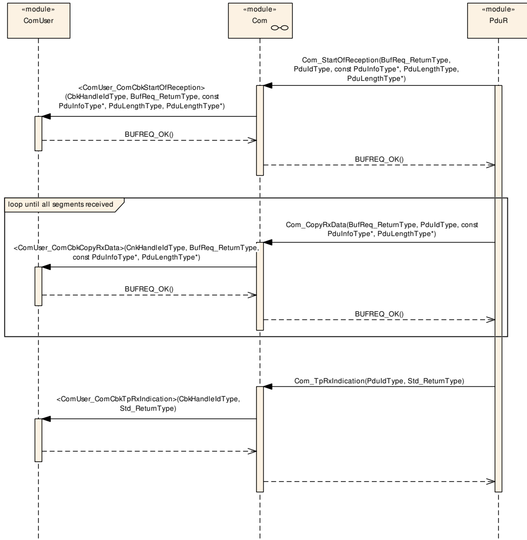
Figure 9.7: Reception via Large Data Path using TP API
