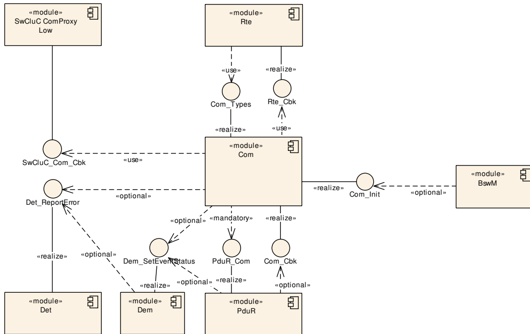
Figure 5.1: AUTOSAR COM module's context view
