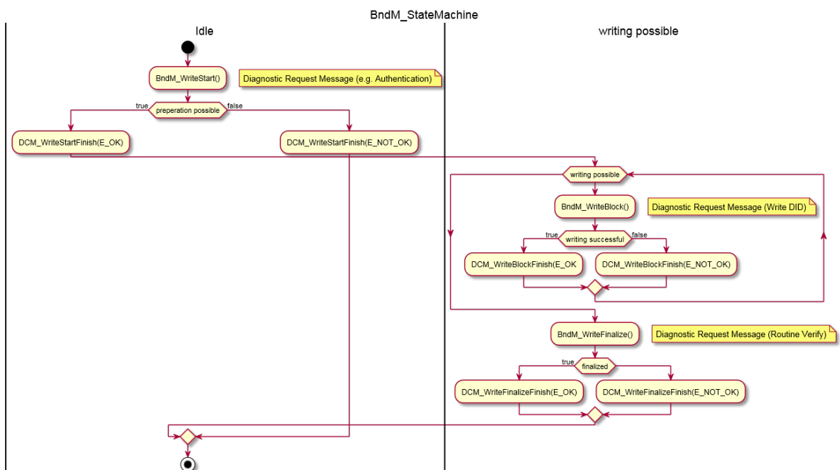
Figure 7.1: Figure BndMStateMachine
