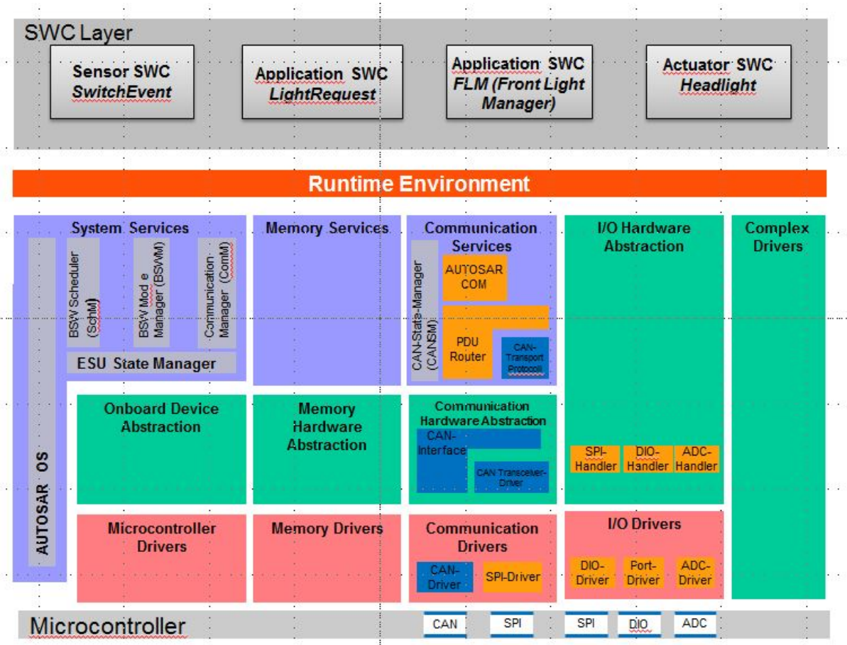
Figure 5.2: SW Components and Involved AUTOSAR BSW Modules
