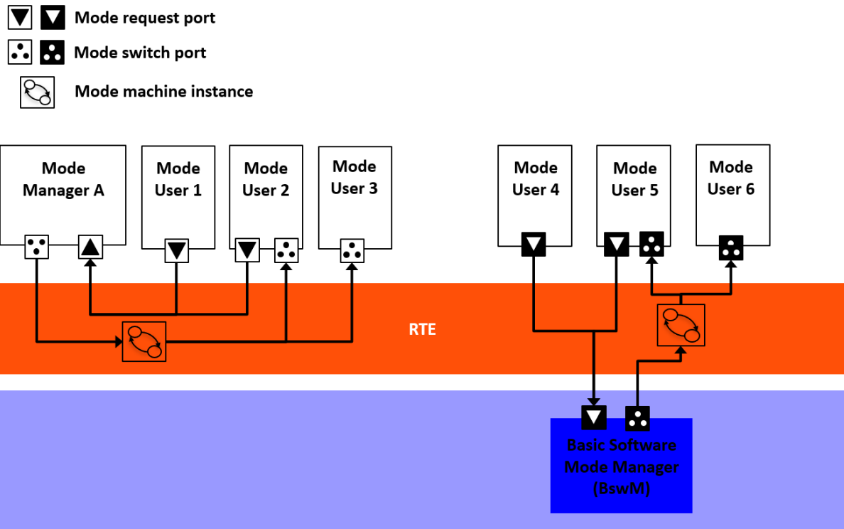
Figure 2.2: Example showing the BswM and some SWCs acting as mode manager-s/users
