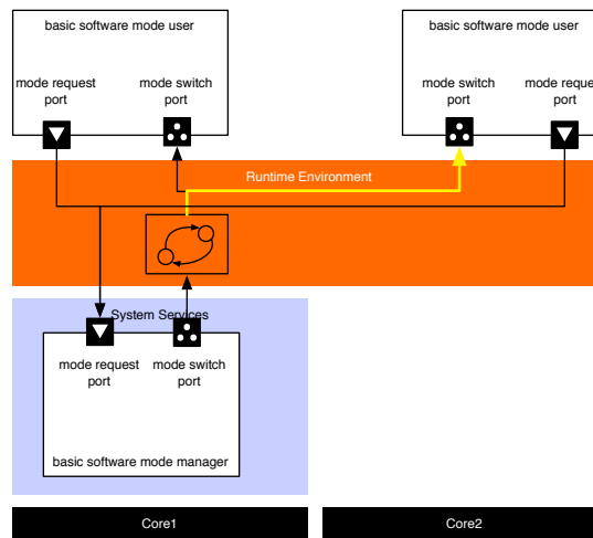
Figure 2.6: Example configuration
