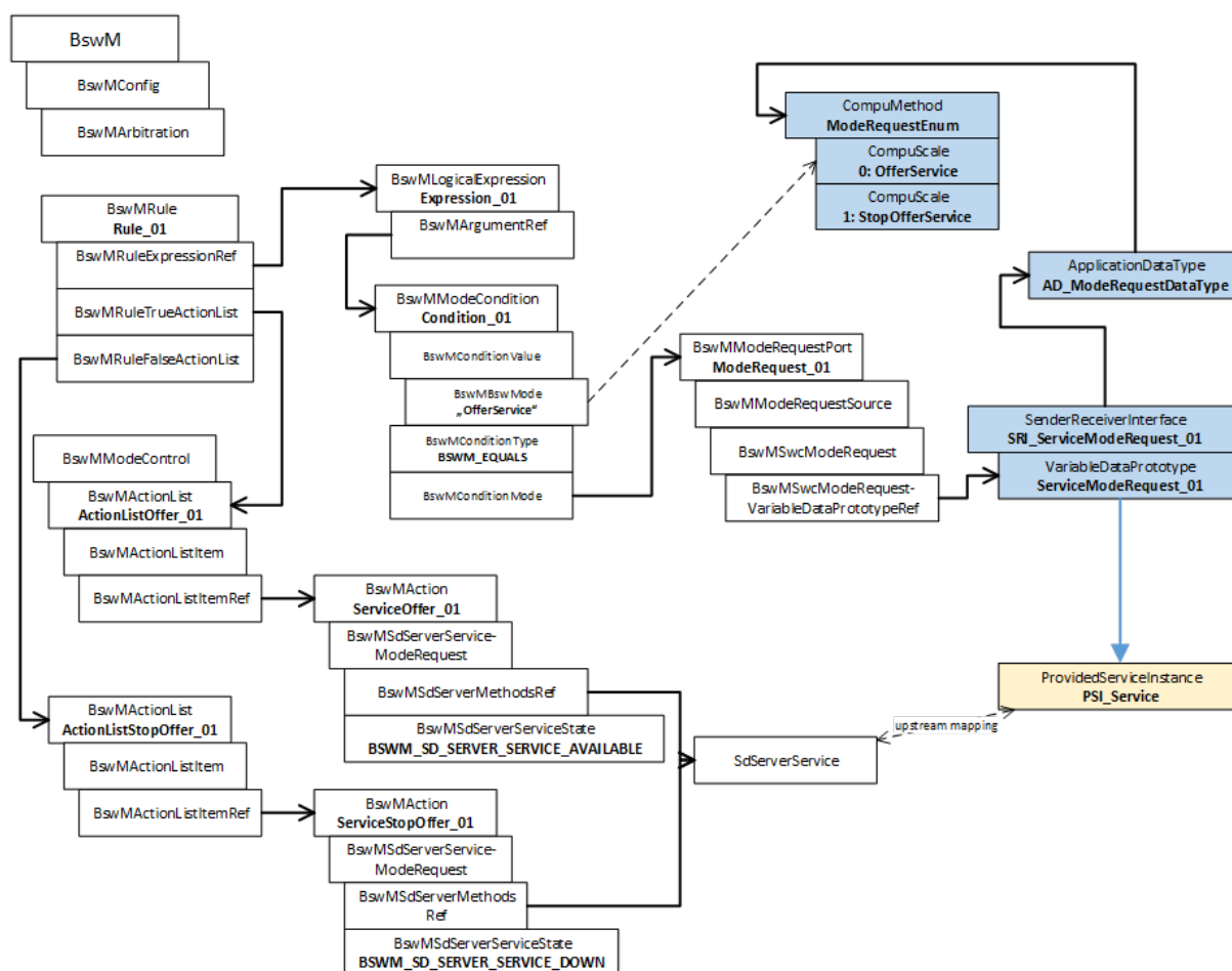
Figure 3.6: Example for a generated BswM configuration
