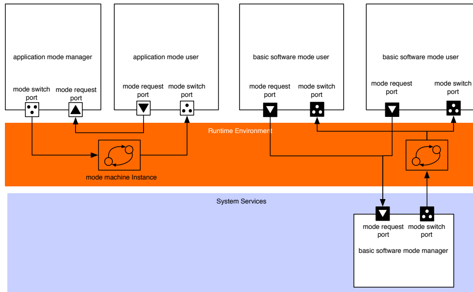
Figure 2.3: The RTE instantiates for each ModeDeclarationGroupPrototype a ModeMachineInstance
