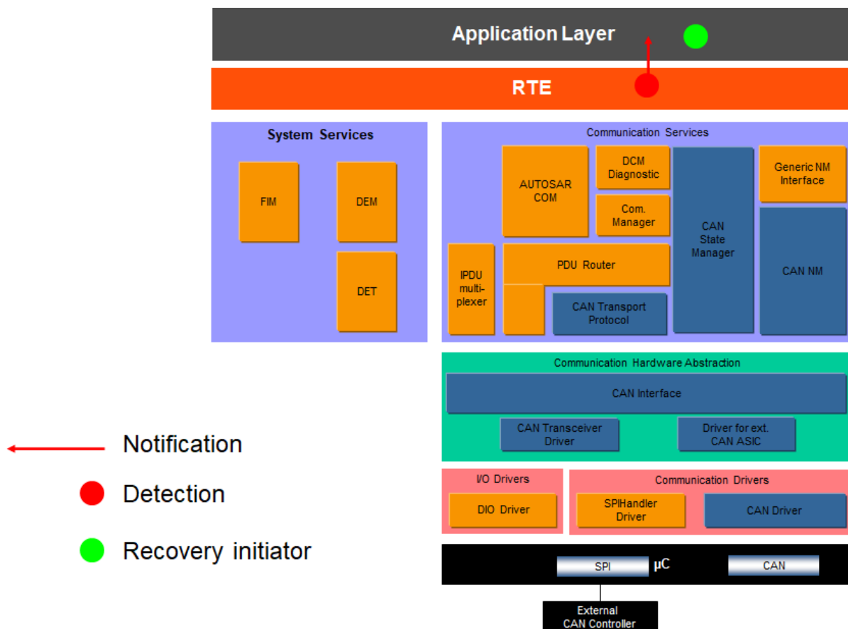
Figure 5.10: Information path for the client / server timeout
