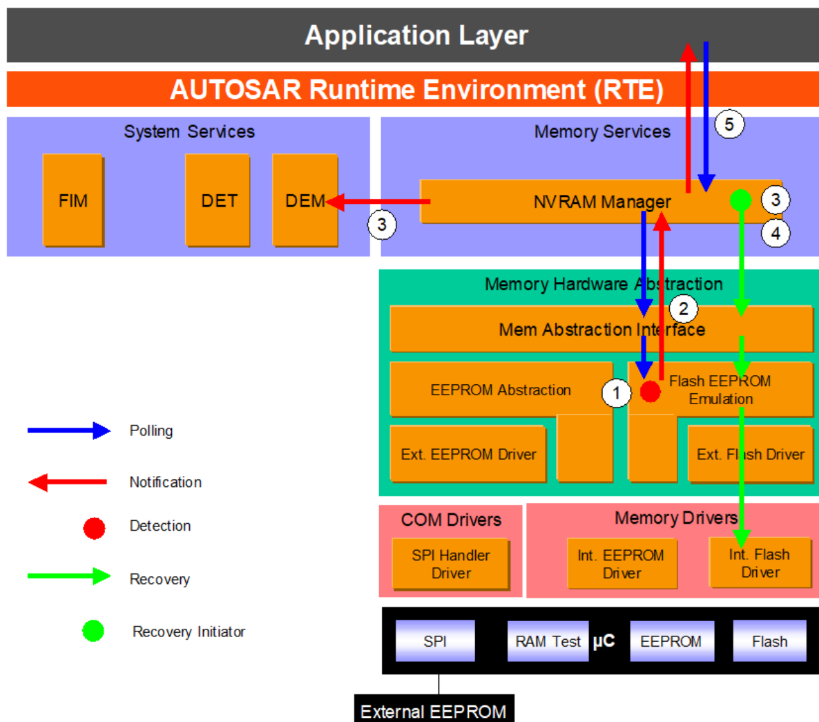
Figure 6.11: Information path for the Fee consistency check
