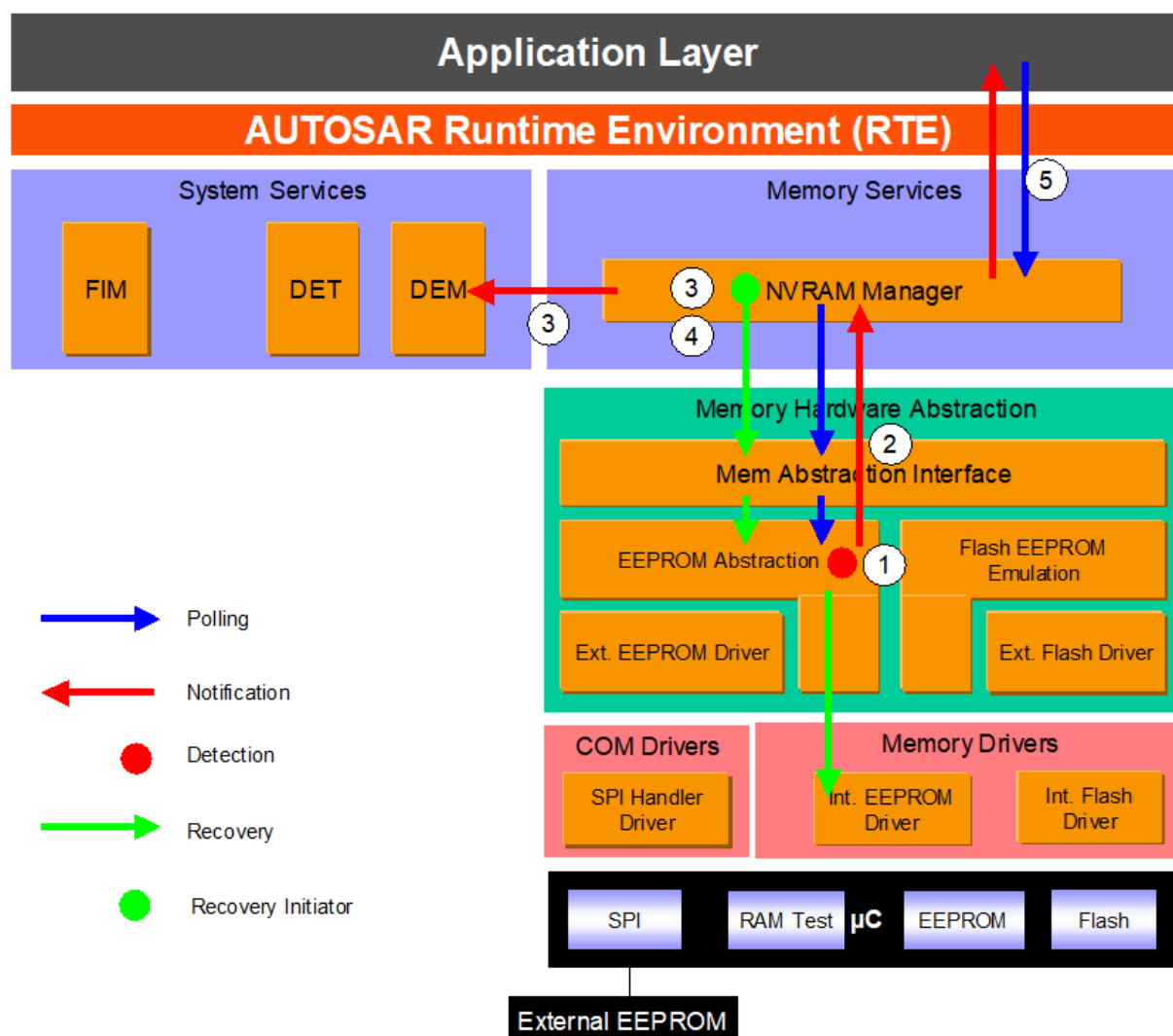
Figure 6.12: Information path for the EA consistency check error
