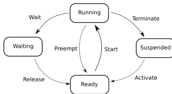
Figure 3.1: Standard Task State Diagram AR_CP_OS_TASK
