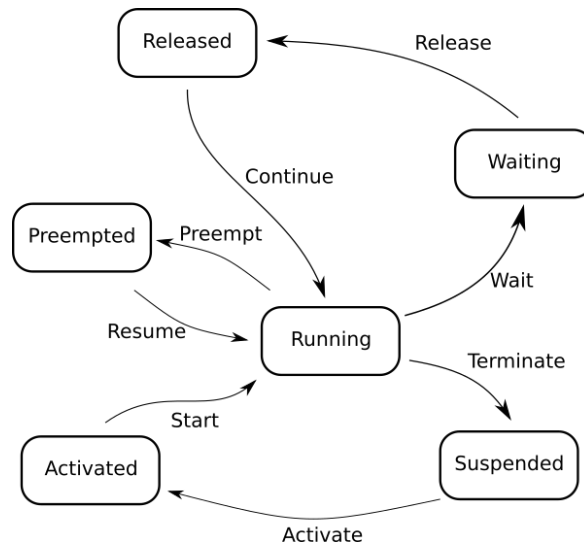
Figure 3.2: Enhanced Task State Diagram AR_CP_OSARTI_TASK
