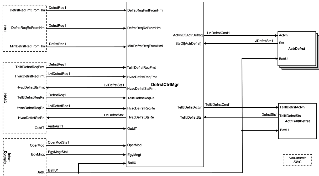
Figure 4.26: DefrostControl
