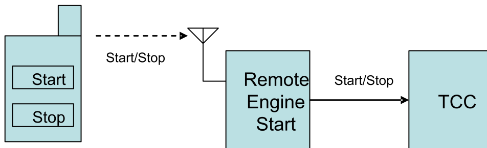
Figure 4.34: TerminalClampControl
