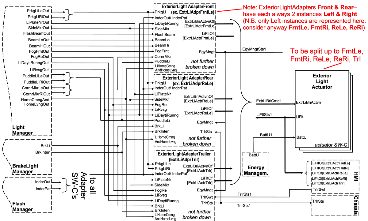
Figure 4.18: ExteriorLight decomposition
