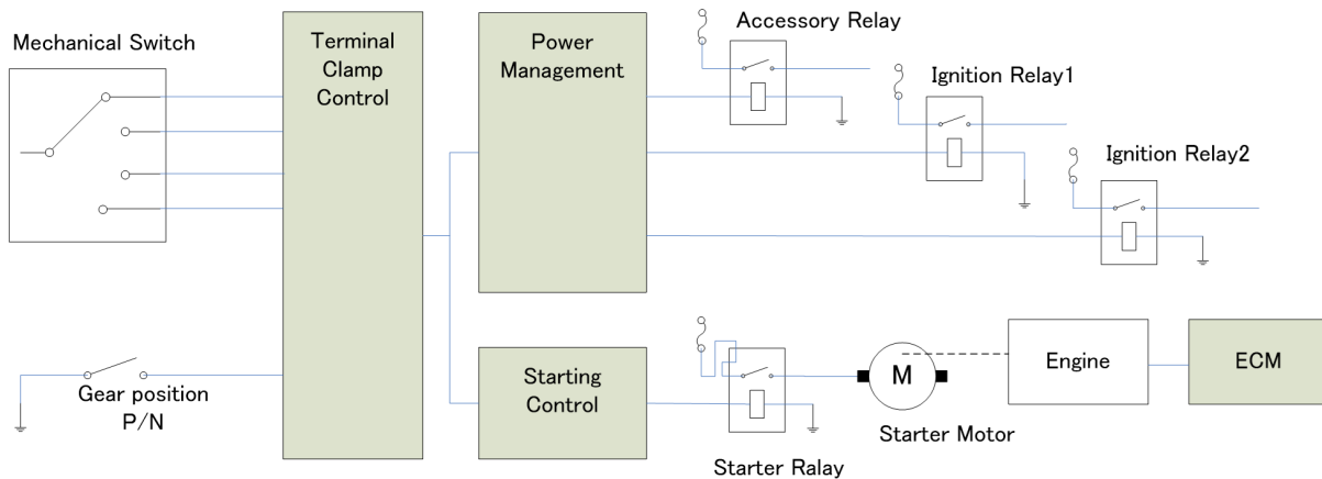
Figure 4.29: TerminalClampControl
