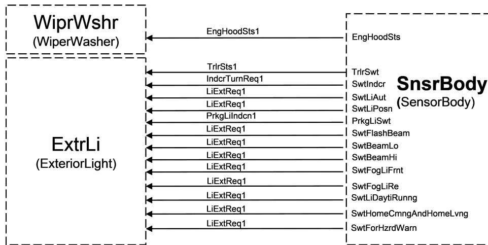
Figure 4.43: BodySensors
