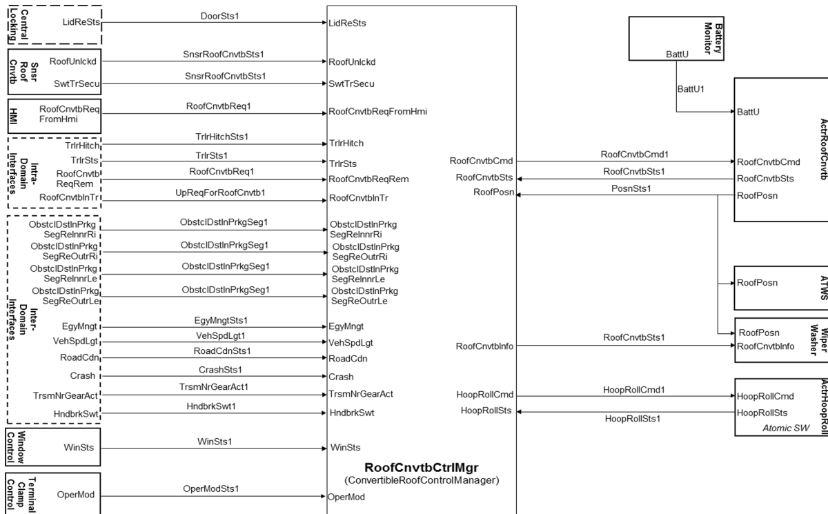
Figure 4.42: ConvertibleControl
