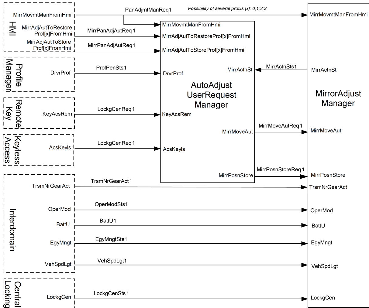
Figure 4.3: Mirror Adjustment & Tinting
