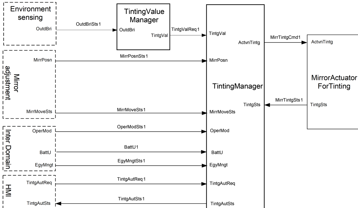
Figure 4.5: Mirror Tinting
