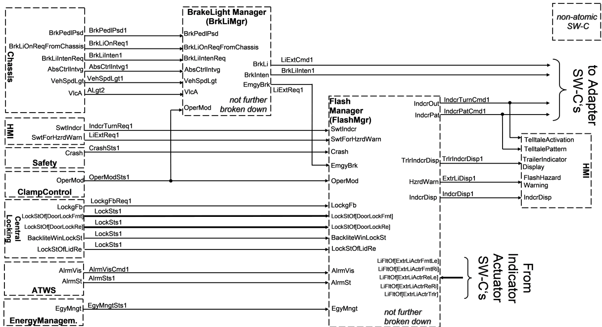
Figure 4.17: ExteriorLight decomposition
