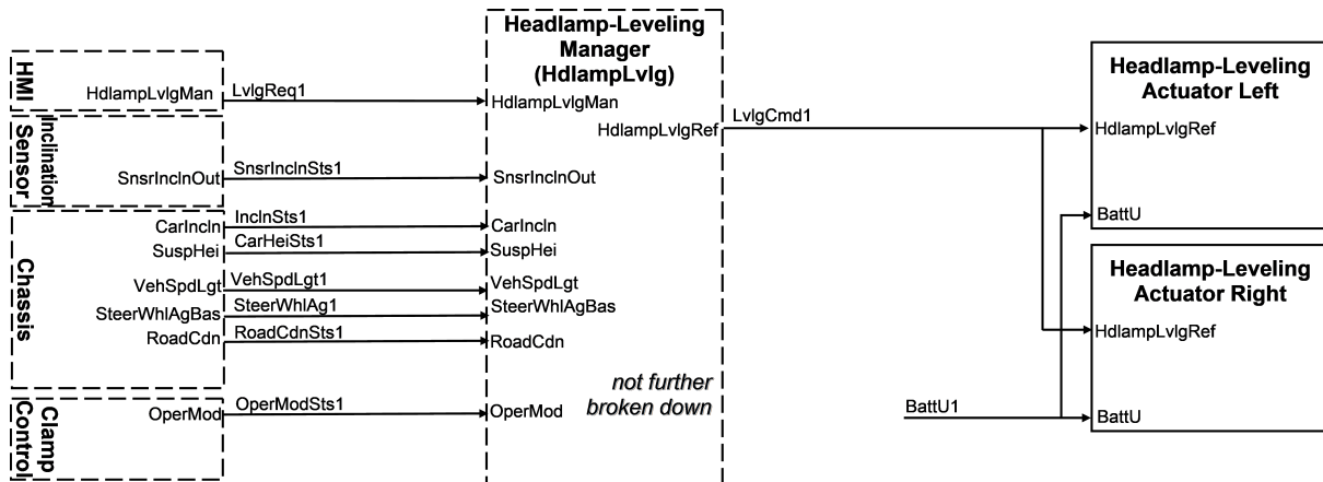
Figure 4.19: ExteriorLight decomposition
