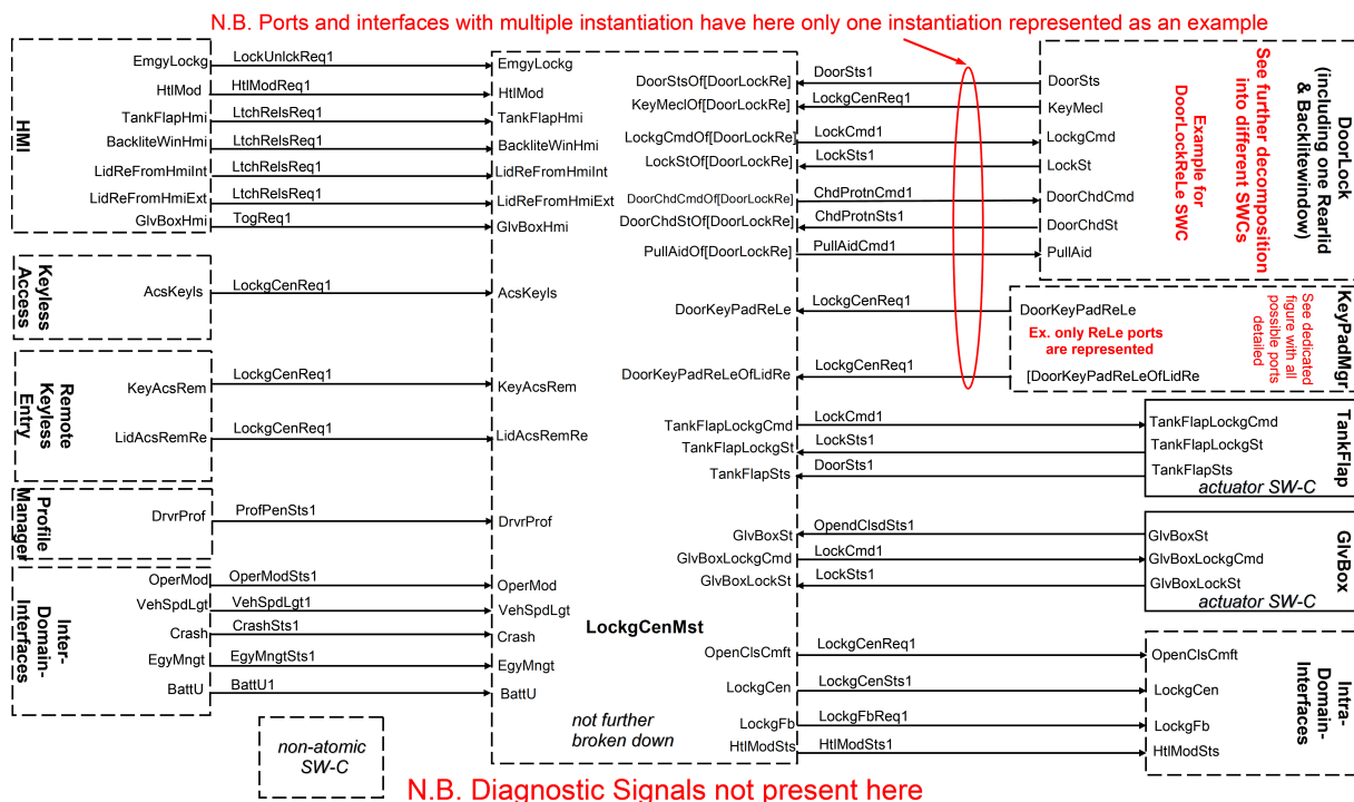
Figure 4.11: CentralLocking
