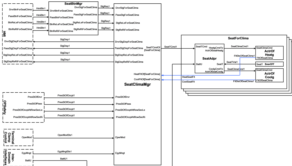
Figure 4.37: SeatClimatization Decomposition
