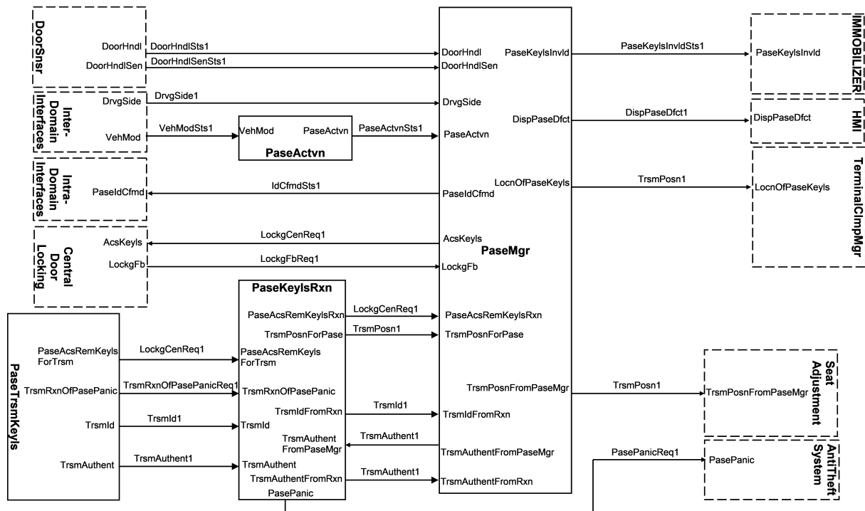
Figure 4.38: PassiveEntry
