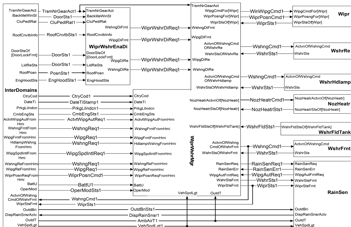
Figure 4.1: WiperWasher
