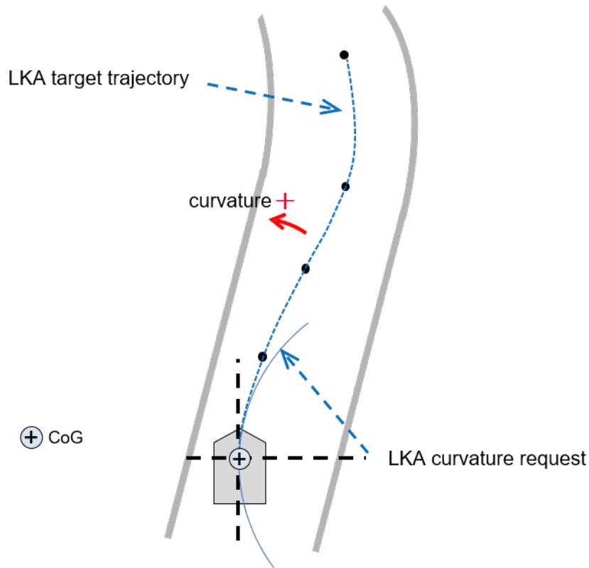
Figure 2.7: Curvature request
