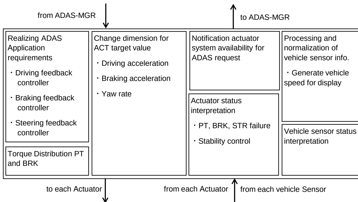
Figure 4.4: Vehicle-MGR functions
