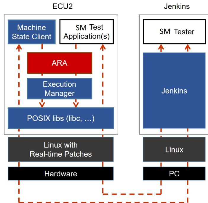
Figure 17.1: Illustration of test setup for State Management.
