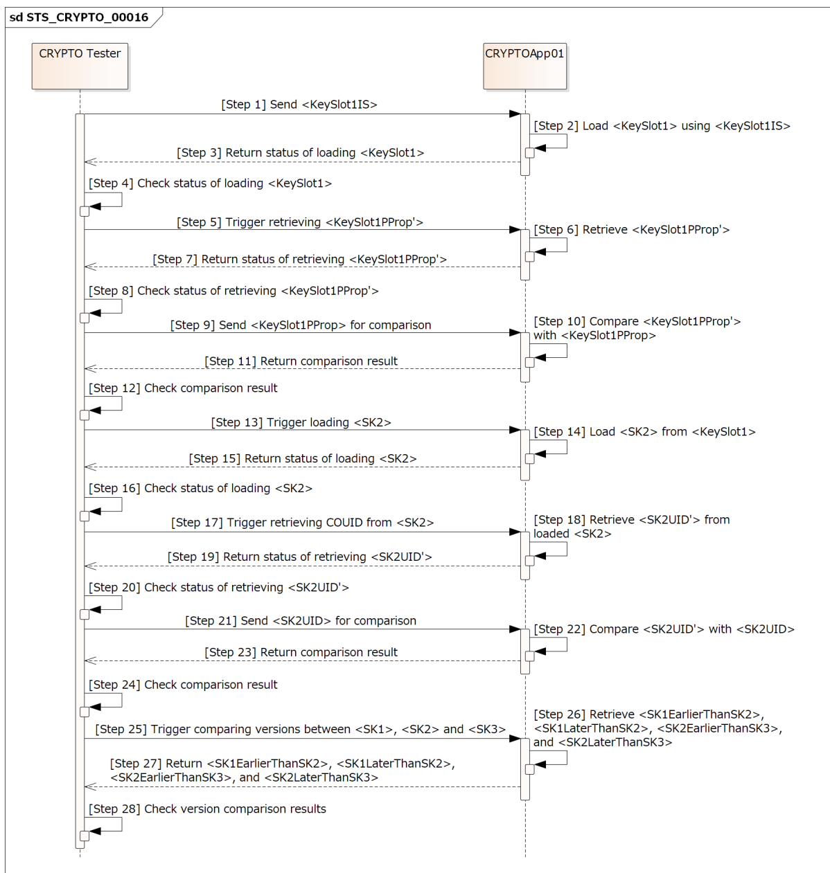
Figure 15.15: Sequence diagram of STS_CRYPT0_00016.
