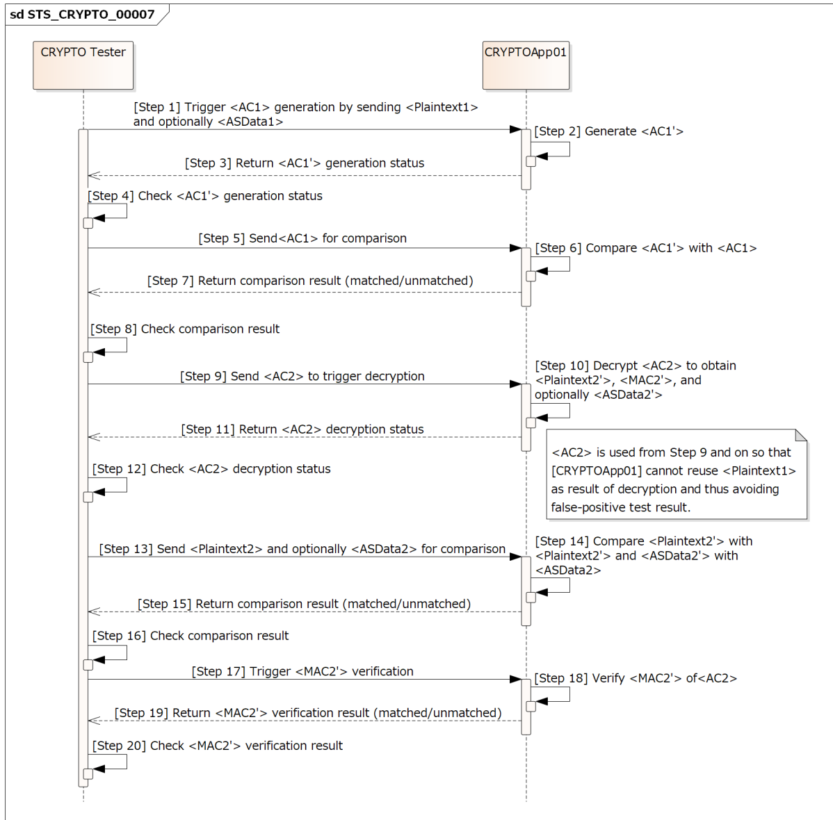
Figure 15.5: Sequence diagram of STS_CRYPTO_00007.
