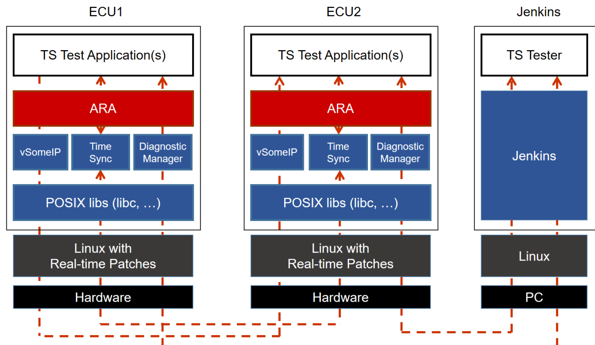
Figure 12.1: Illustration of test setup for Time Synchronization.
