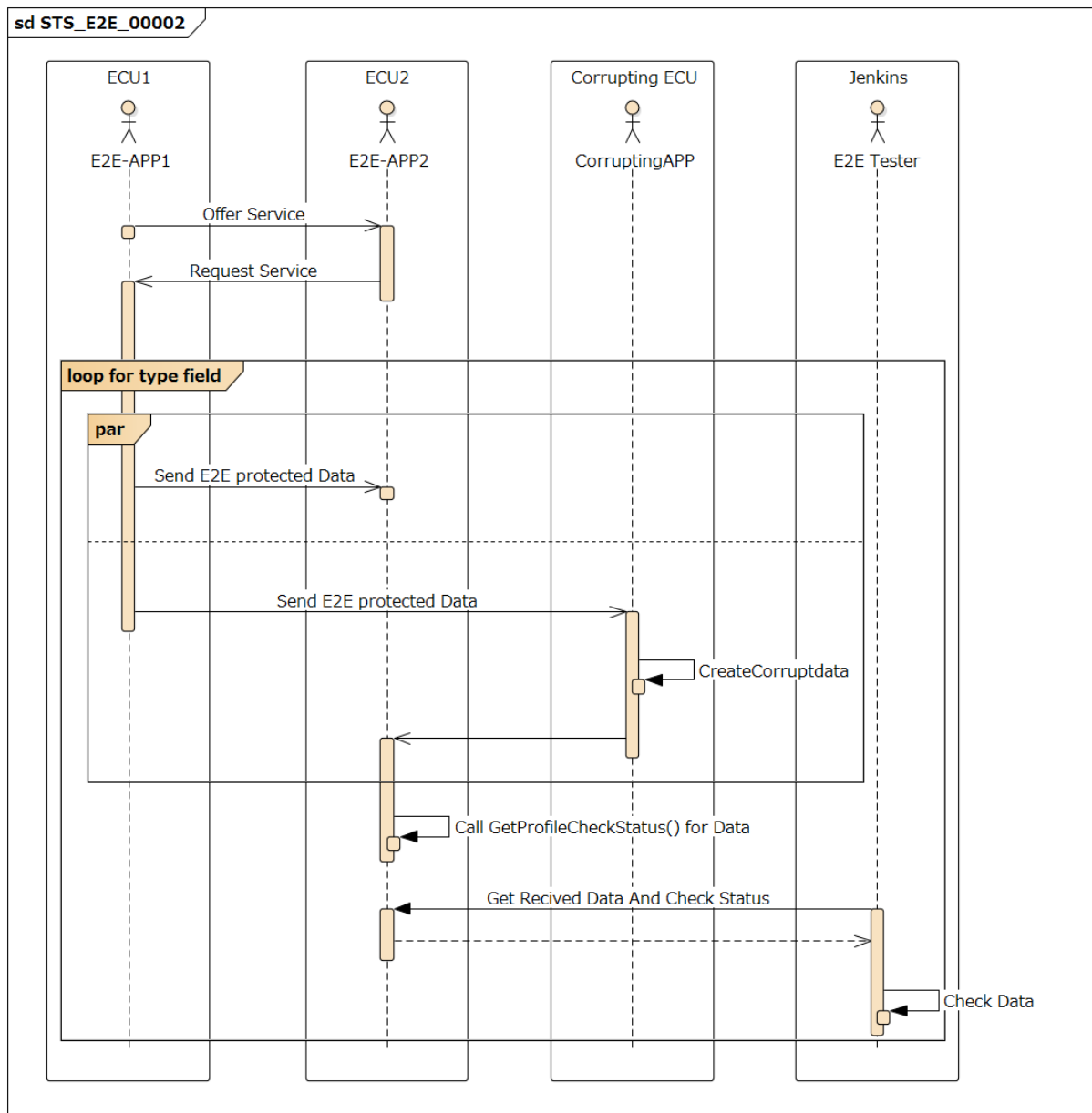
Figure 11.4: Sequence diagram of STS_E2E_00002.
