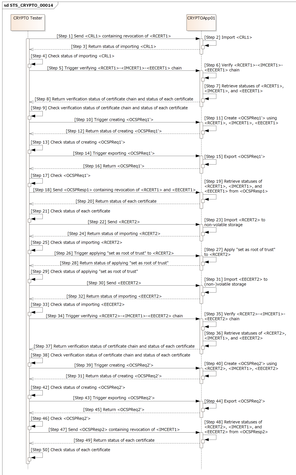
Figure 15.13: Sequence diagram of STS_CRYPT0_00014.
