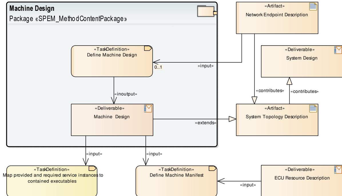
Figure 2.22: Machine Design
