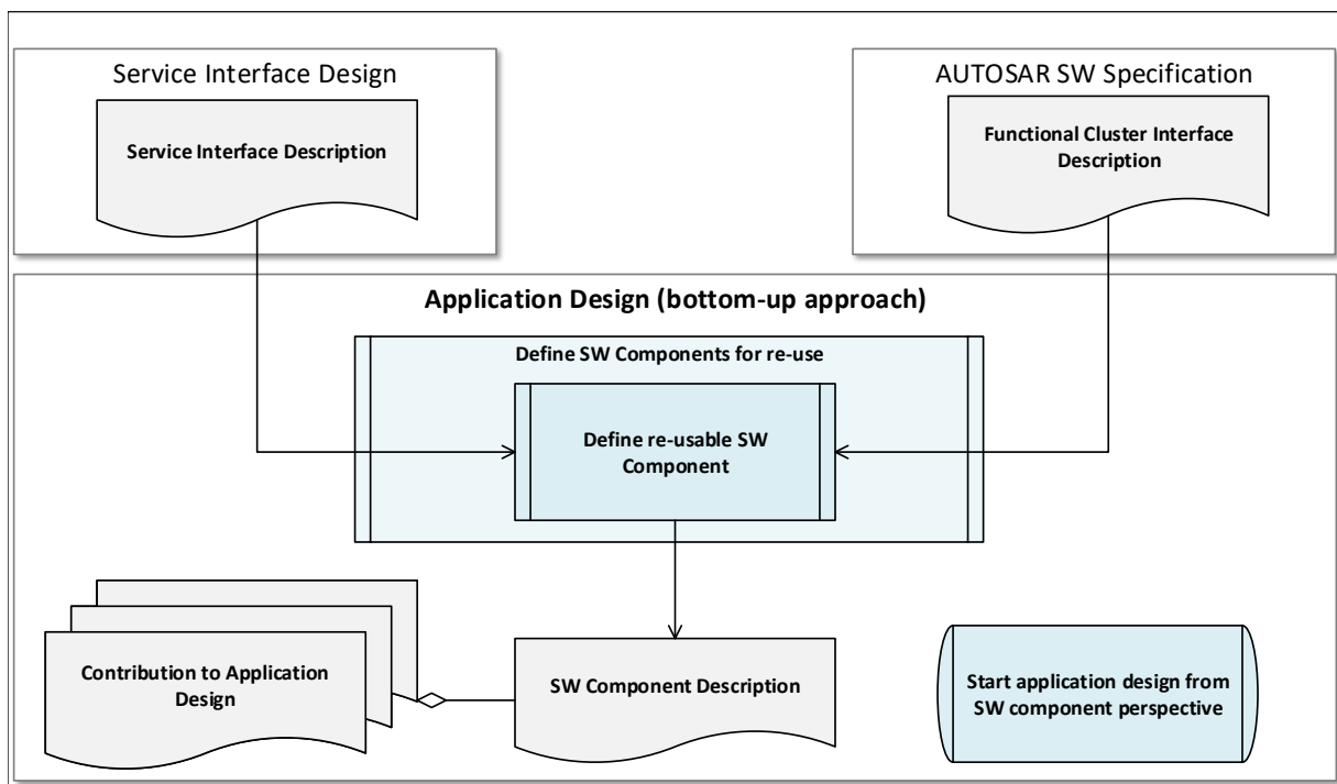
Figure 2.18: How to elaborate Application Design (bottom-up approach)
