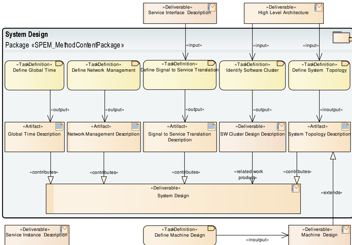
Figure 2.8: System Design
