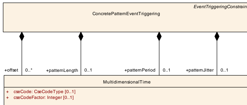
Figure 3.38: ConcretePatternEventTriggering
