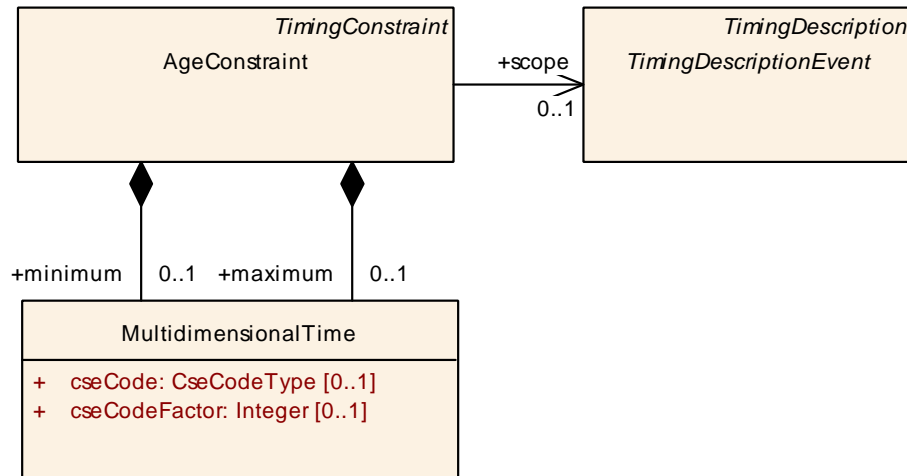
Figure 3.48: Age constraint
