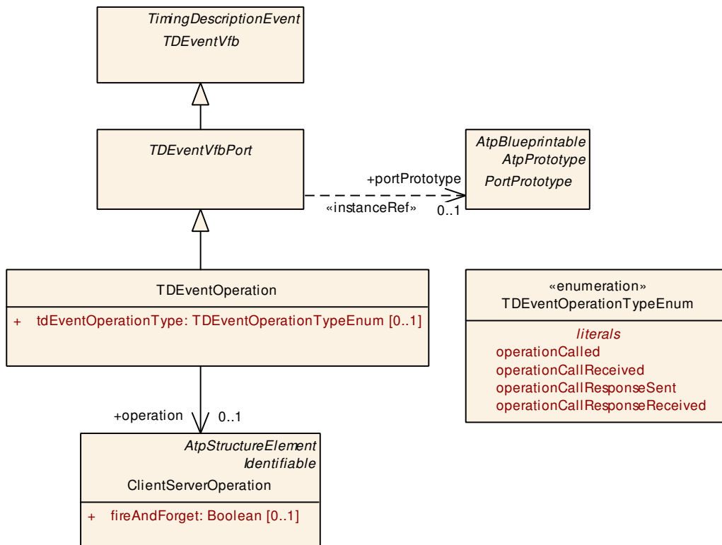
Figure 3.13: Operation
