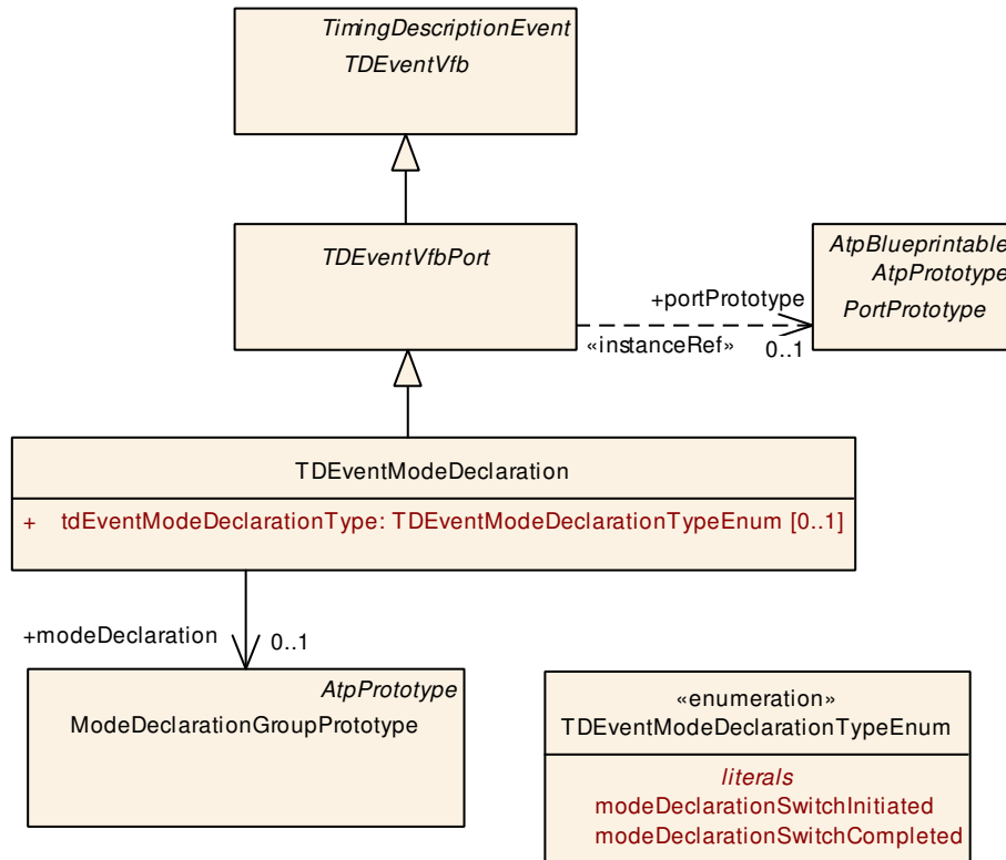
Figure 3.14: Mode Declaration
