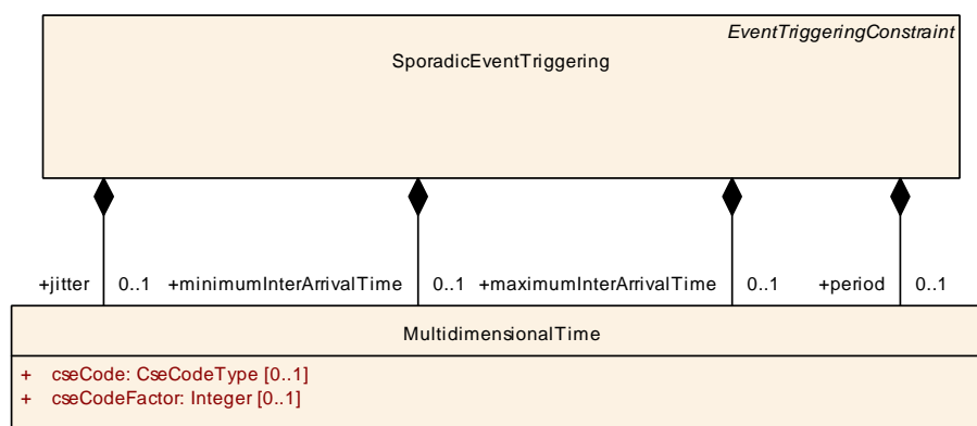
Figure 3.36: SporadicEventTriggering
