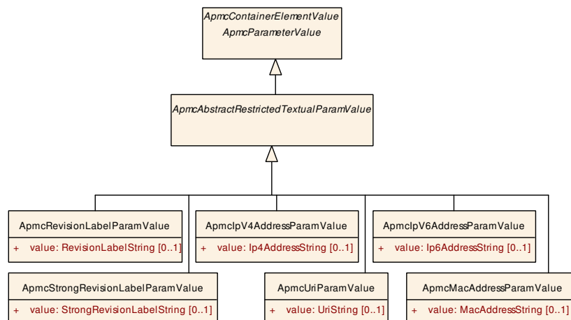
Figure 4.5: Overview of the restricted string parameter values
