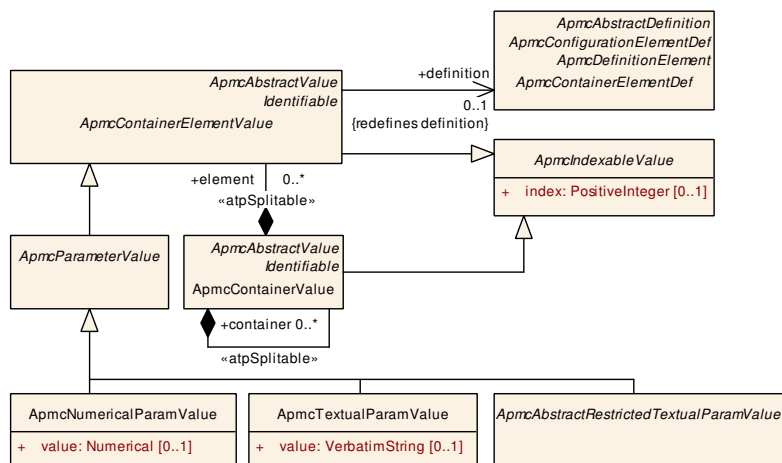
Figure 4.4: Overview of the manifest parameter values
