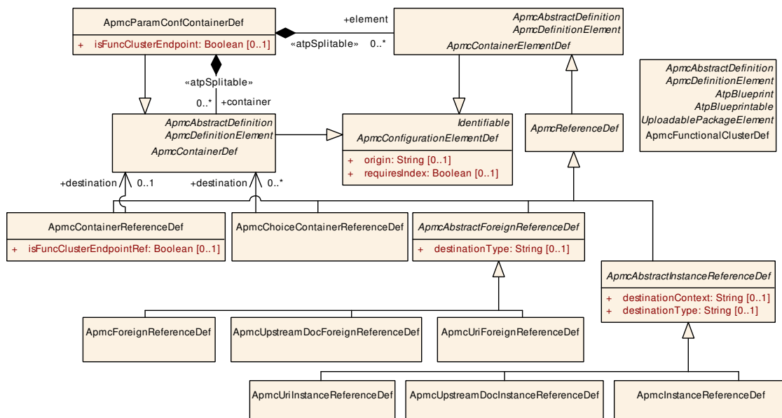
Figure 4.3: Overview of the manifest reference definition
