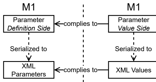
Figure 2.2: Visualization of the difference between parameter definition and parameter value
