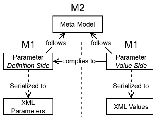
Figure 2.3: Visualization of the overall relation between meta-levels and “definition” vs. “value”
