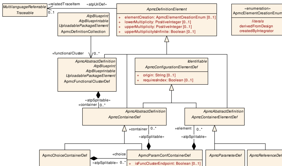
Figure 3.2: Overview of the target-configuration definition
