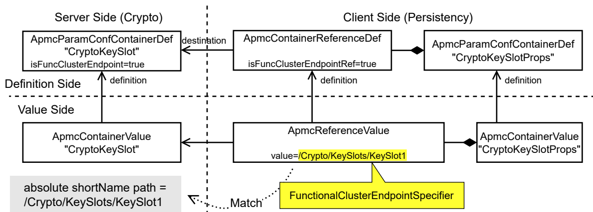
Figure 5.1: Persistence wants to encrypt storage content
