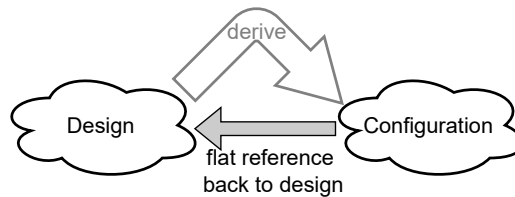
Figure 2.6: Visualization of the modeling strategy in which the configuration model is partially derived out of the design model and maintains flat references into the design model
