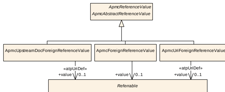
Figure 4.7: Overview of the manifest foreign reference values
