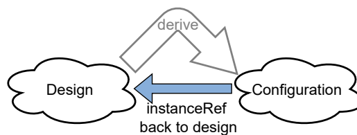
Figure 2.7: Visualization of the modeling strategy in which the configuration model is partially derived out of the design model and maintains instanceRefs into the design model
