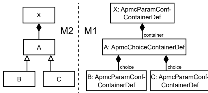
Figure 3.3: Visualization of the semantics of a choice container
