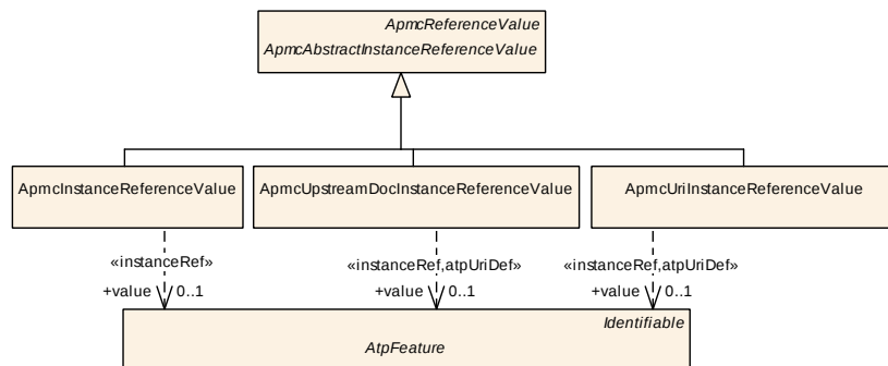
Figure 4.8: Overview of the manifest instance reference values
