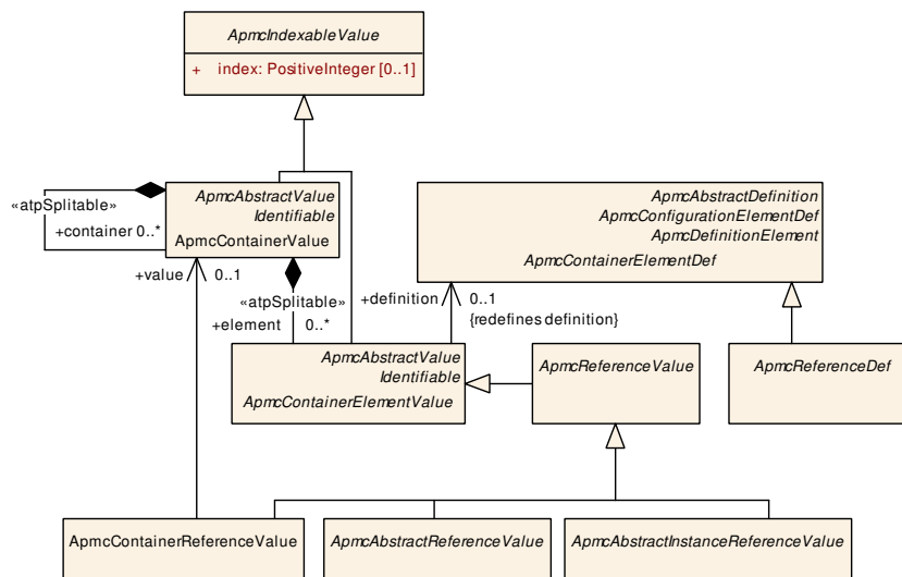
Figure 4.6: Overview of the manifest reference values
