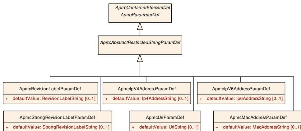
Figure 4.2: Modeling of the definition of string parameters with a content restriction
