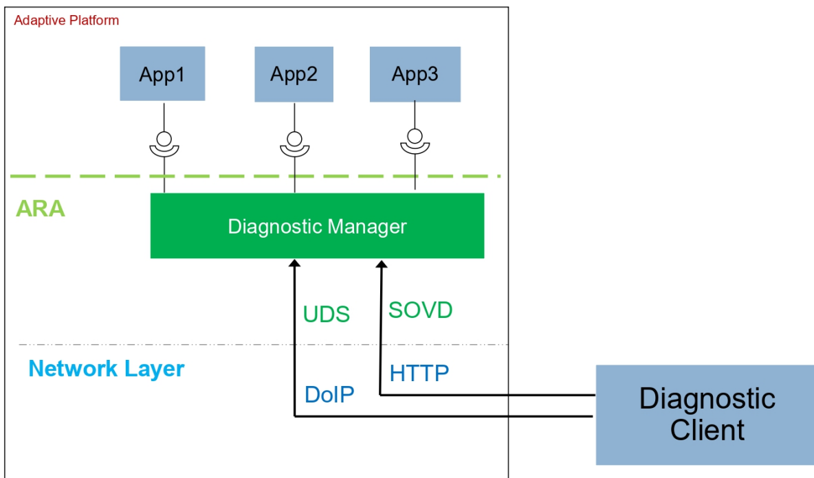
Figure 9.3: Deployment Overview of Diagnostics
