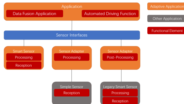
Figure 24.1: Sensor Interfaces Architecture
