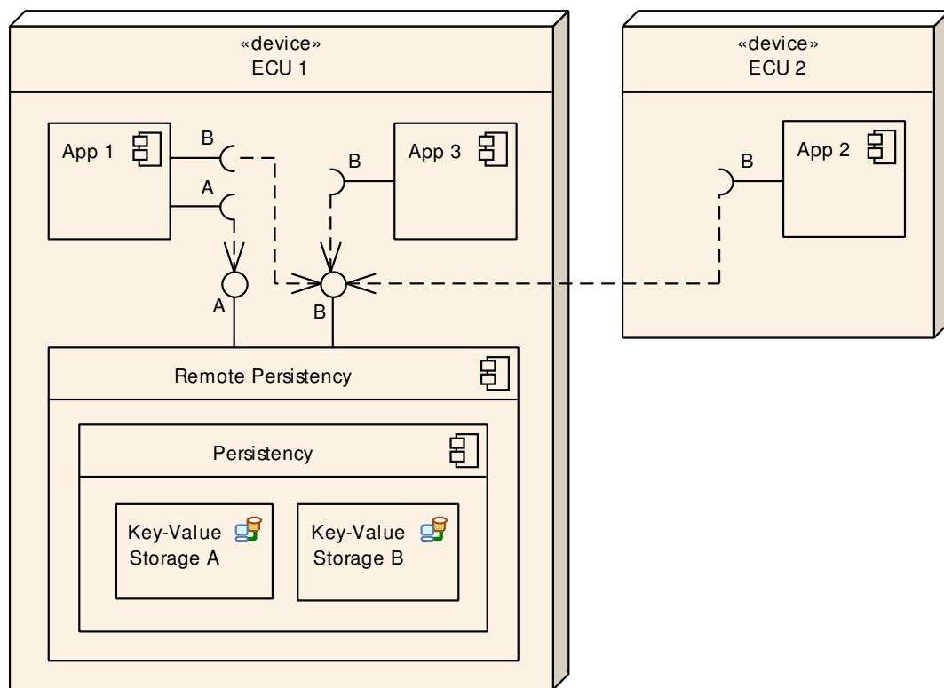
Figure 23.1: Architecture of Remote Persistence
