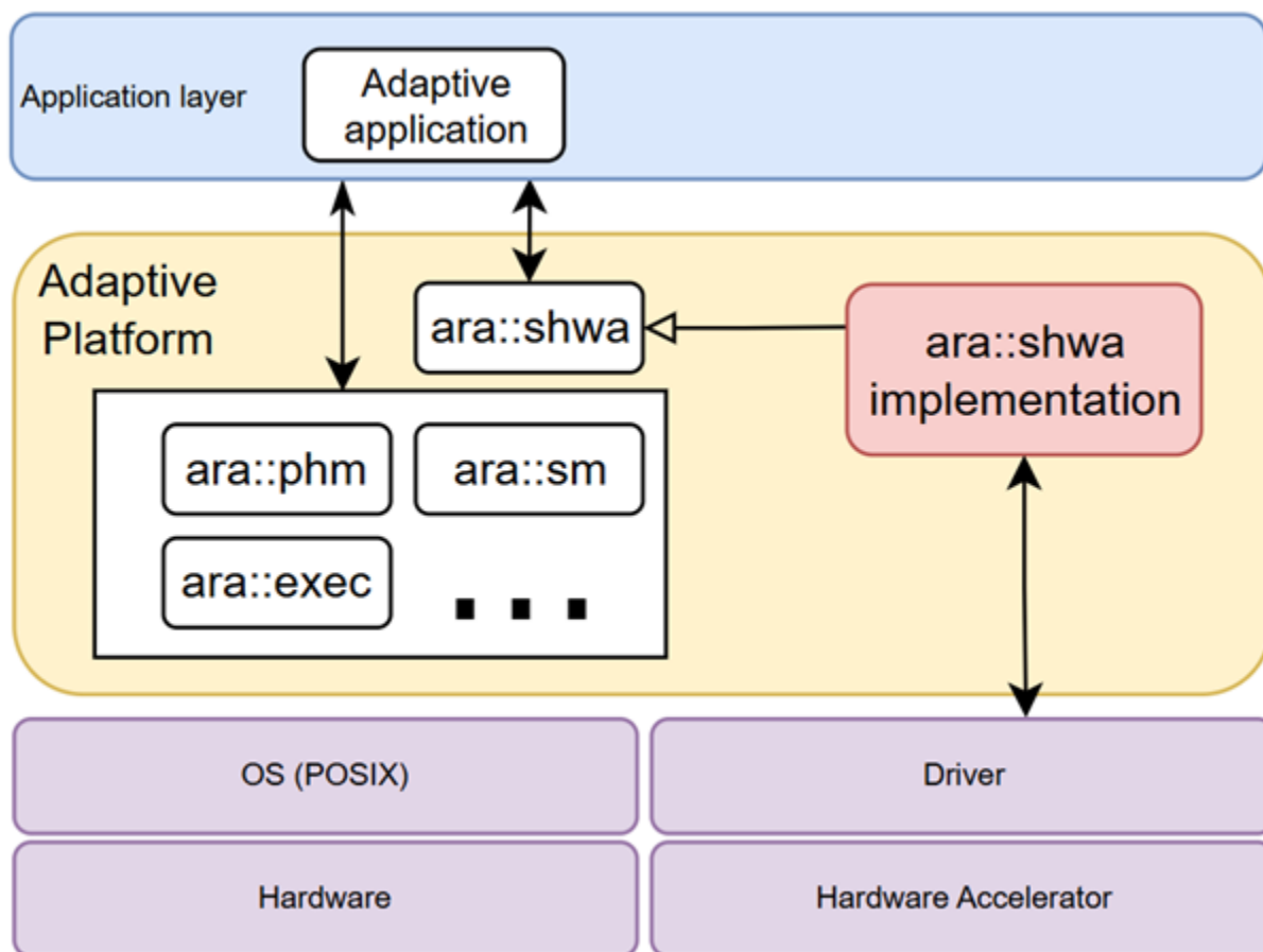
Figure 17.2: Safe Hardware Acceleration integration to AUTOSAR AP
