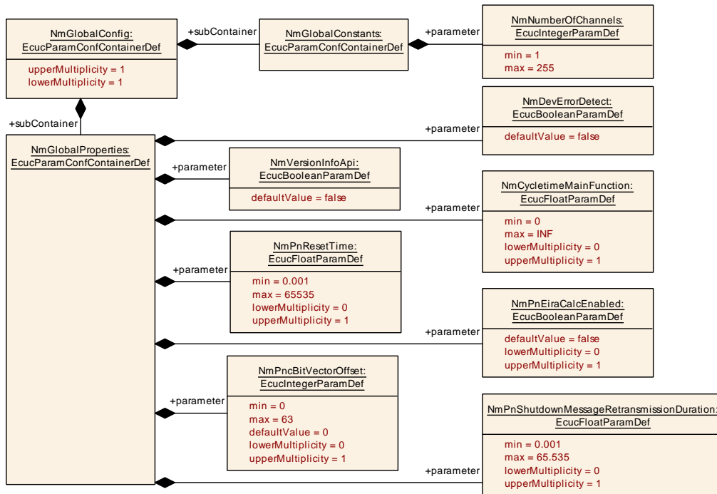
Figure 10.3: NmGlobalConfig overview
