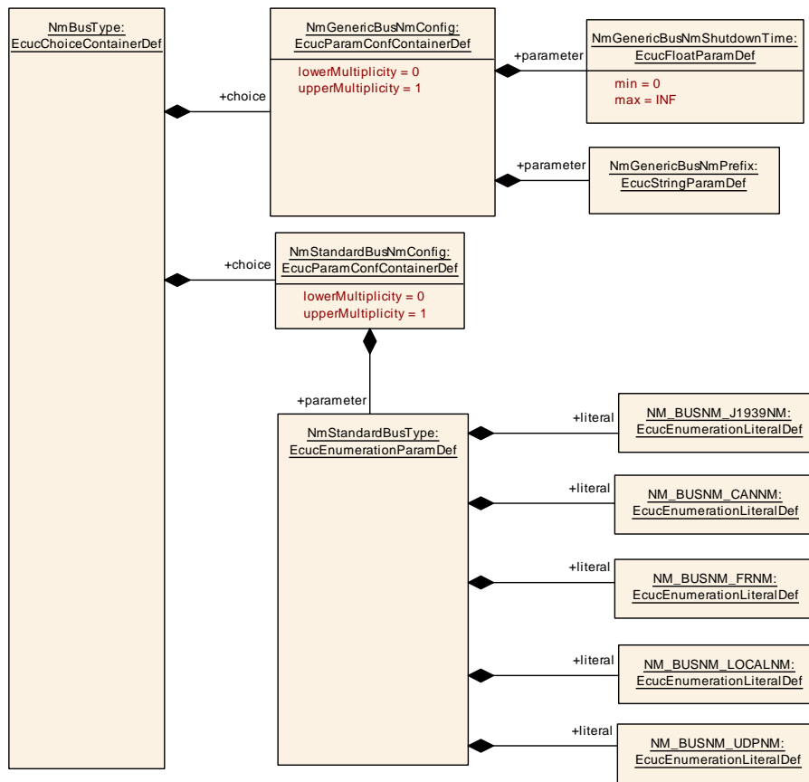
Figure 10.6: NmBusType overview
