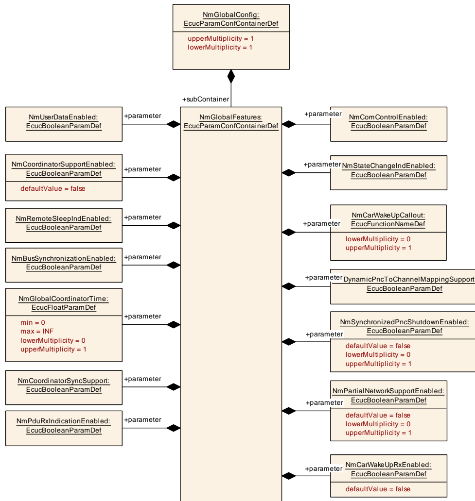
Figure 10.4: NmGlobalFeatures overview
