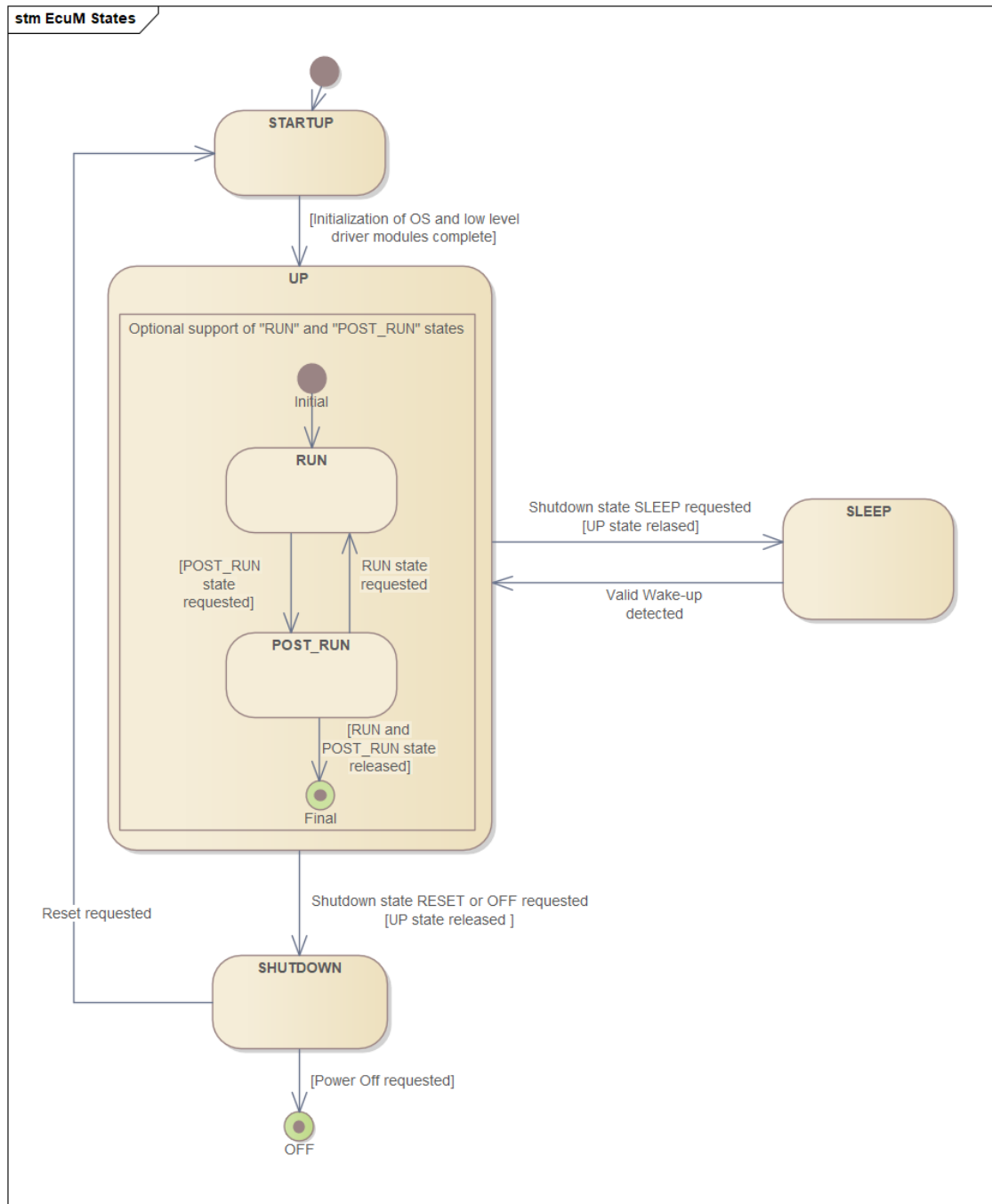
Figure 4.1: State Machine of the ECU State Management
